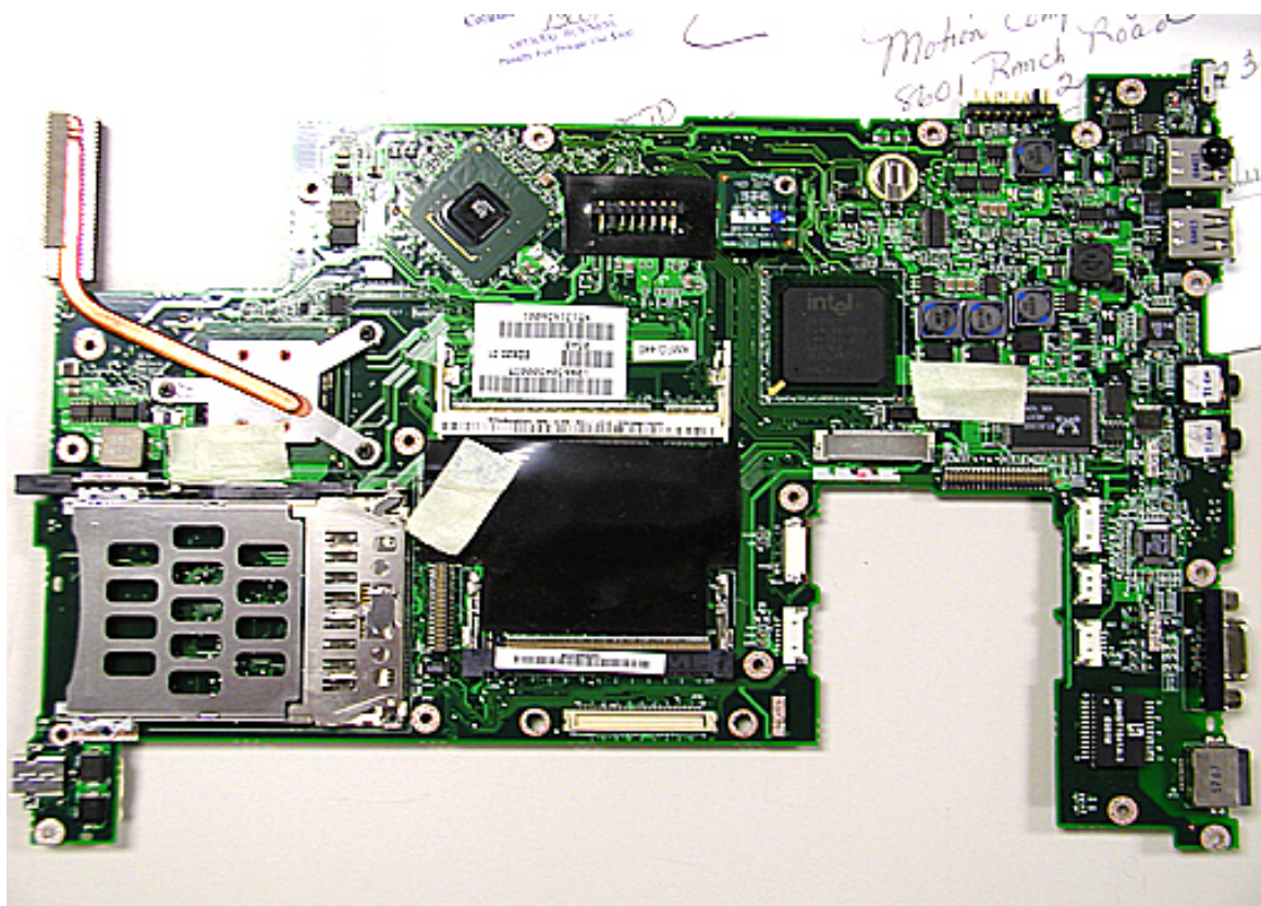
Motherboard Bottom Side
