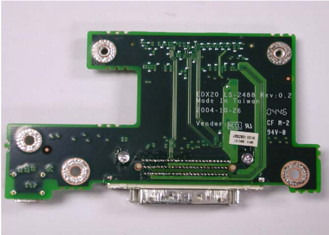
Docking Board Bottom View
