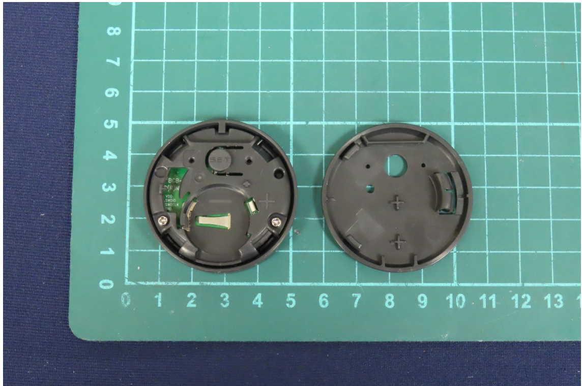
(7) EUT Photo
