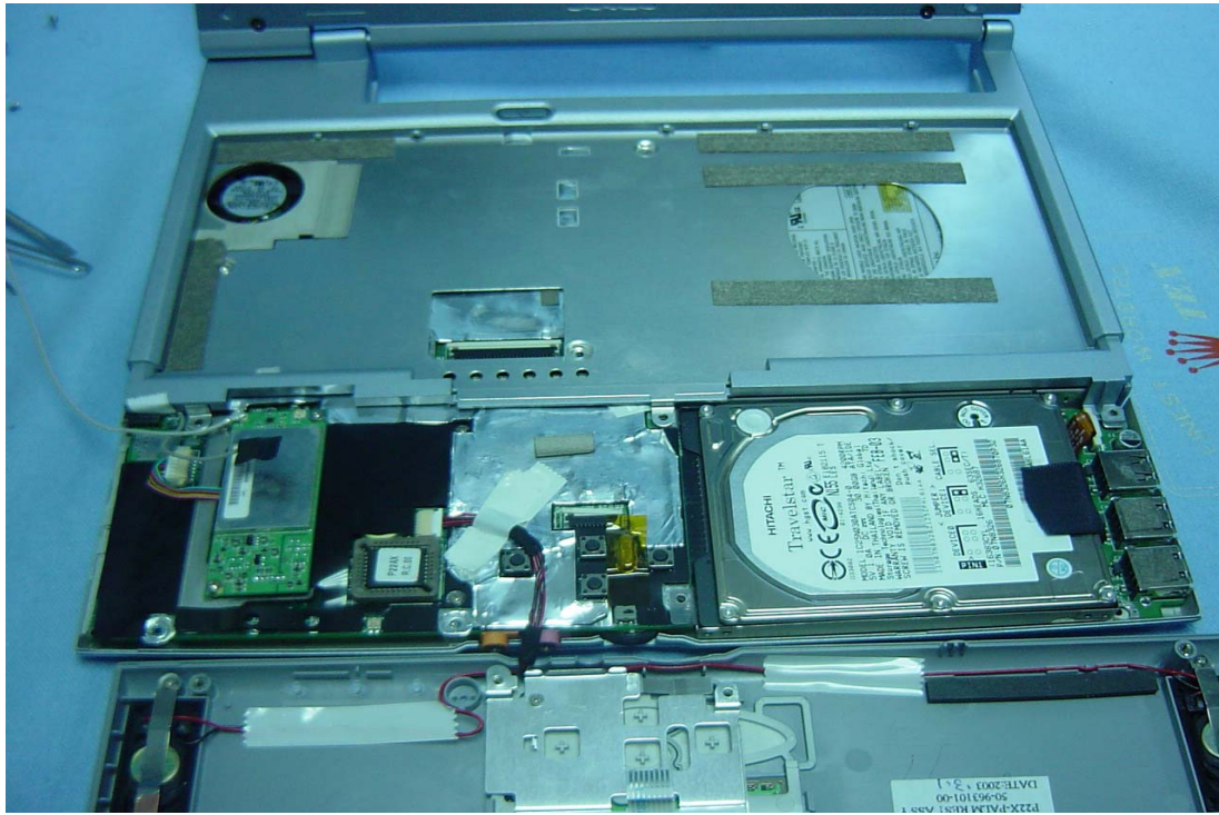
Internal of EUT --- 3
