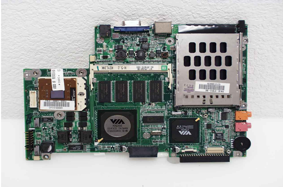
Front View of Motherboard
