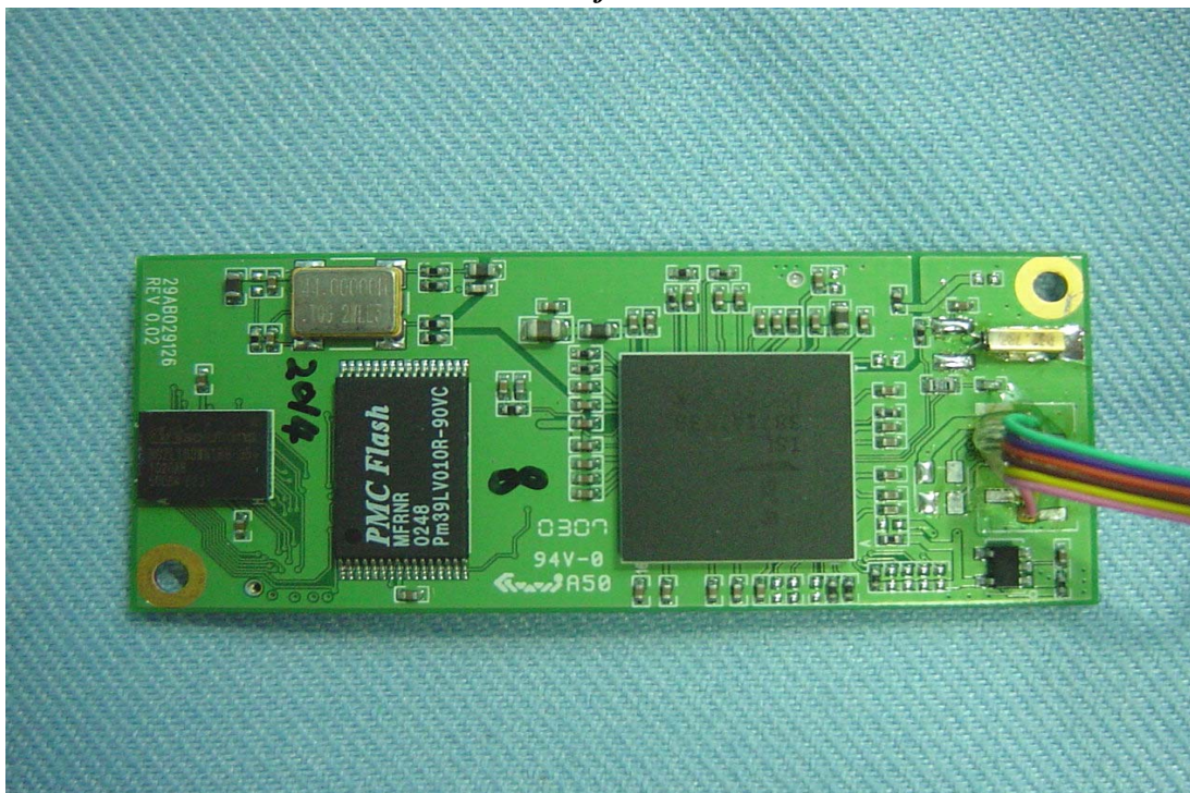
Back View of RF Module
