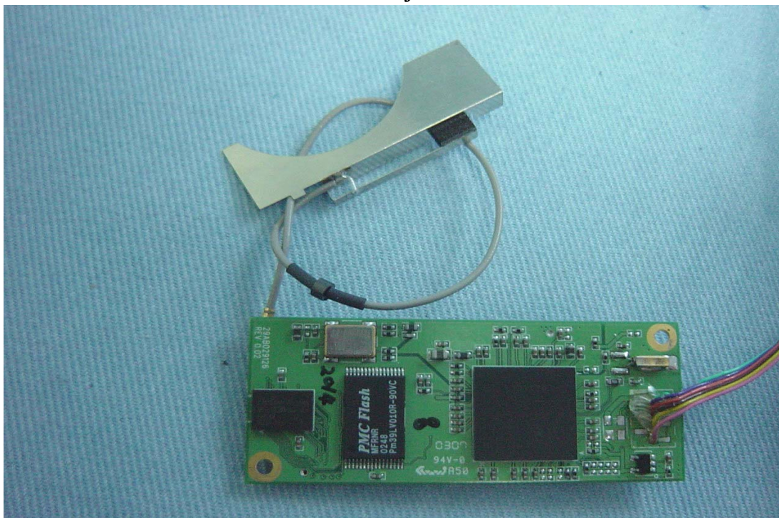
Back View of Antenna
