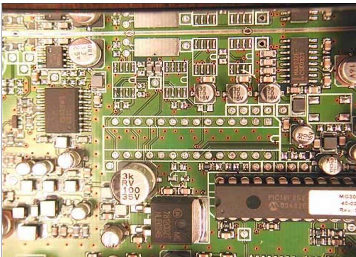
PCB 5
