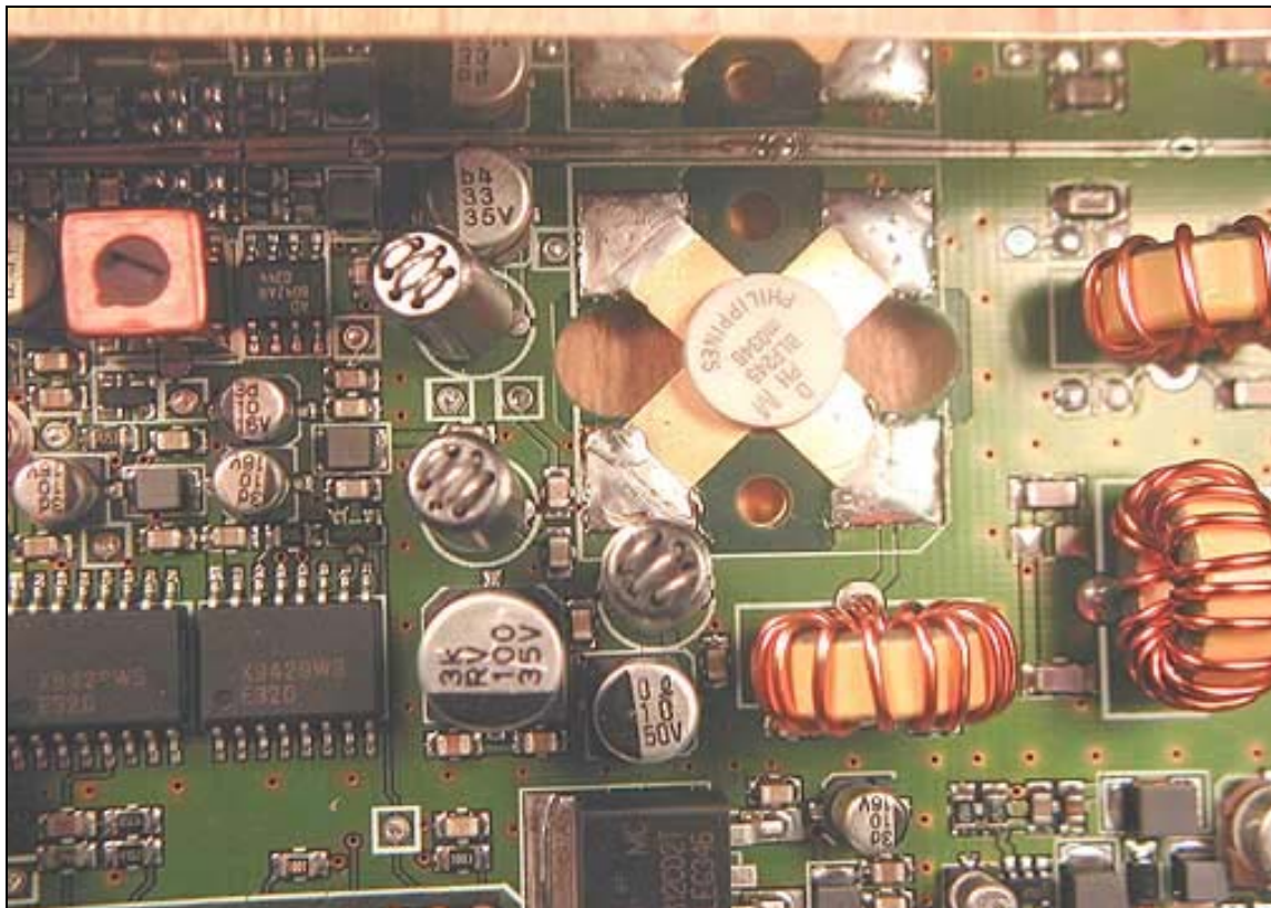
PCB 4
