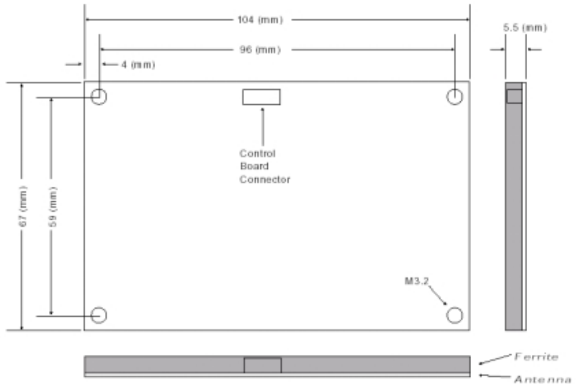
Figure 8: Antenna Dimensions
