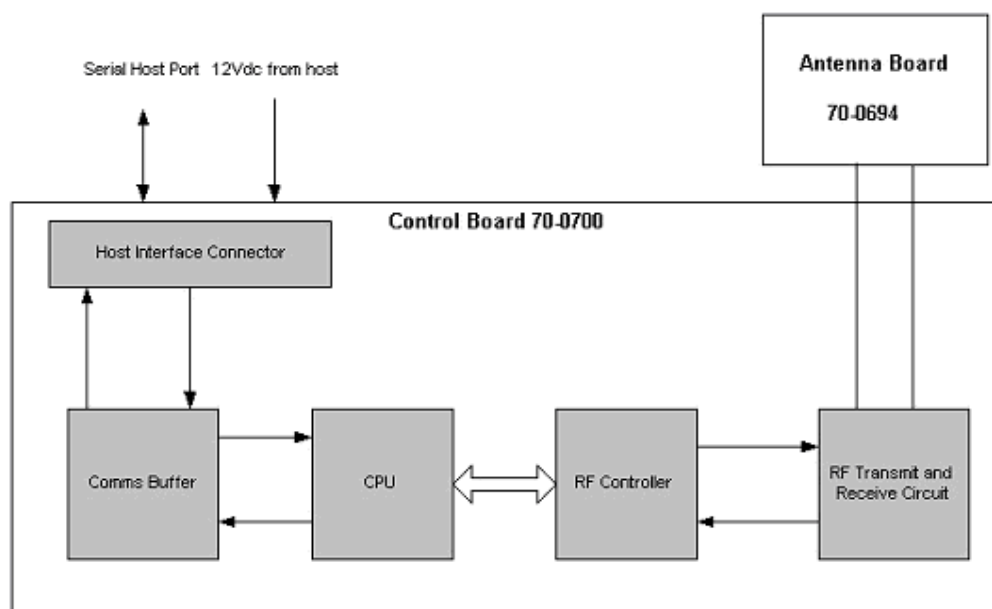
Figure 3: Module Architecture
