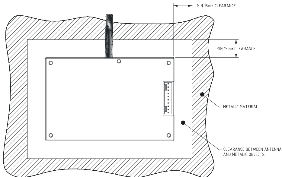
Figure 9: Clearance between antenna and metallic objects.
