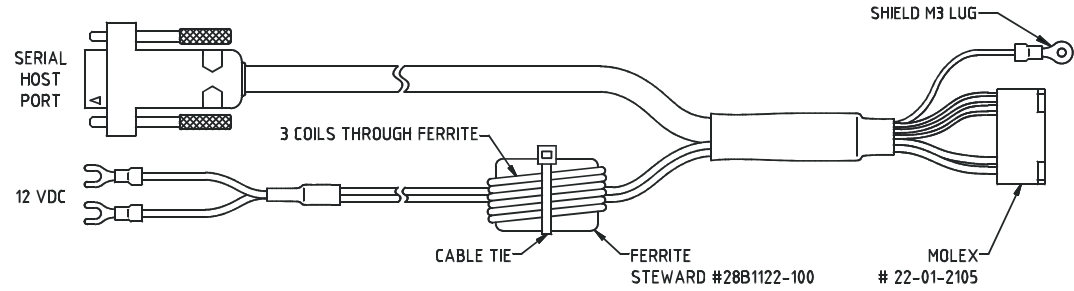
Figure 4: Interconnecting Host Cable
