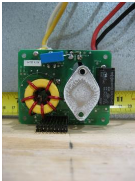
POWER SUPPLY BOTTOM SIDE
