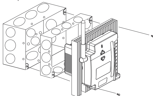
Figure 3 - Mounting Diagram
