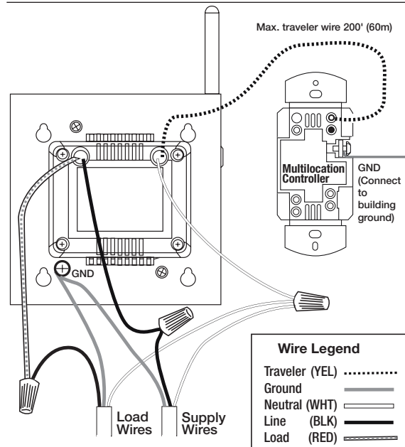
Figure 2 - Wiring Diagram
