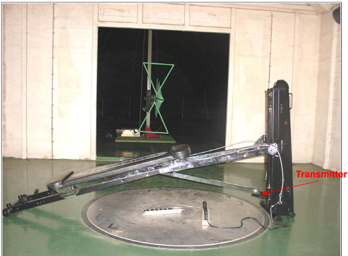
Front View
