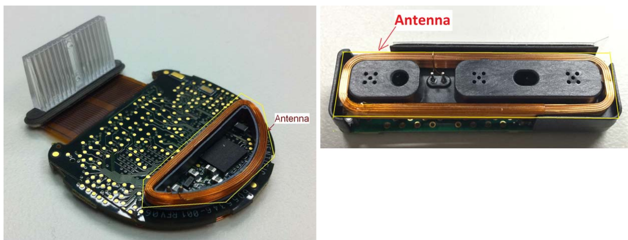
Figure 6: IPG Internal Photo, comparing SC-1132 (on the left) to SC-1140/DB-1140 (on the right)
