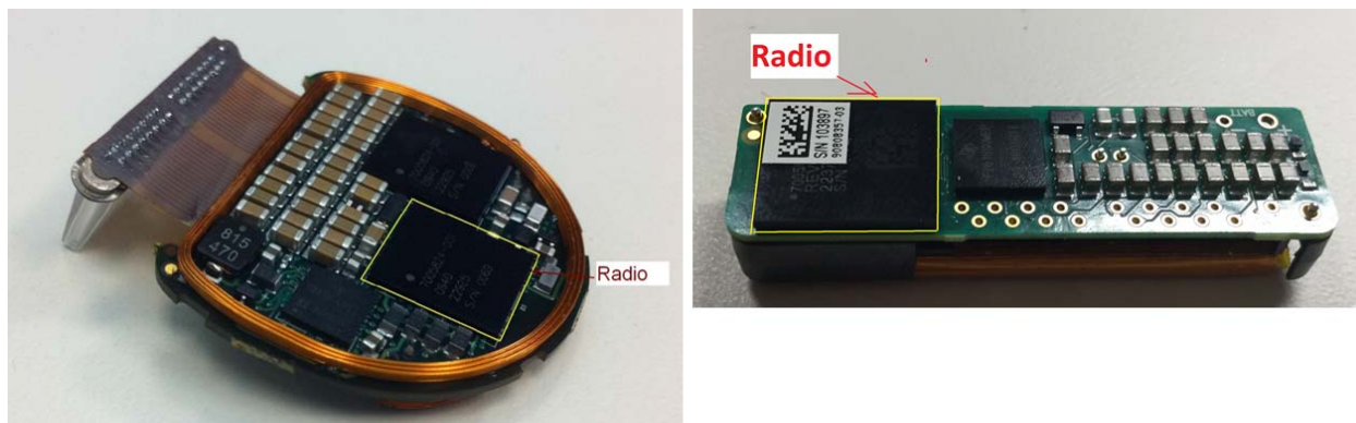
Figure 5: IPG Internal Photo, comparing SC-1132 (on the left) to SC-1140/DB-1140 (on the right)
