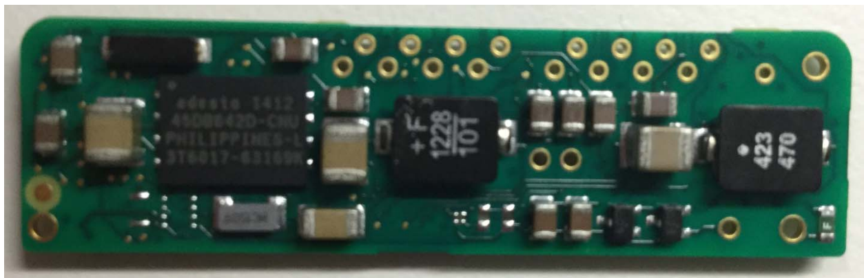
Figure 4: IPG PCBA Photo
