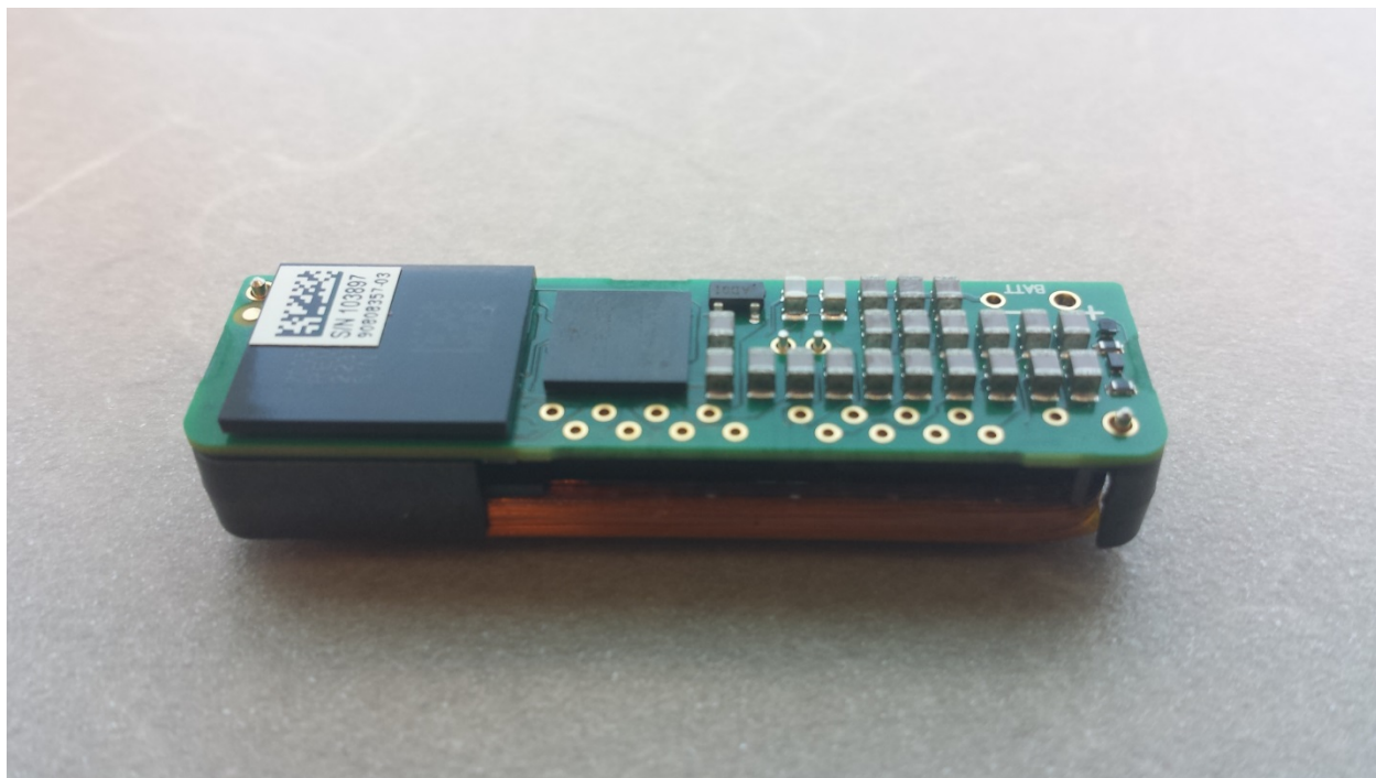
Figure 2: IPG Internal Photo
