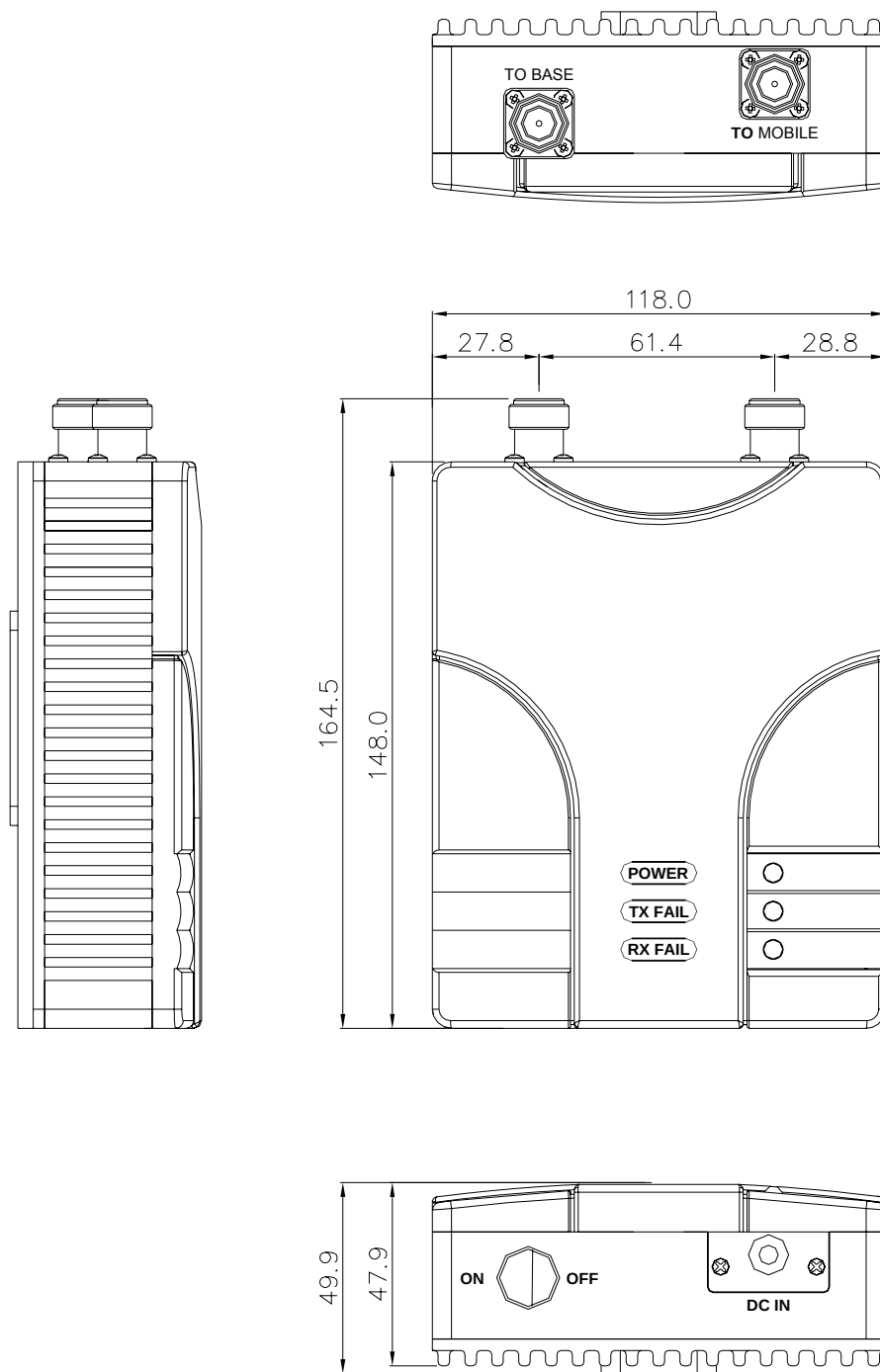
<Figure 2-7: USHR-1900H Connectors>
