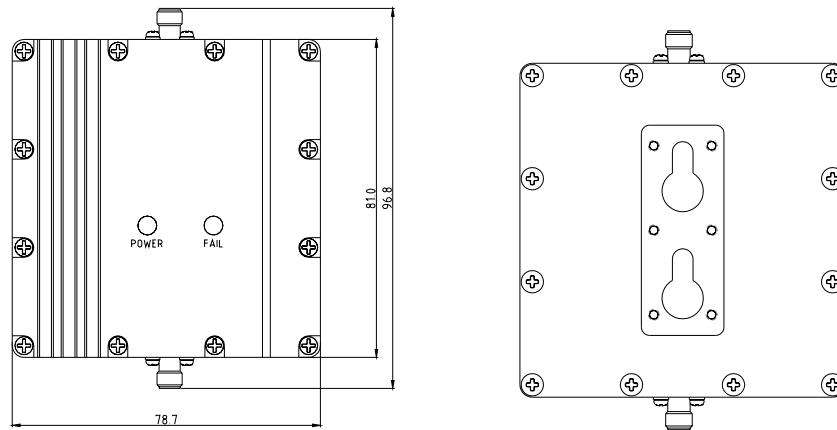
<Figure 5-1: USHR-800 Front and Back views>
