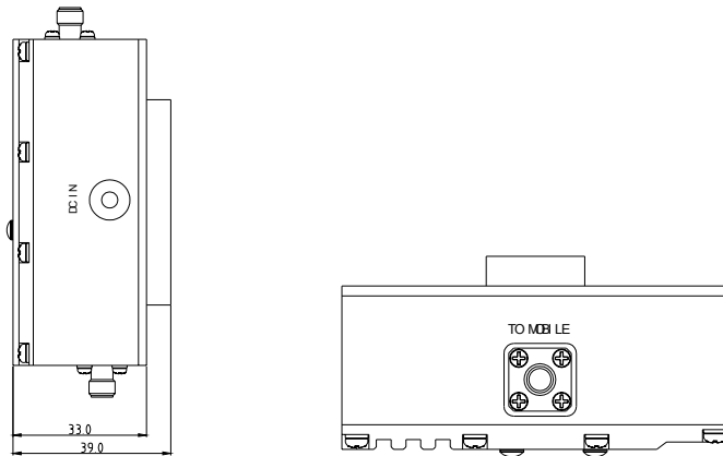
< Figure 2-7: USHR-800 Connectors >
