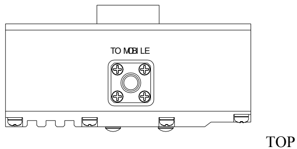
<Figure 5-2: USHR-800 Top and Bottom views>
