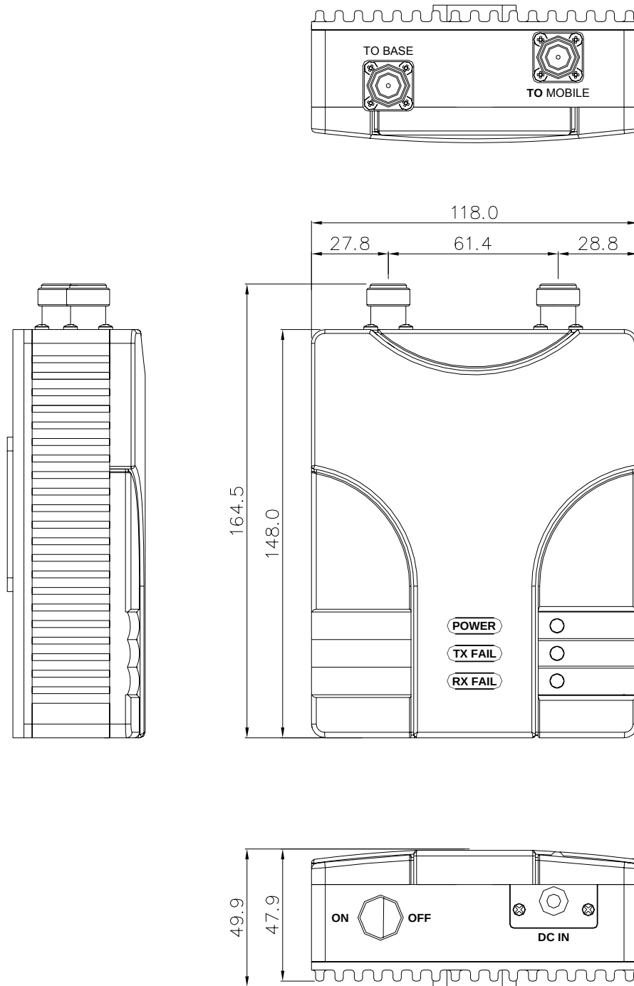
<Figure 2-7: USHR-800H Connectors>
