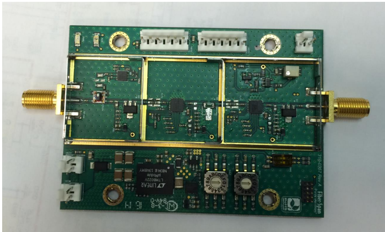
LNA Board
