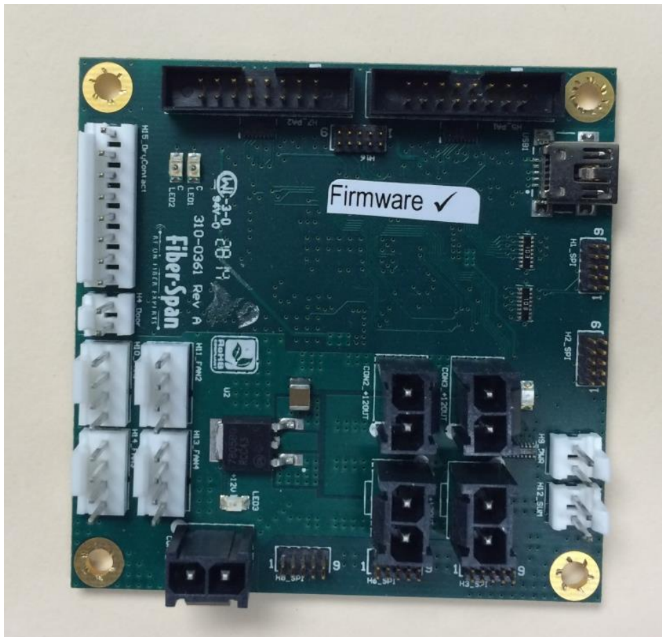
Control Board
