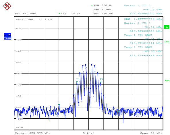
Figure 8.4-2: 823.975 MHz output
