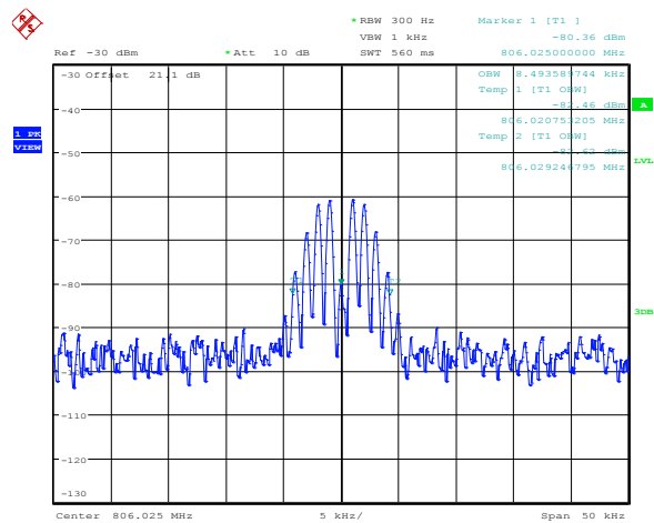
Figure 8.4-1: 806.025 MHz output
