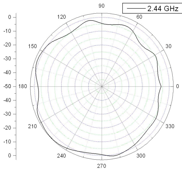
Elevation Pattern
