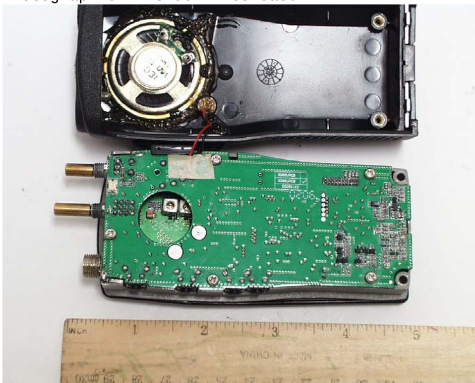
Photograph of inside MT16U case.
