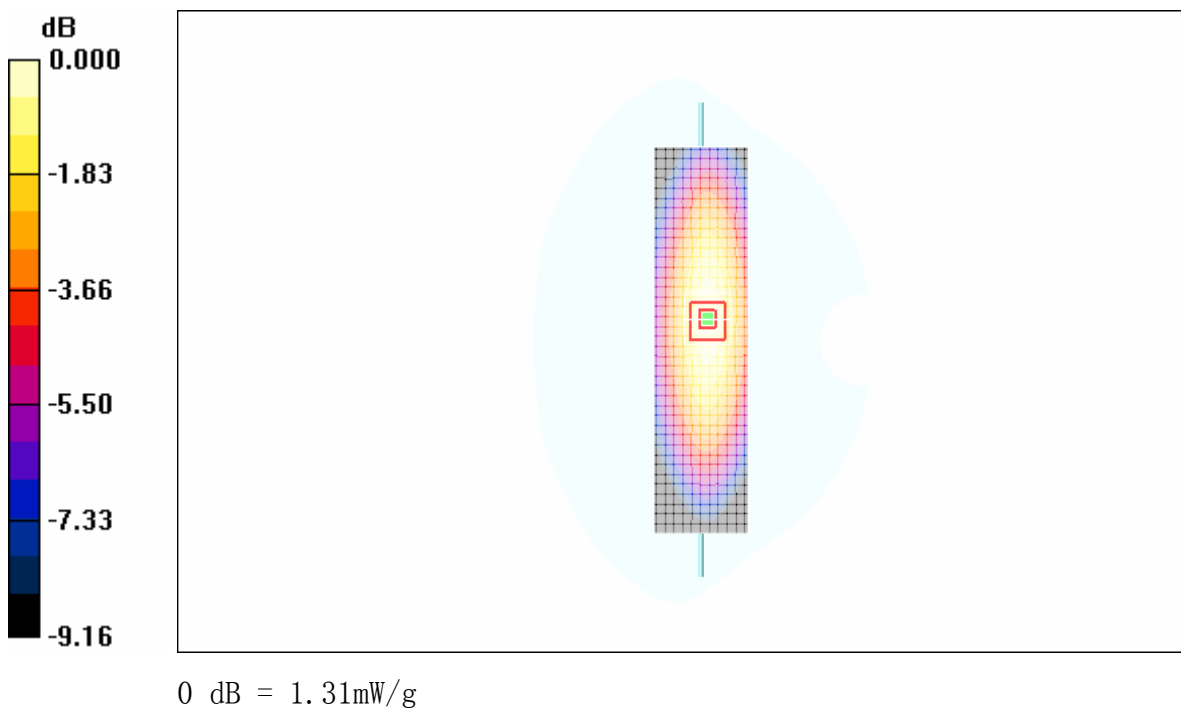
Fig.25 validation 450MHz 250mW
