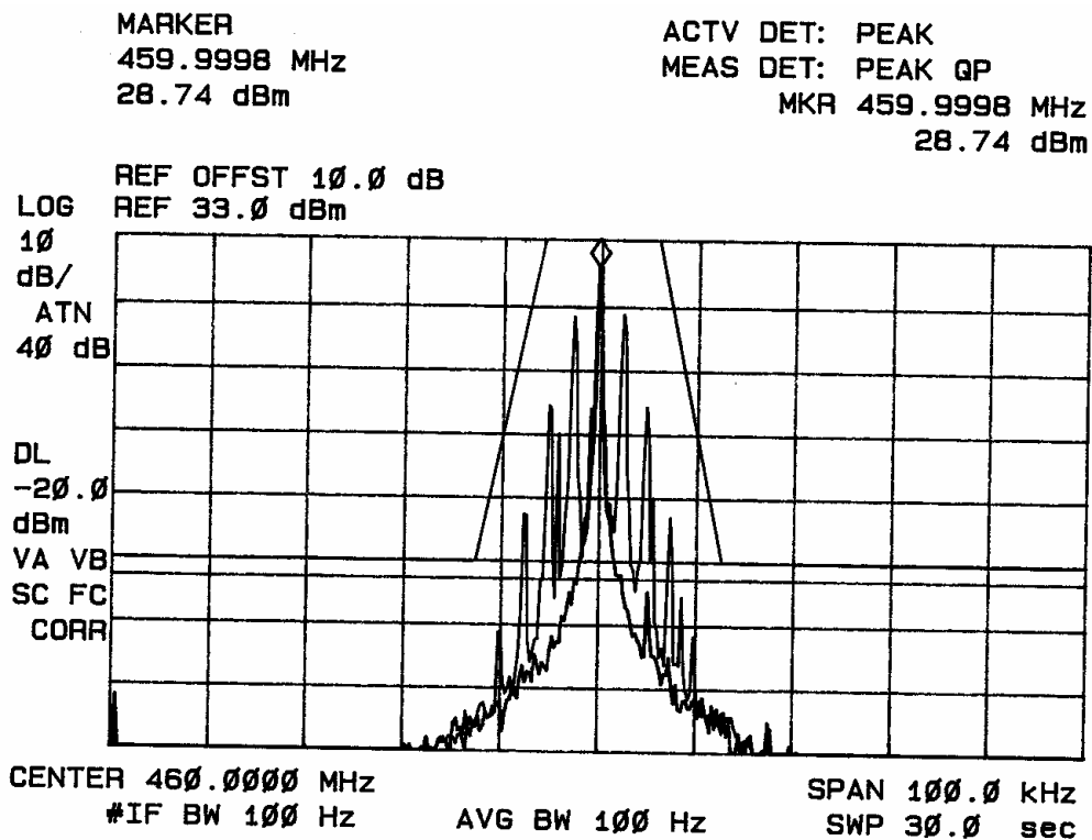
Figure 5: Occupied Band Width, with no tone squelch (2W)
