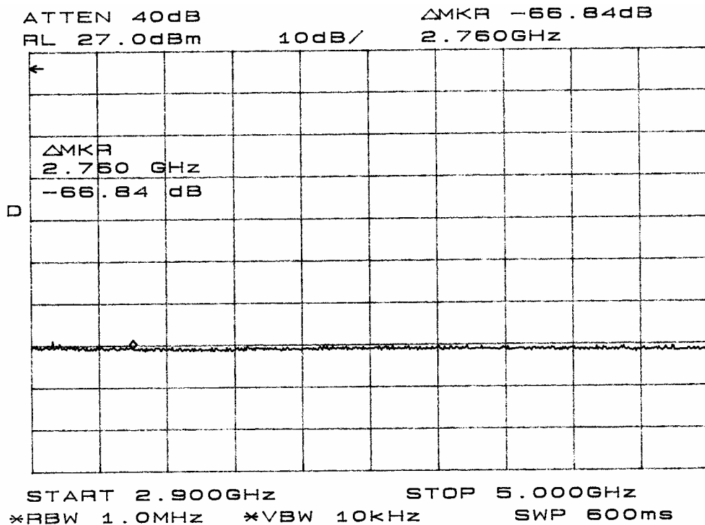
Figure 9: Emissions at Antenna Terminal (0.5W)
