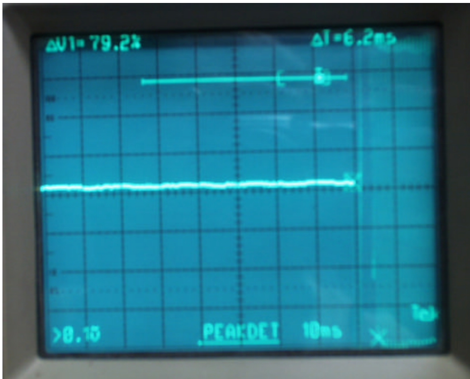
Figure 14 Transient Behavior of Transmitter t3
