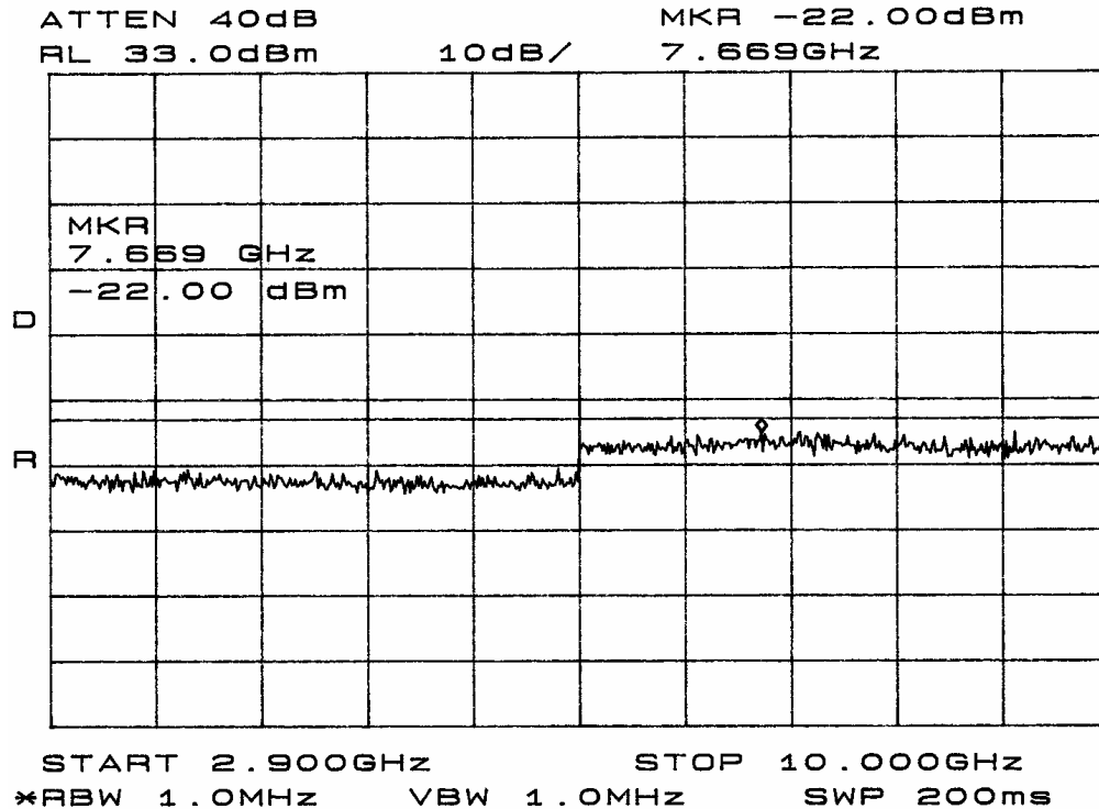
Figure 12: Emissions at Antenna Terminal (2W)
