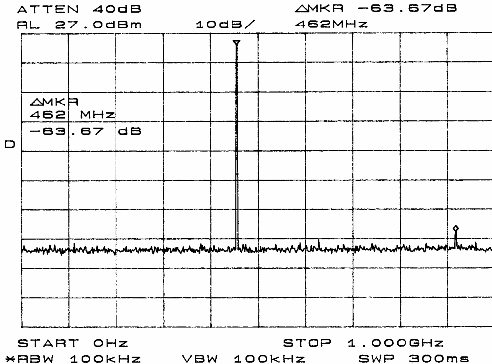
Figure 7: Emissions at Antenna Terminal (0.5W)
