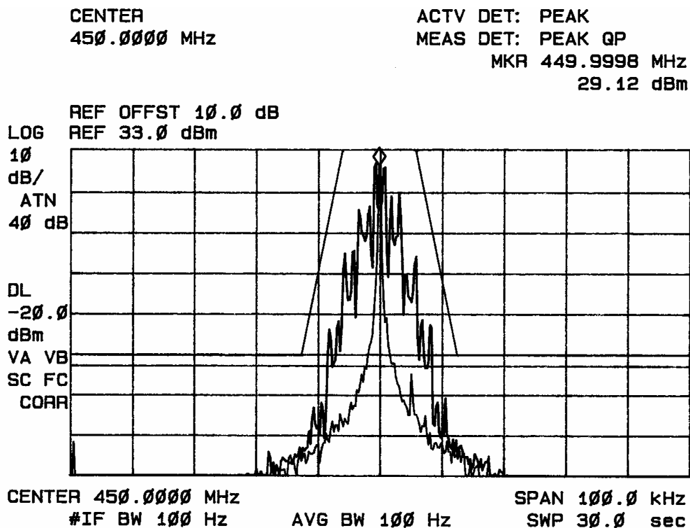
Figure 6: Occupied Band Width, with DCS tone squelch (2W)
