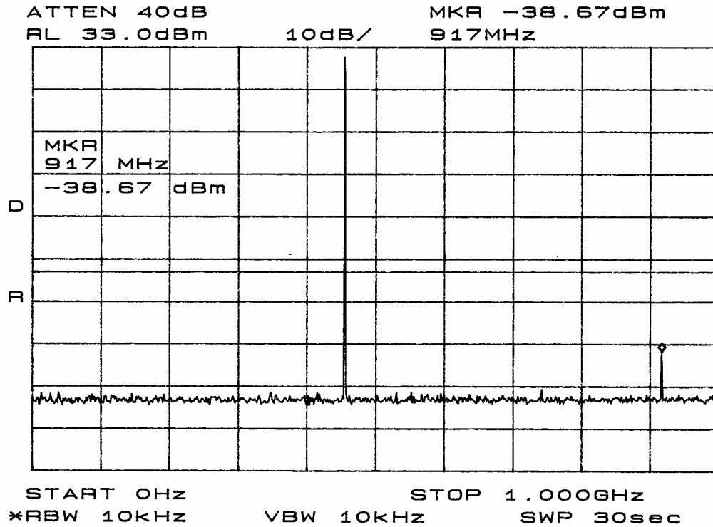
Figure 10: Emissions at Antenna Terminal (2W)
