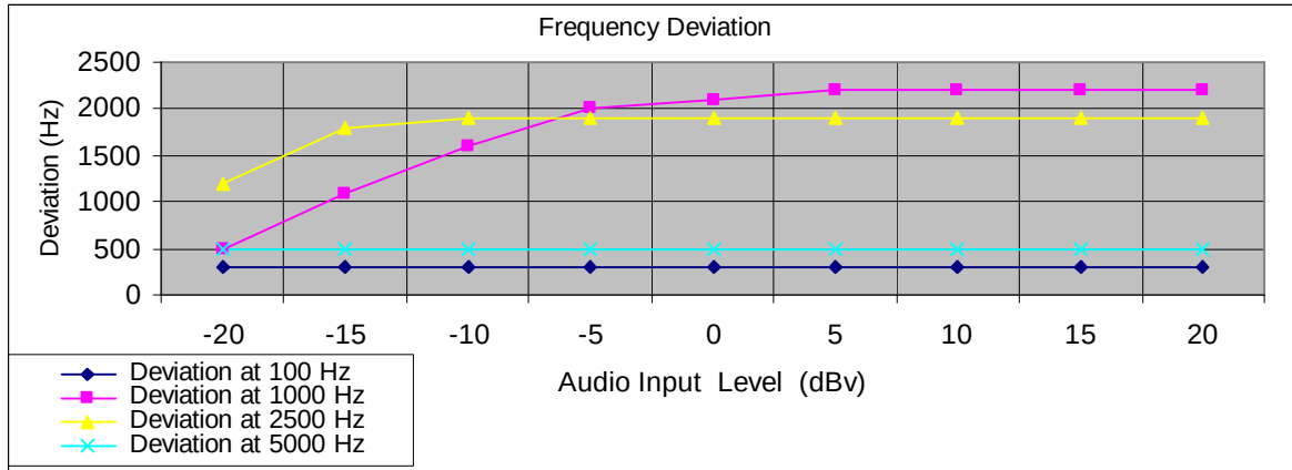
Figure 2 Deviation Characteristics.
