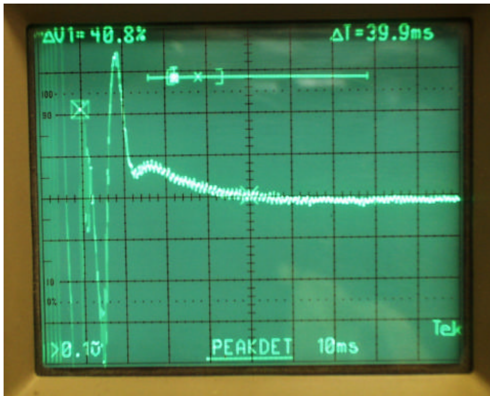
Figure 13 Transient Behavior of Transmitter t1
