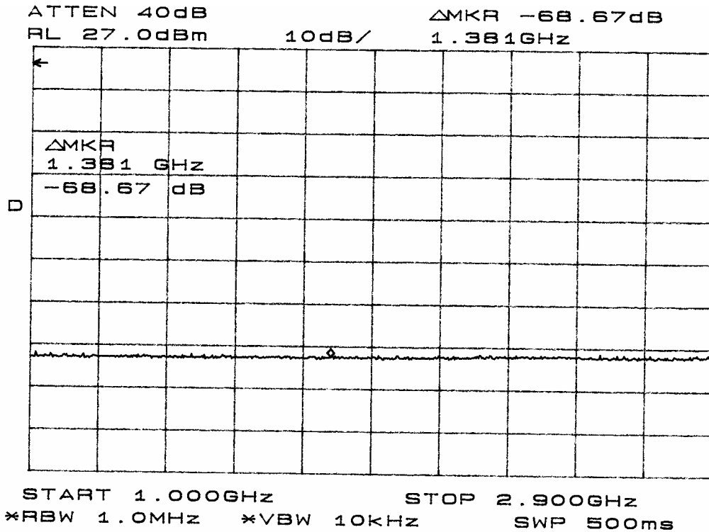
Figure 8: Emissions at Antenna Terminal (0.5W)
