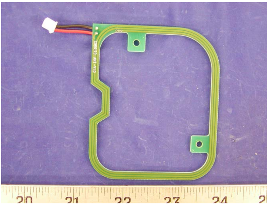
Antenna View
