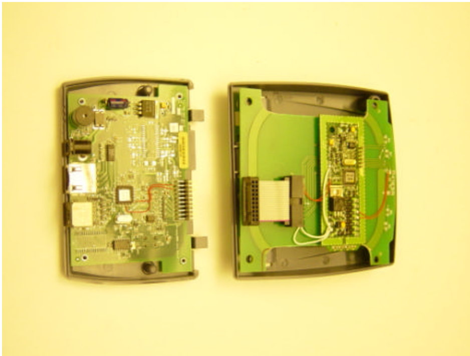
EUT – Cover Off View I
