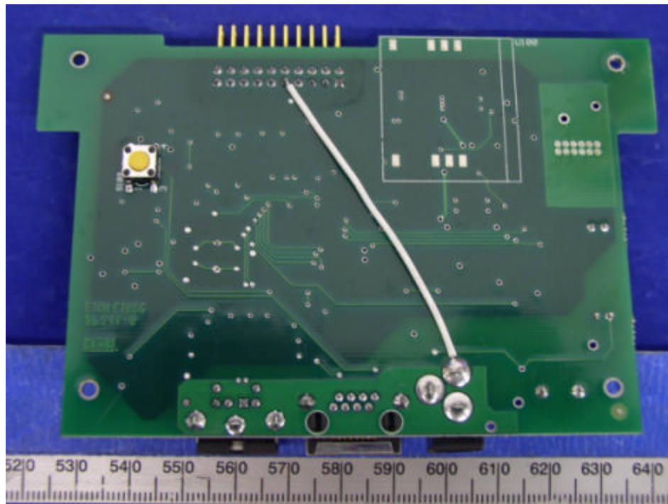
EUT – Solder View II
