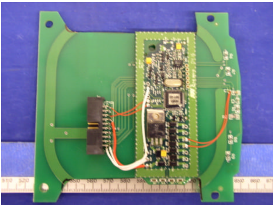
EUT – Component View I
