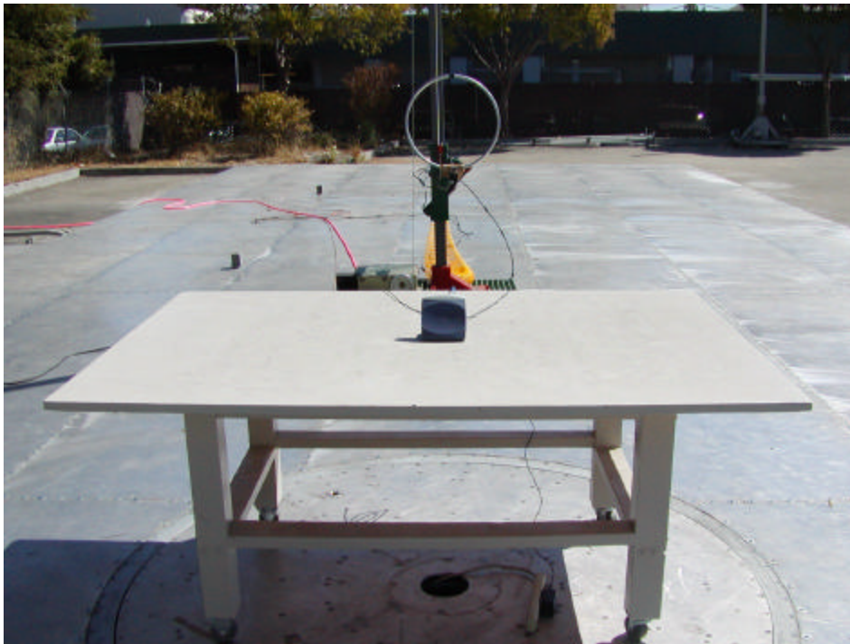
Radiated Emission – Front View
