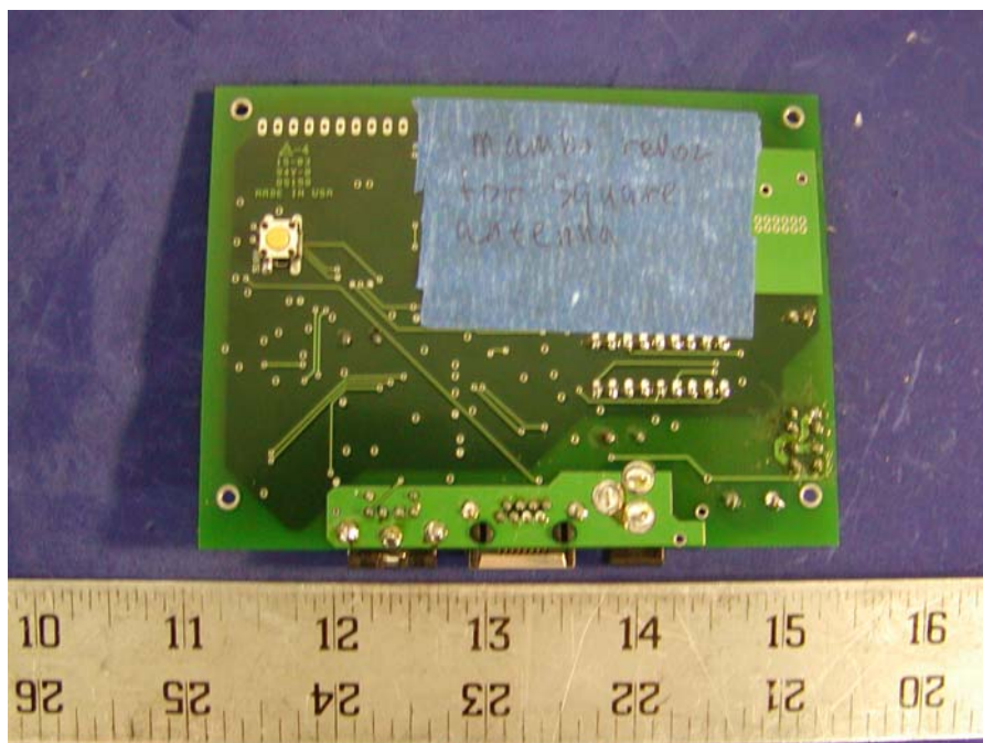
Transceiver Board Solder View 1
