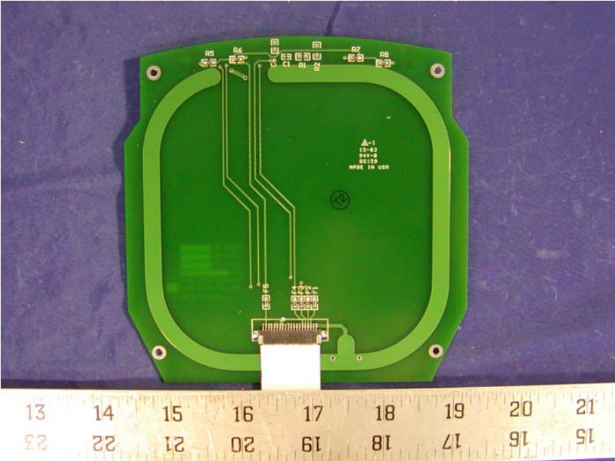
300-1018 Antenna Rear View
