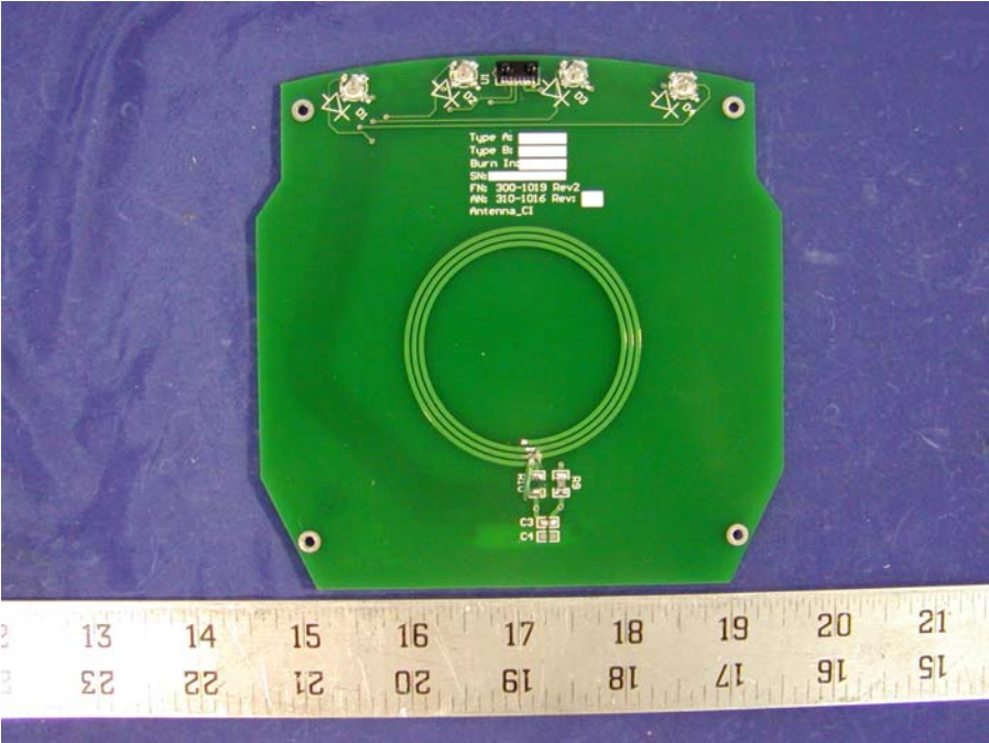
300-1019 Antenna Front View
