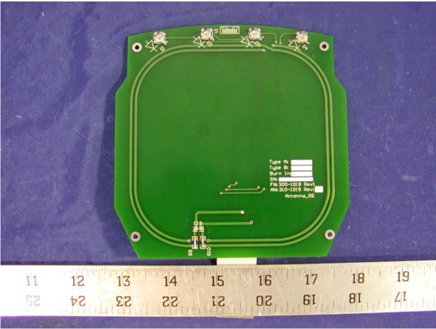
300-1018 Antenna Front View
