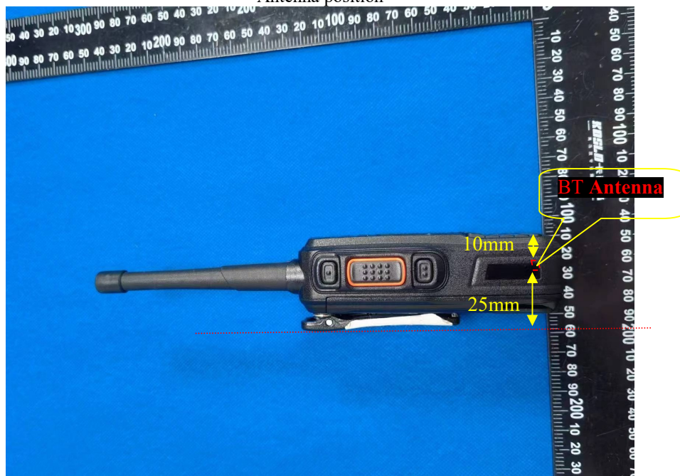
Antenna position
