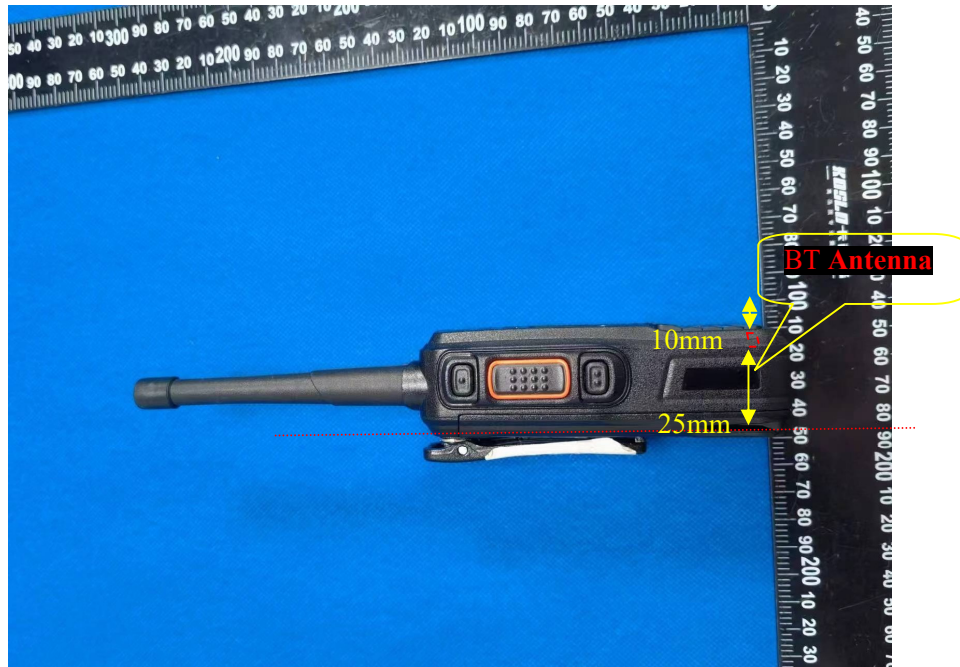
Antenna position
