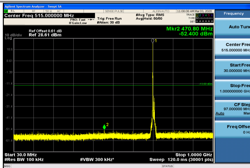
Band12-10MHz-QPSK-23130-1RB#0-30~1000MHz
