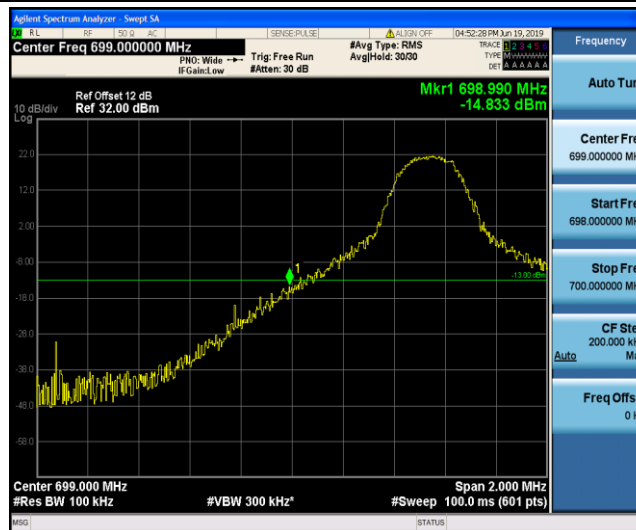
Band12_5MHz_23035_1RB#0
