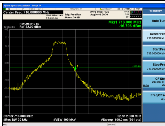
Band12_3MHz_16QAM_23165_1RB#14
