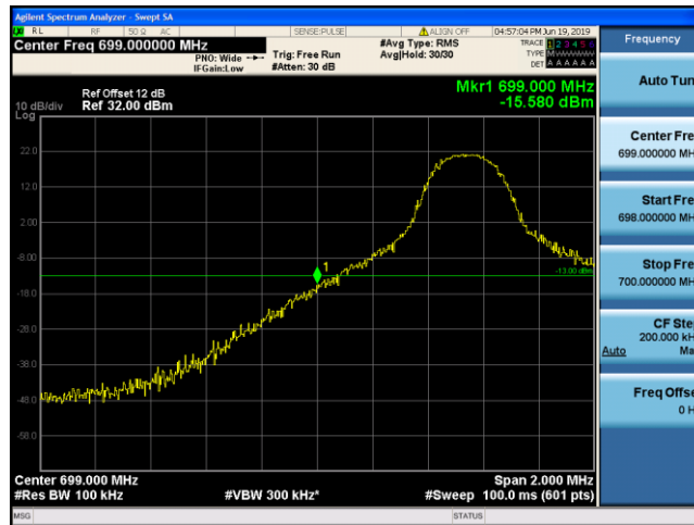
Band12_5MHz_QPSK_23035_1RB#0
