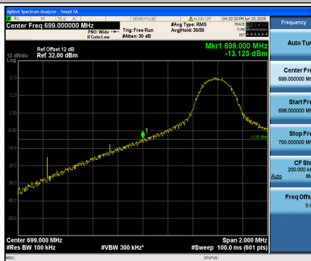
Band12_10MHz_QPSK_23060_1RB#0
