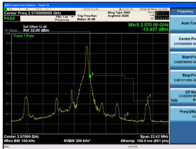
Band7_5MHz_QPSK_21425_1RB#24
