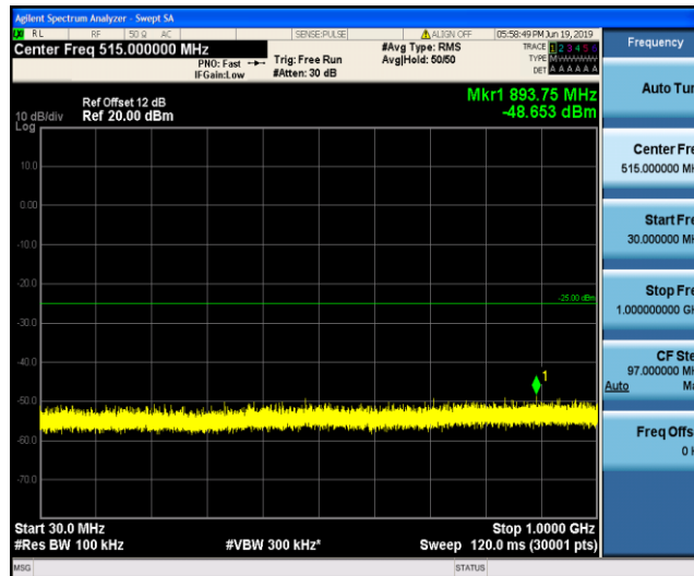
Band41_5MHz_16QAM_41215_1RB#0
