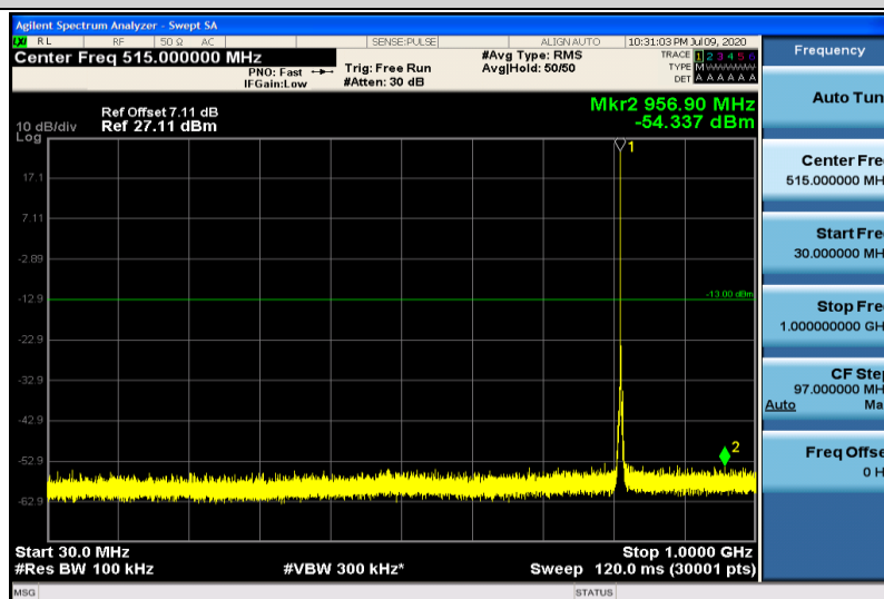
Band26-3MHz-16QAM-26705-1RB#0-30~1000MHz
