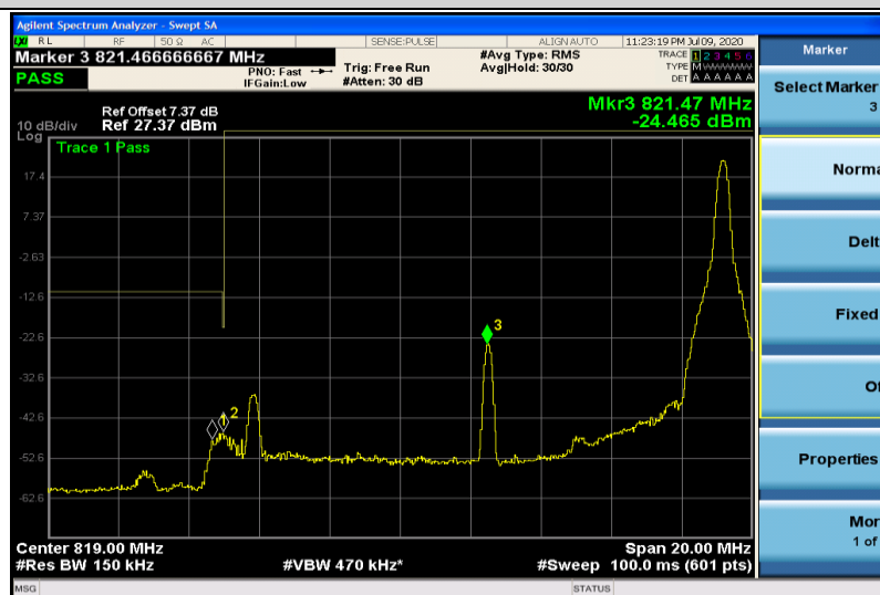
Band26-15MHz-16QAM-26765-1RB#74
