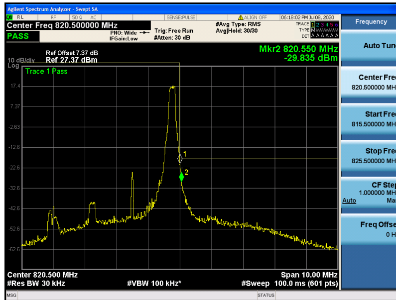
Band26-3MHz-16QAM-26740-1RB#14
