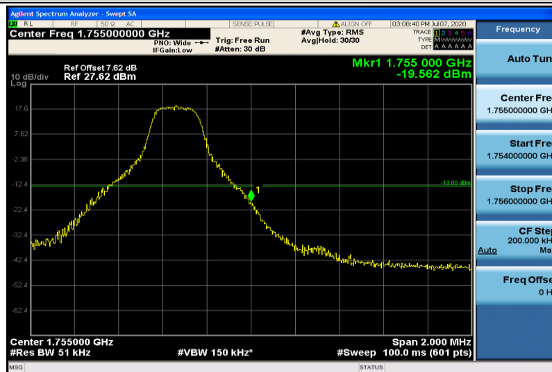
Band4-5MHz-QPSK-20375-1RB#24
