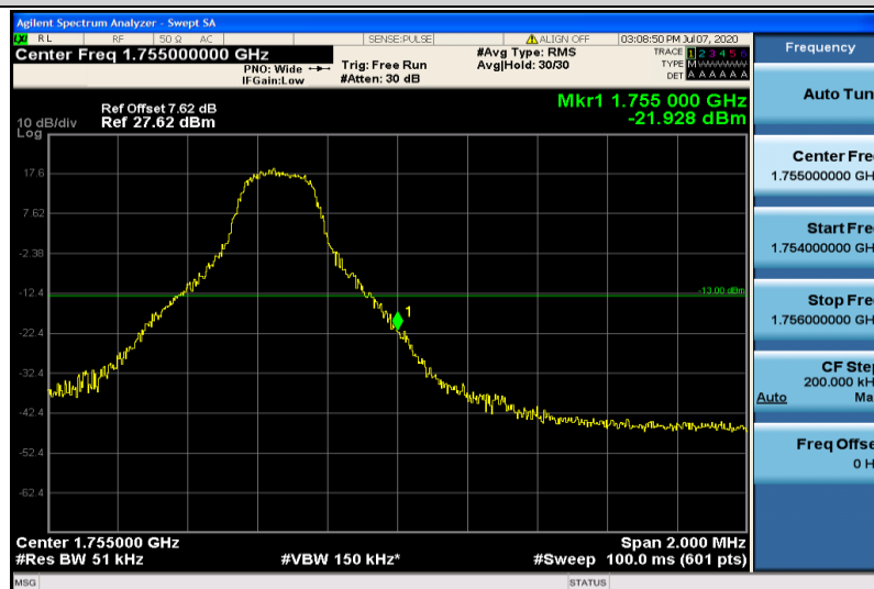
Band4-5MHz-16QAM-20375-1RB#24
