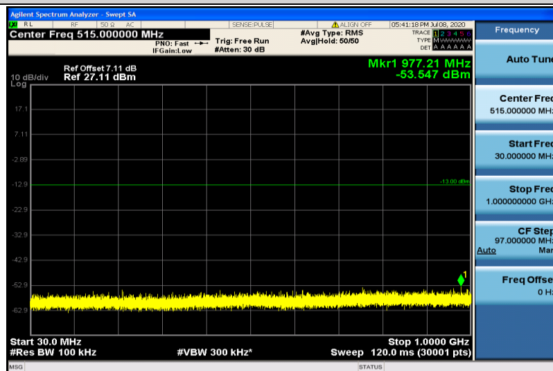
Band25-10MHz-16QAM-26640-1RB#0-30~1000MHz
