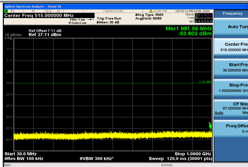
Band25-5MHz-16QAM-26665-1RB#0-30~1000MHz
