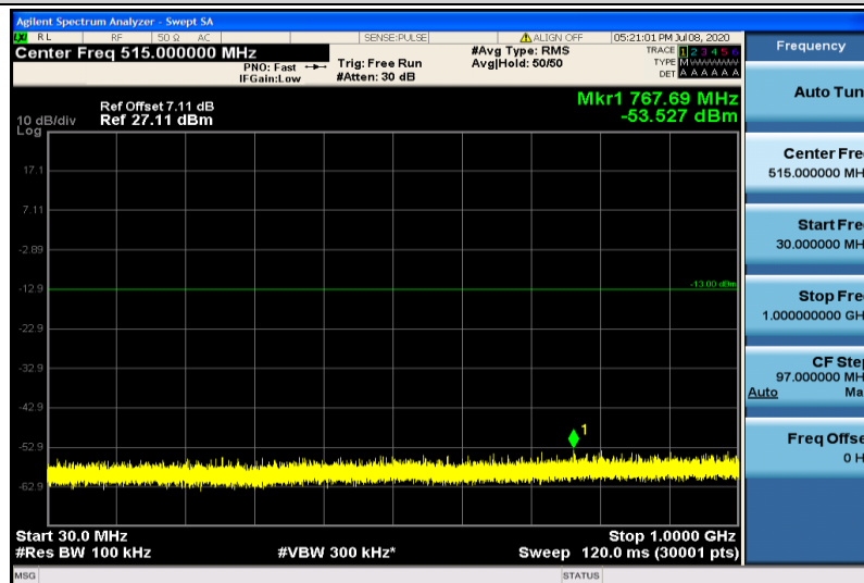
Band25-3MHz-16QAM-26055-1RB#0-30~1000MHz
