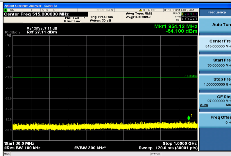
Band25-1.4MHz-16QAM-26047-1RB#0-30~1000MHz
