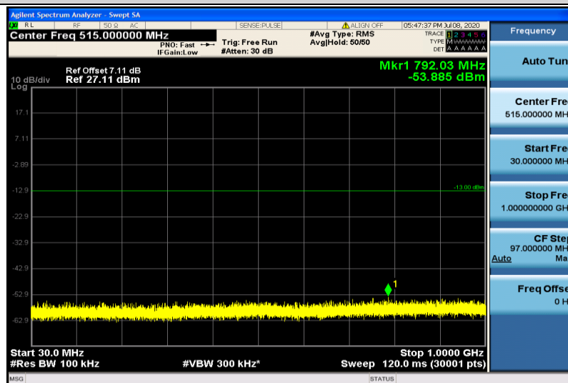
Band25-15MHz-QPSK-26615-1RB#0-30~1000MHz
