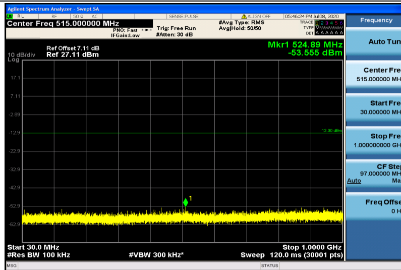
Band25-15MHz-QPSK-26365-1RB#0-30~1000MHz
