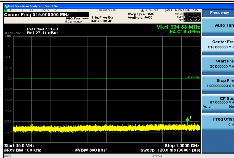
Band25-5MHz-QPSK-26665-1RB#0-30~1000MHz
