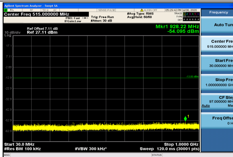
Band25-5MHz-16QAM-26065-1RB#0-30~1000MHz
