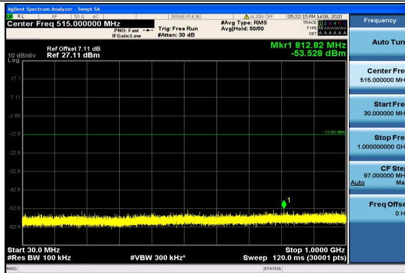
Band25-3MHz-16QAM-26365-1RB#0-30~1000MHz
