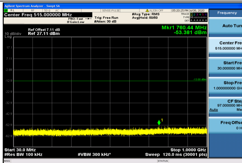
Band25-3MHz-QPSK-26055-1RB#0-30~1000MHz
