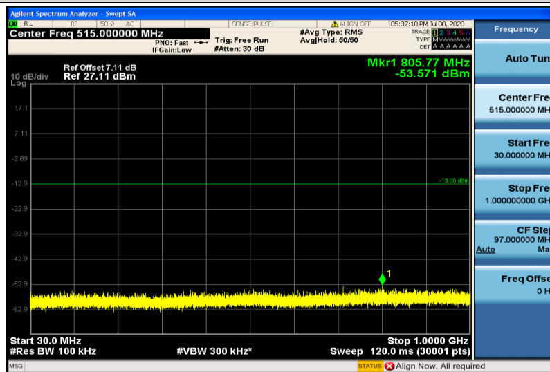
Band25-10MHz-16QAM-26090-1RB#0-30~1000MHz
