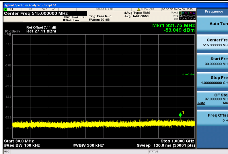
Band25-5MHz-16QAM-26365-1RB#0-30~1000MHz
