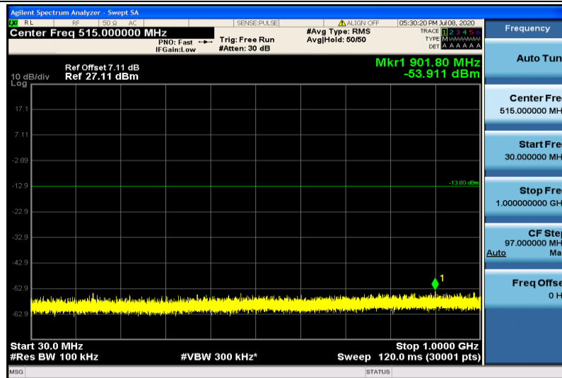
Band25-5MHz-QPSK-26365-1RB#0-30~1000MHz
