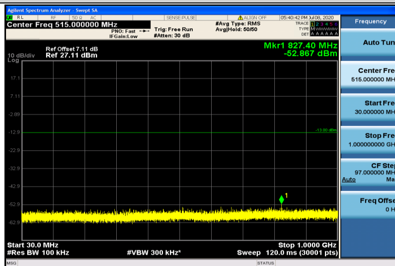
Band25-10MHz-QPSK-26640-1RB#0-30~1000MHz
