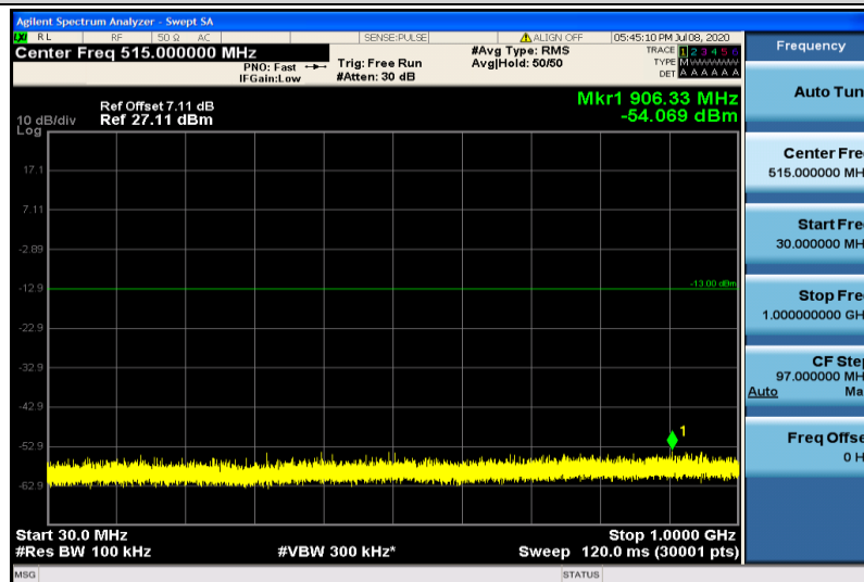
Band25-15MHz-QPSK-26115-1RB#0-30~1000MHz
