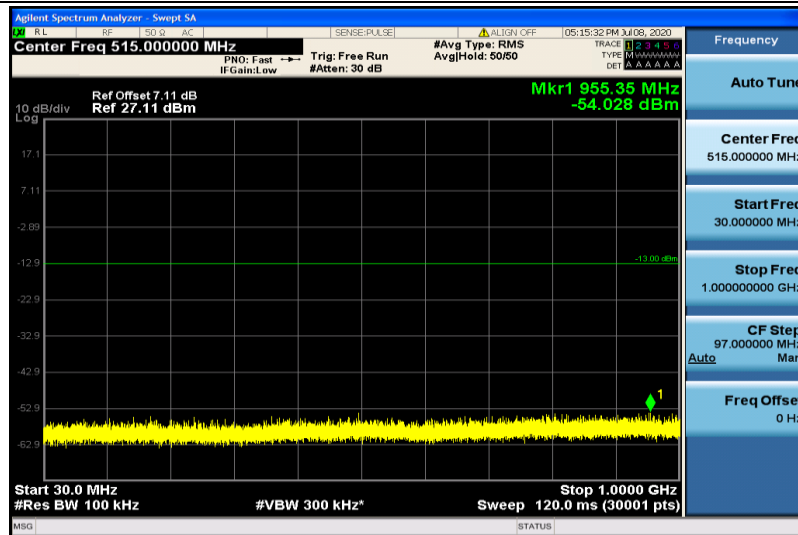
Band25-1.4MHz-16QAM-26365-1RB#0-30~1000MHz
