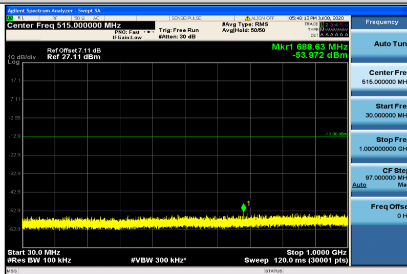
Band25-15MHz-16QAM-26615-1RB#0-30~1000MHz
