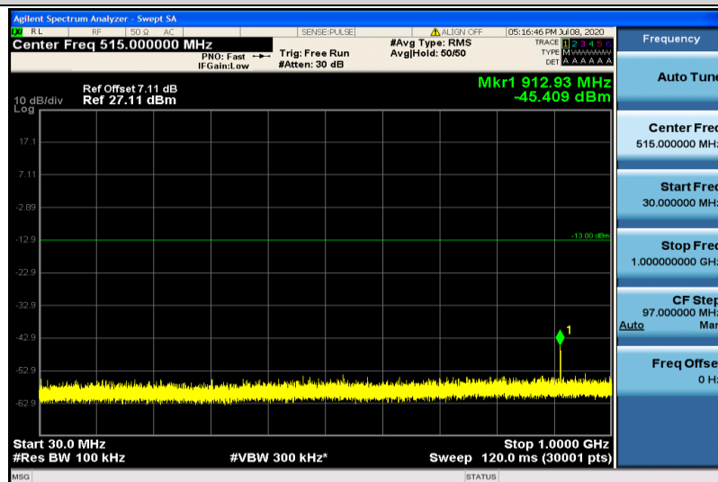
Band25-1.4MHz-16QAM-26683-1RB#0-30~1000MHz
