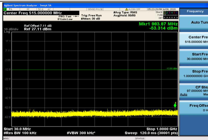
Band25-3MHz-16QAM-26675-1RB#0-30~1000MHz
