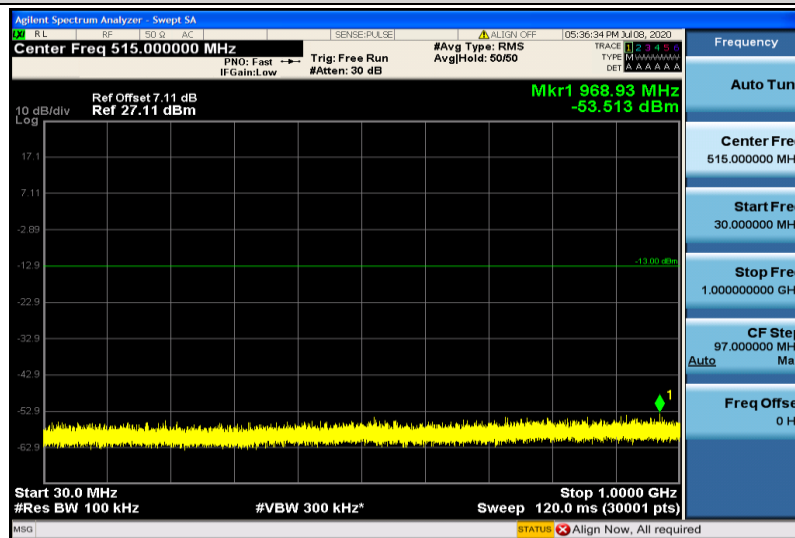
Band25-10MHz-QPSK-26090-1RB#0-30~1000MHz
