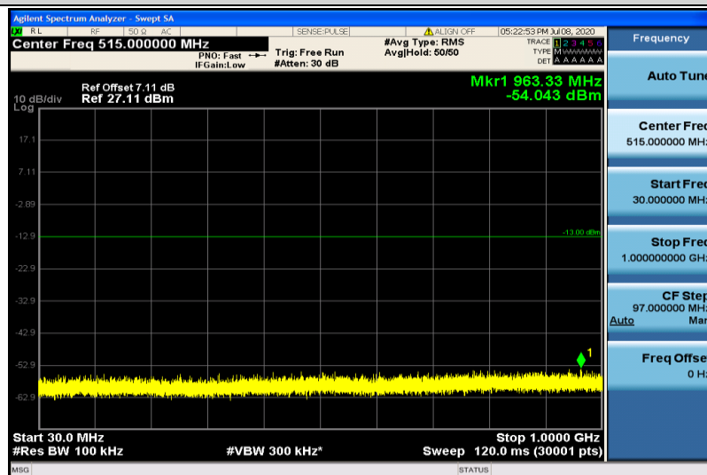
Band25-3MHz-QPSK-26675-1RB#0-30~1000MHz
