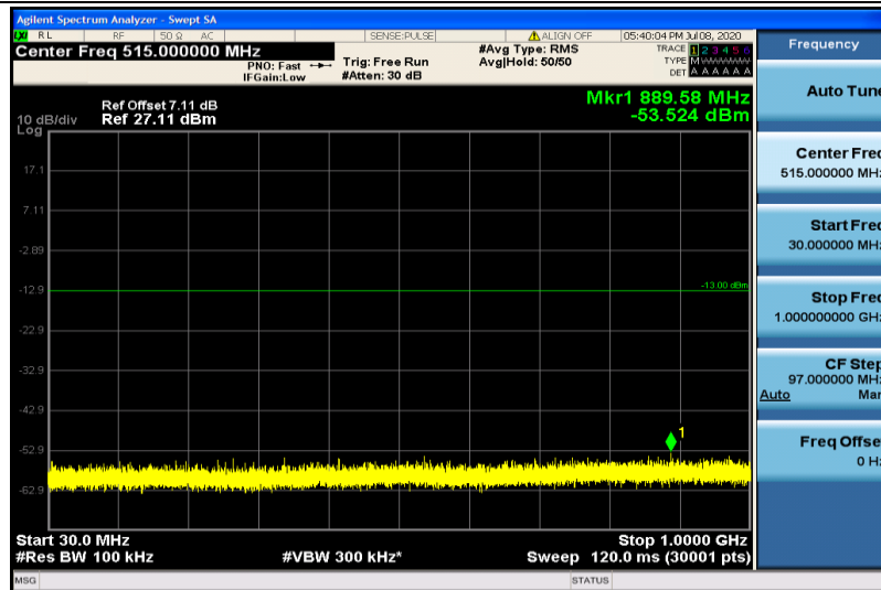
Band25-10MHz-16QAM-26365-1RB#0-30~1000MHz
