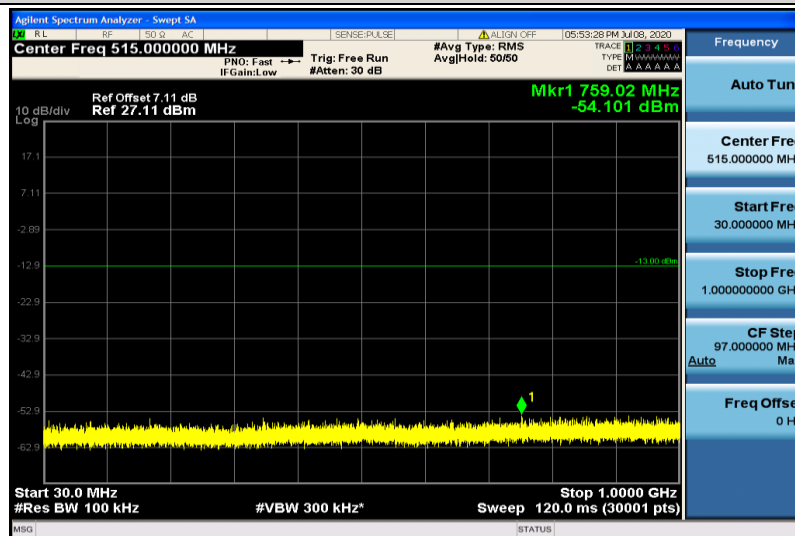
Band25-20MHz-16QAM-26140-1RB#0-30~1000MHz
