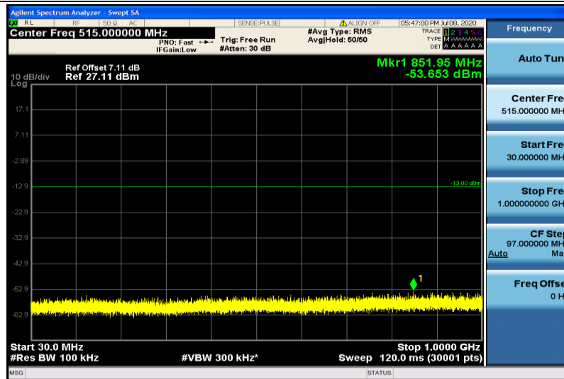
Band25-15MHz-16QAM-26365-1RB#0-30~1000MHz
