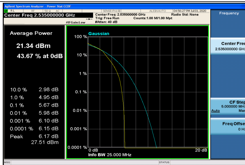
Band7-5MHz-16QAM-21100-25RB#0
