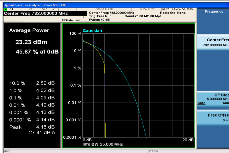
Band13-5MHz-QPSK-23230-1RB#0
