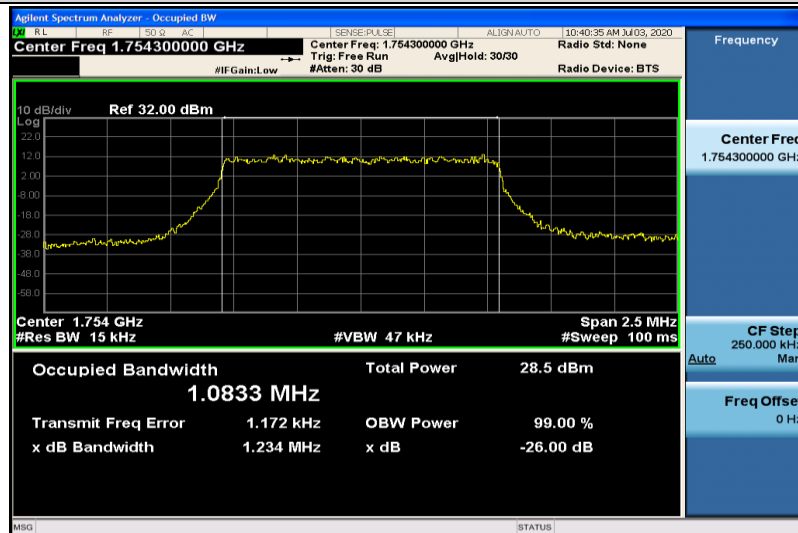
Band4-1.4MHz-QPSK-20393-6RB#0-1.0833
