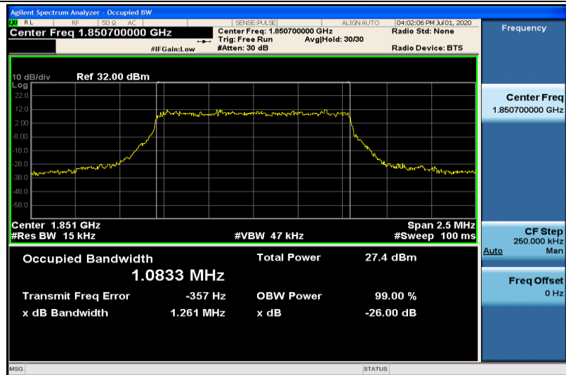
Band2-1.4MHz-16QAM-18607-6RB#0-1.0833
