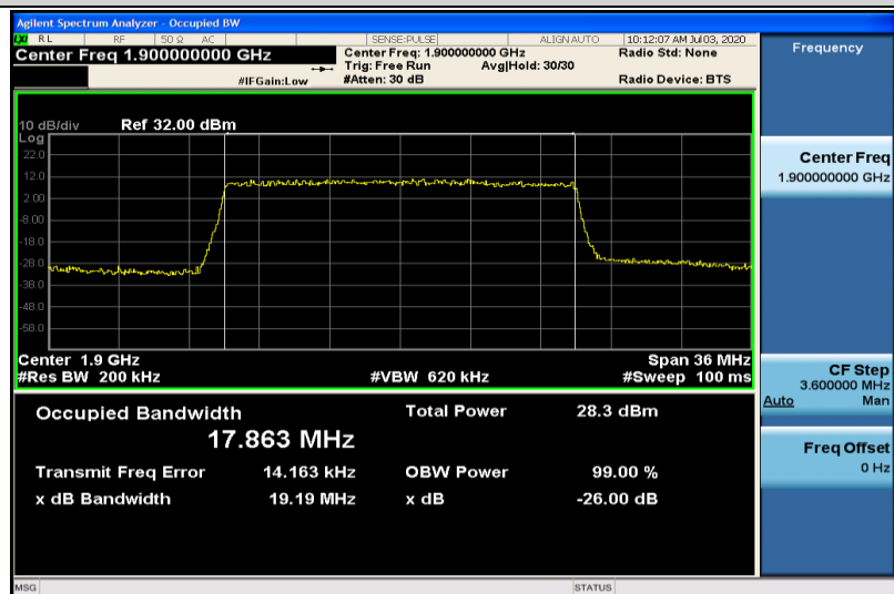
Band2-20MHz-16QAM-19100-100RB#0-17.863
