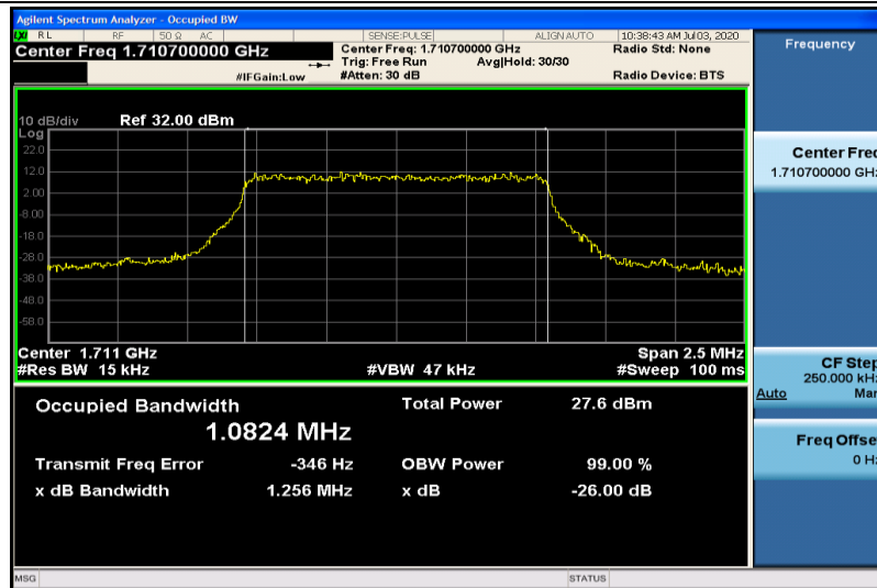
Band4-1.4MHz-16QAM-19957-6RB#0-1.0824
