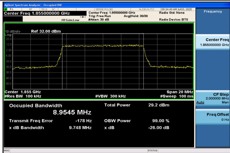
Band2-10MHz-QPSK-18650-50RB#0-8.9545
