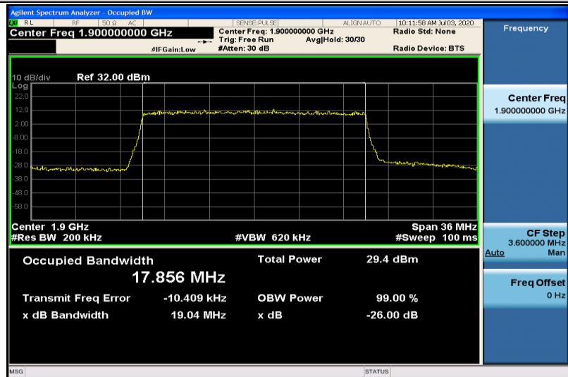
Band2-20MHz-QPSK-19100-100RB#0-17.856
