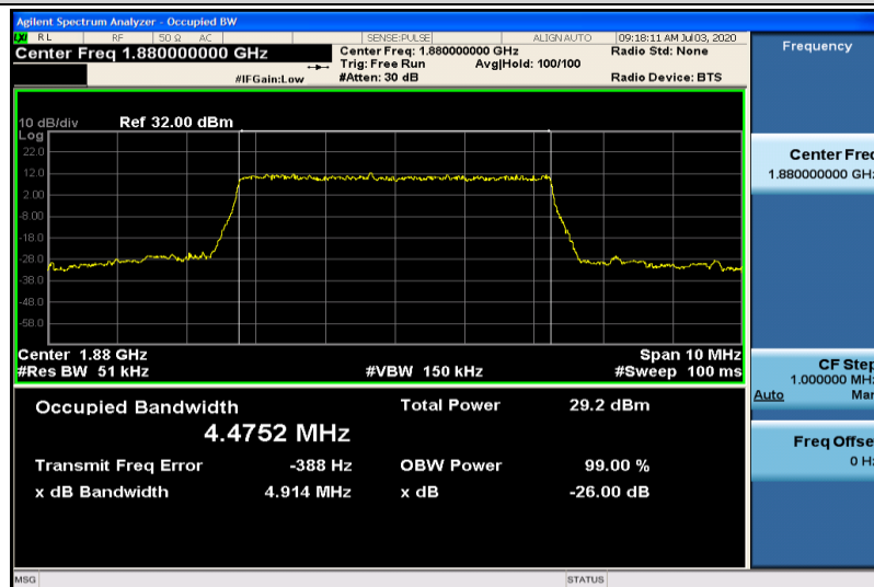
Band2-5MHz-QPSK-18900-25RB#0-4.4752
