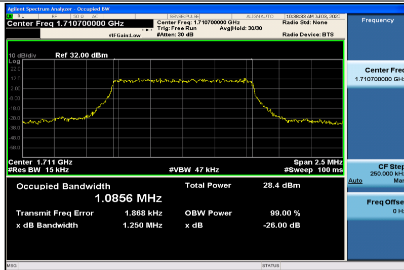
Band4-1.4MHz-QPSK-19957-6RB#0-1.0856
