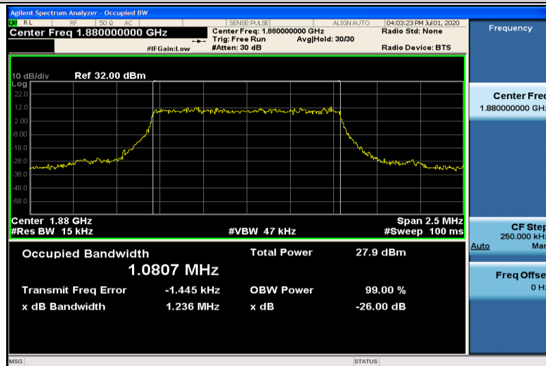
Band2-1.4MHz-QPSK-18900-6RB#0-1.0807
