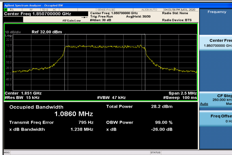
Band2-1.4MHz-QPSK-18607-6RB#0-1.0860
