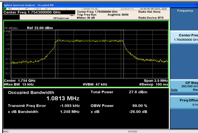
Band4-1.4MHz-16QAM-20393-6RB#0-1.0813
