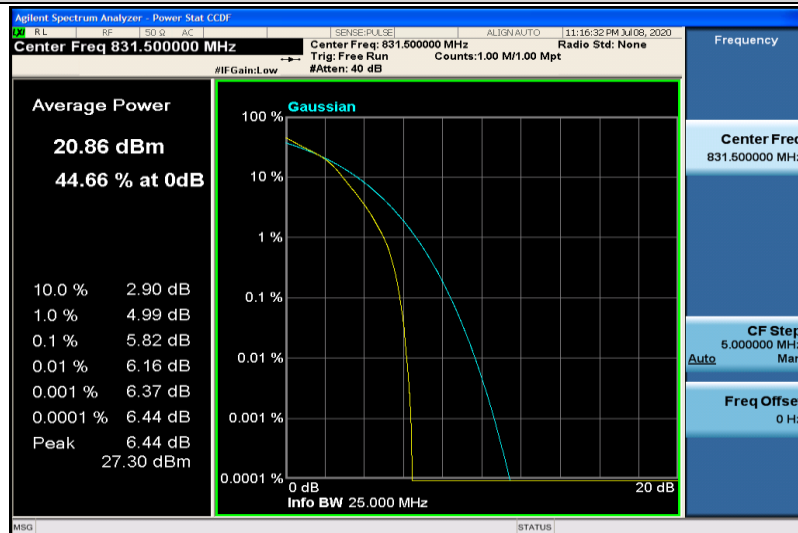
Band26-15MHz-16QAM-26865-75RB#0
