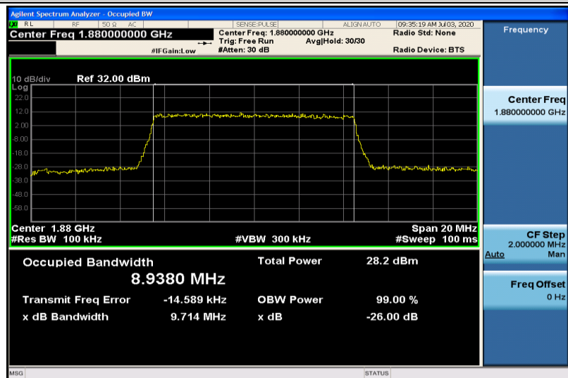
Band2-10MHz-16QAM-18900-50RB#0-8.9380
