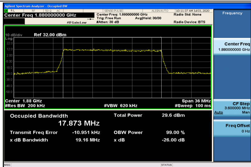
Band2-20MHz-QPSK-18900-100RB#0-17.873
