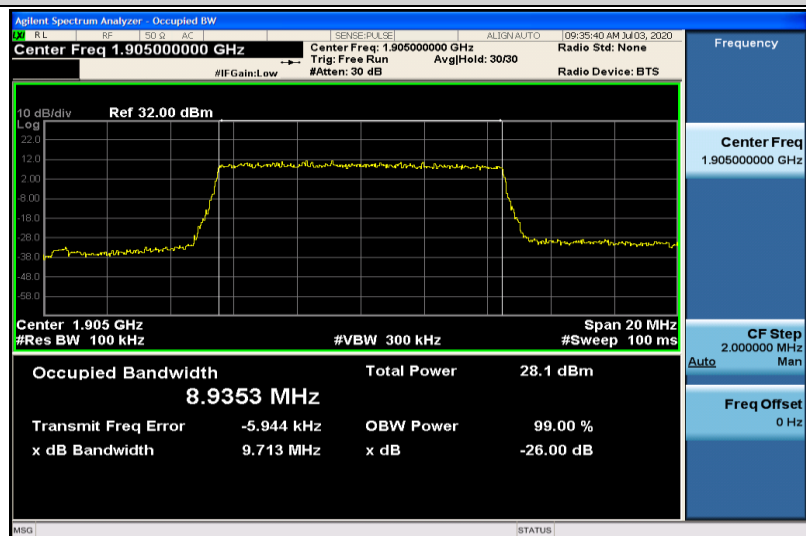
Band2-10MHz-16QAM-19150-50RB#0-8.9353
