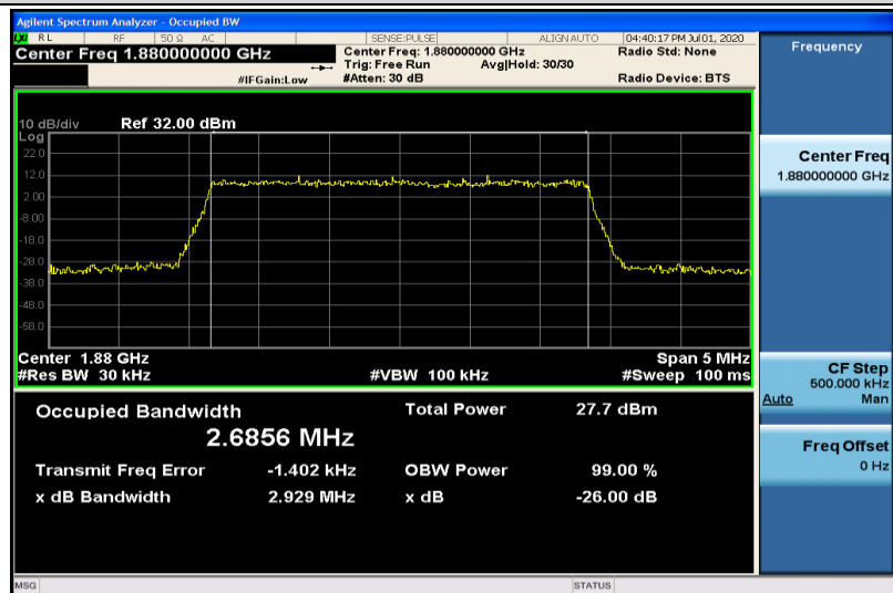
Band2-3MHz-16QAM-18900-15RB#0-2.6856
