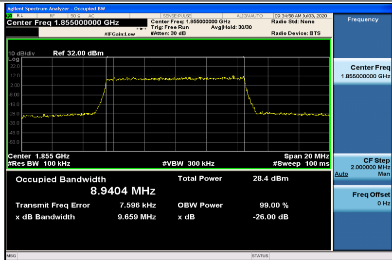
Band2-10MHz-16QAM-18650-50RB#0-8.9404
