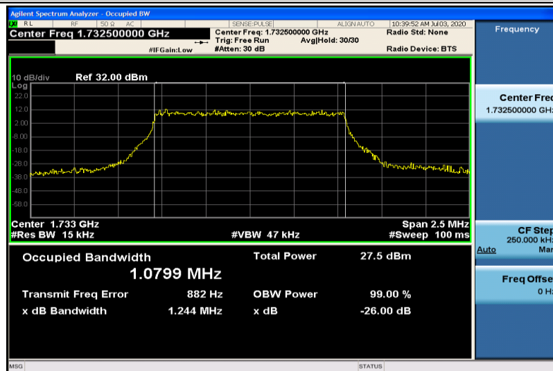
Band4-1.4MHz-16QAM-20175-6RB#0-1.0799
