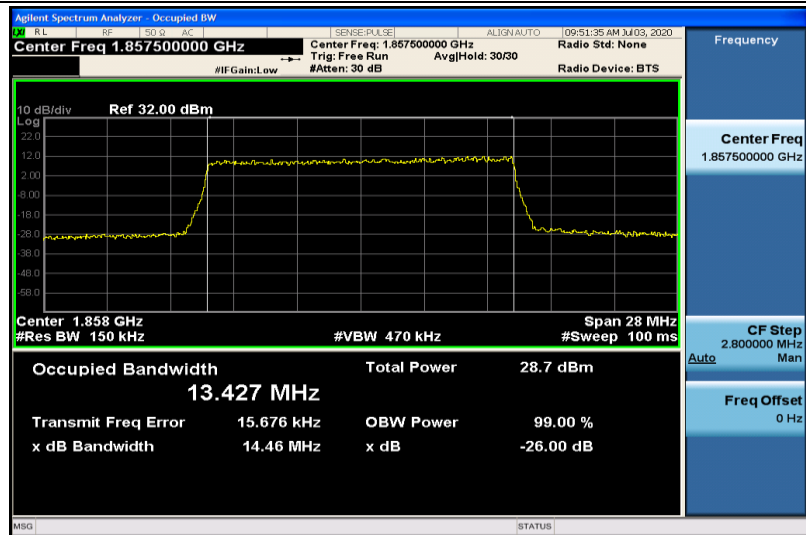
Band2-15MHz-16QAM-18675-75RB#0-13.427
