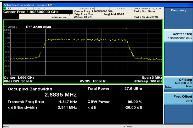
Band2-3MHz-16QAM-19185-15RB#0-2.6835
