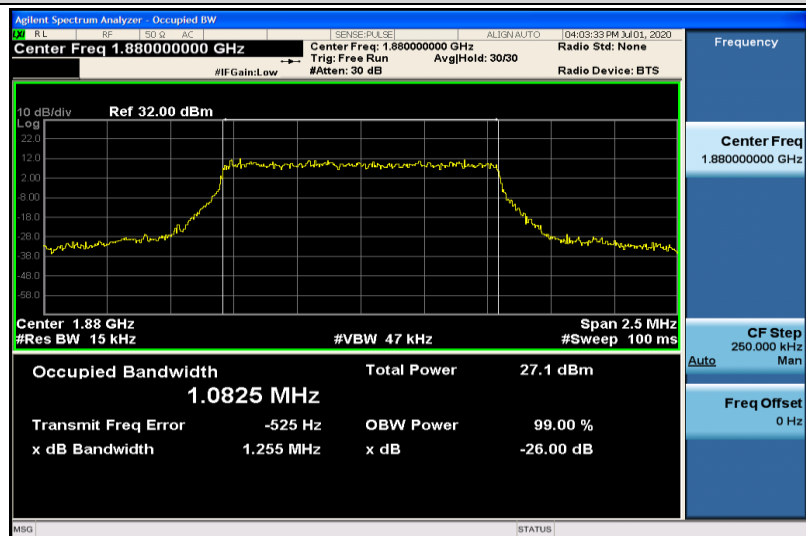
Band2-1.4MHz-16QAM-18900-6RB#0-1.0825
