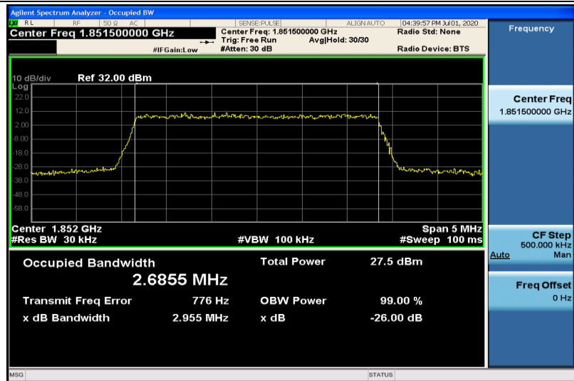
Band2-3MHz-16QAM-18615-15RB#0-2.6855
