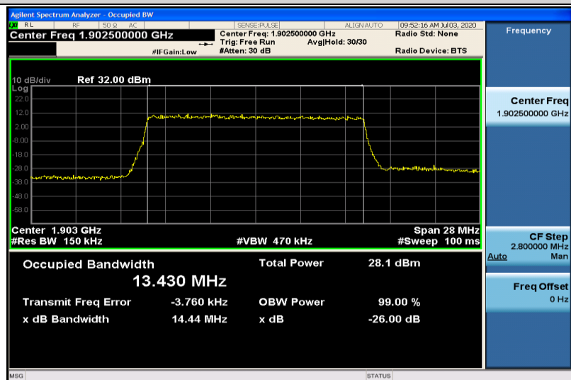
Band2-15MHz-16QAM-19125-75RB#0-13.430
