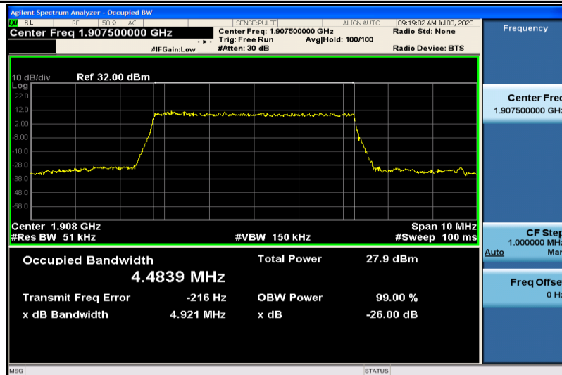
Band2-5MHz-16QAM-19175-25RB#0-4.4839
