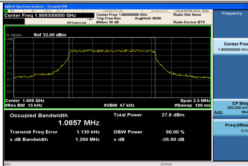
Band2-1.4MHz-QPSK-19193-6RB#0-1.0857
