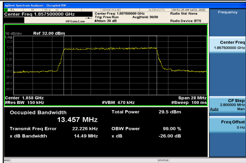
Band2-15MHz-QPSK-18675-75RB#0-13.457
