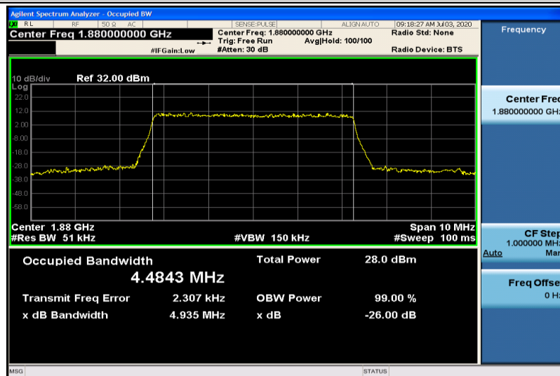
Band2-5MHz-16QAM-18900-25RB#0-4.4843
