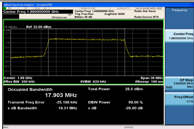
Band2-20MHz-16QAM-18900-100RB#0-17.903
