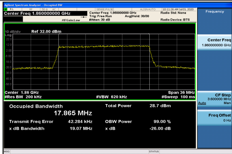
Band2-20MHz-16QAM-18700-100RB#0-17.865
