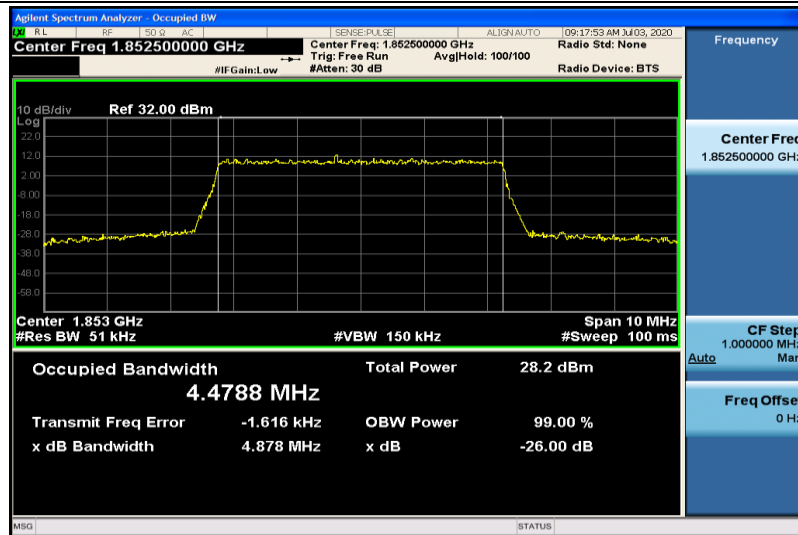
Band2-5MHz-16QAM-18625-25RB#0-4.4788
