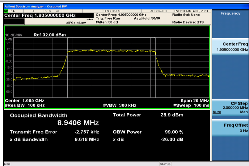
Band2-10MHz-QPSK-19150-50RB#0-8.9406
