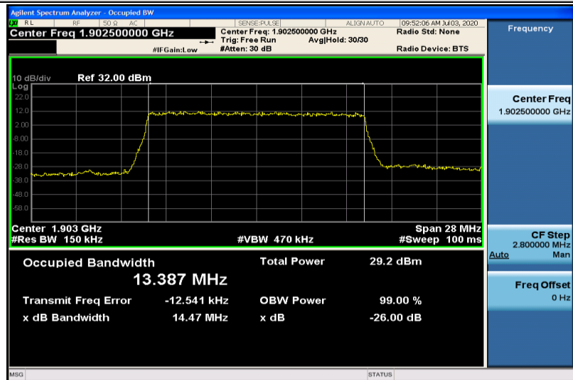
Band2-15MHz-QPSK-19125-75RB#0-13.387
