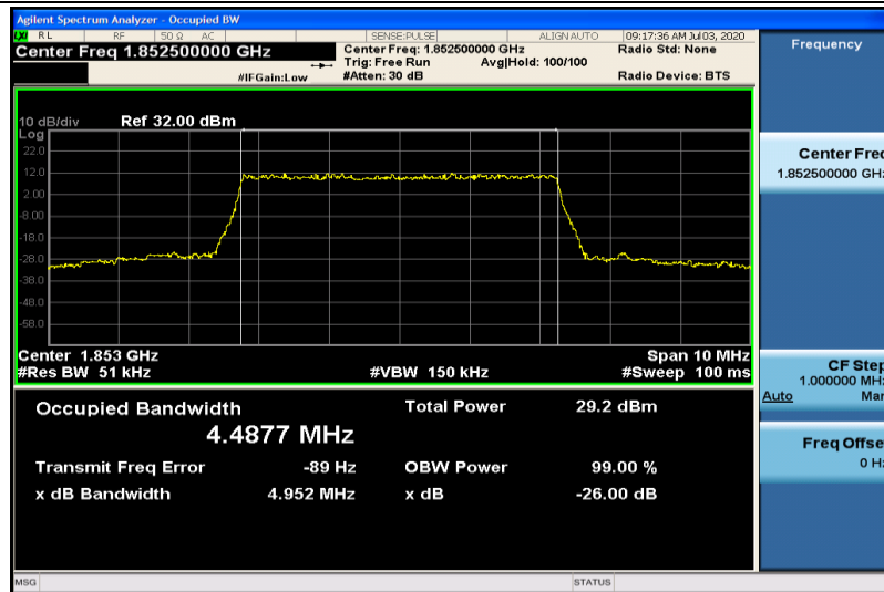
Band2-5MHz-QPSK-18625-25RB#0-4.4877
