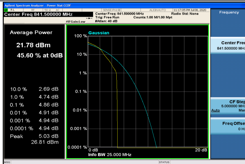
Band26-15MHz-16QAM-26965-1RB#0
