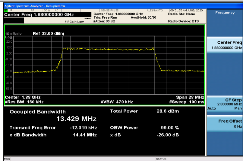
Band2-15MHz-16QAM-18900-75RB#0-13.429
