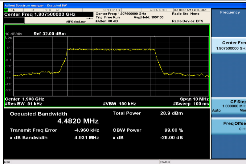
Band2-5MHz-QPSK-19175-25RB#0-4.4820
