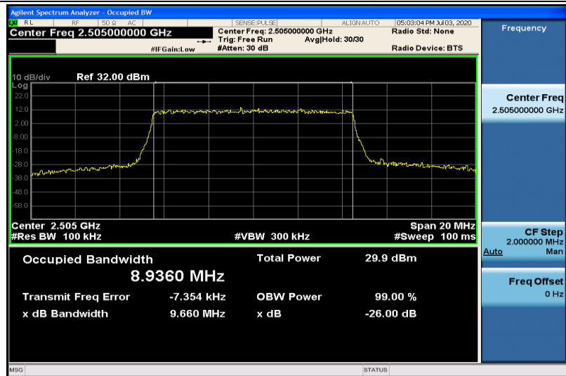
Band7-10MHz-16QAM-20800-50RB#0-8.9360
