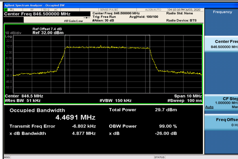
Band5-5MHz-16QAM-20625-25RB#0-4.4691
