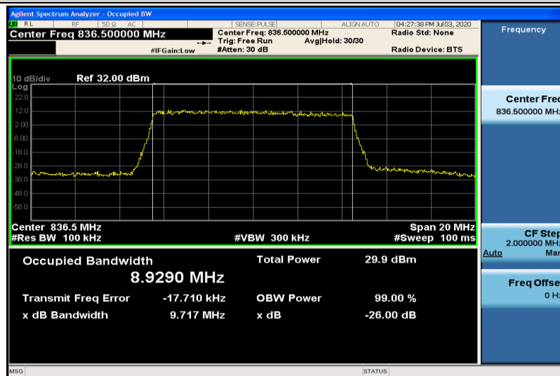
Band5-10MHz-16QAM-20525-50RB#0-8.9290
