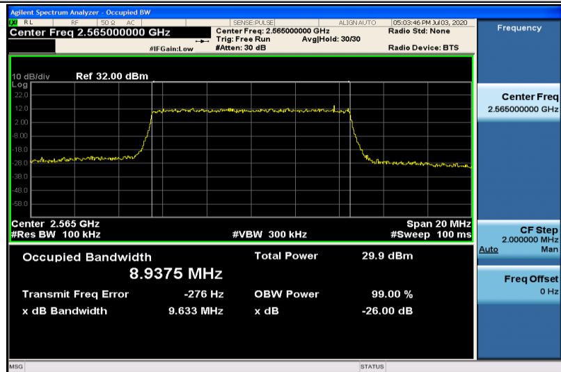
Band7-10MHz-16QAM-21400-50RB#0-8.9375
