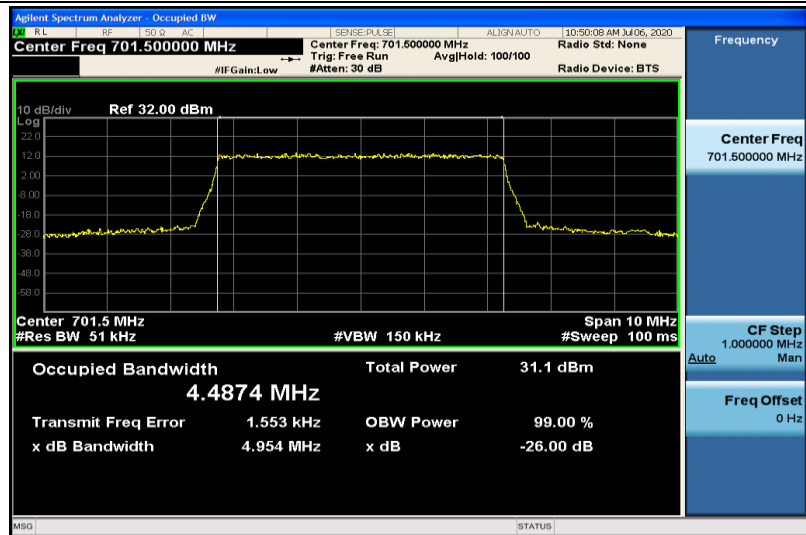
Band12-5MHz-QPSK-23035-25RB#0-4.4874
