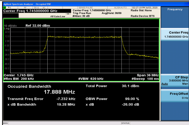
Band4-20MHz-QPSK-20300-100RB#0-17.888
