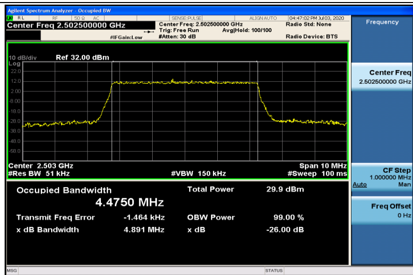
Band7-5MHz-16QAM-20775-25RB#0-4.4750
