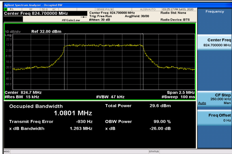
Band5-1.4MHz-QPSK-20407-6RB#0-1.0801
