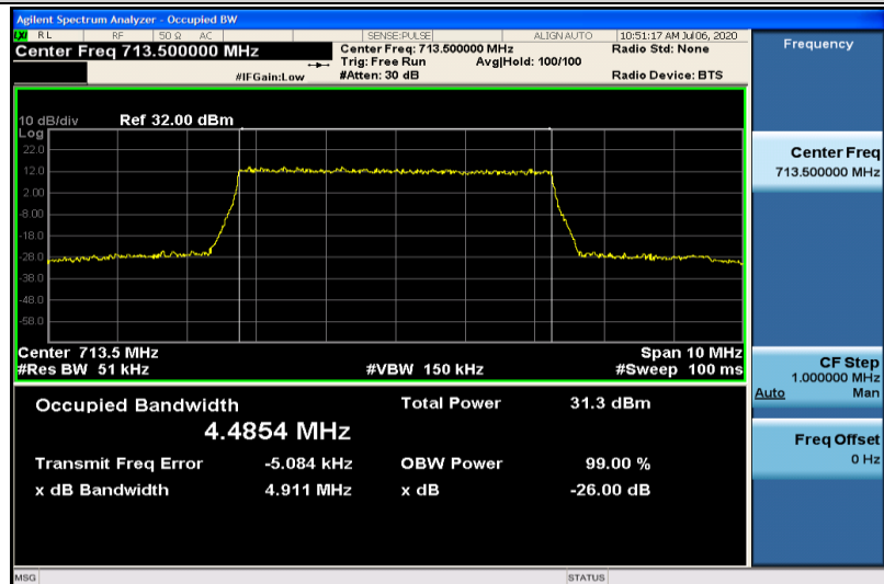
Band12-5MHz-QPSK-23155-25RB#0-4.4854
