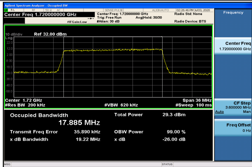
Band4-20MHz-16QAM-20050-100RB#0-17.885
