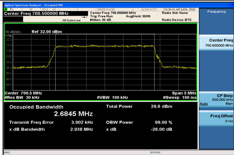
Band12-3MHz-16QAM-23025-15RB#0-2.6845
