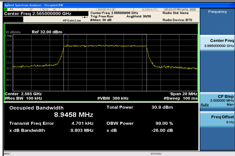
Band7-10MHz-QPSK-21400-50RB#0-8.9458
