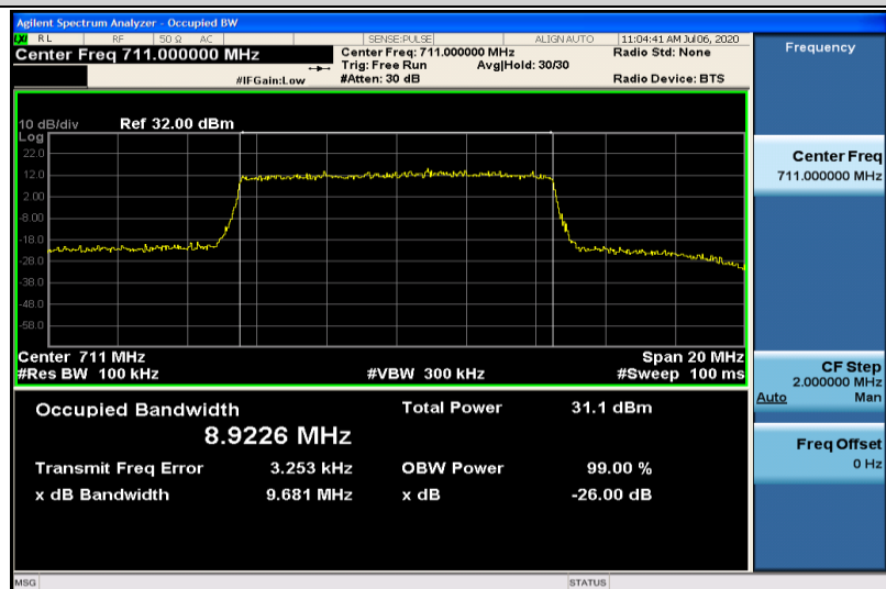
Band12-10MHz-QPSK-23130-50RB#0-8.9226
