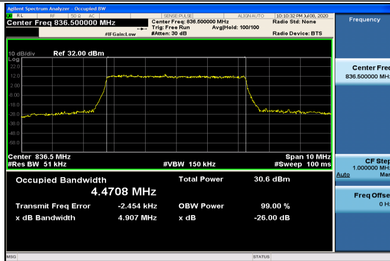
Band26-5MHz-QPSK-26915-25RB#0-4.4708
