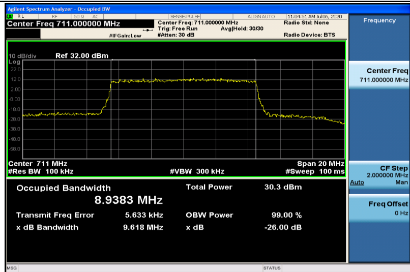
Band12-10MHz-16QAM-23130-50RB#0-8.9383
