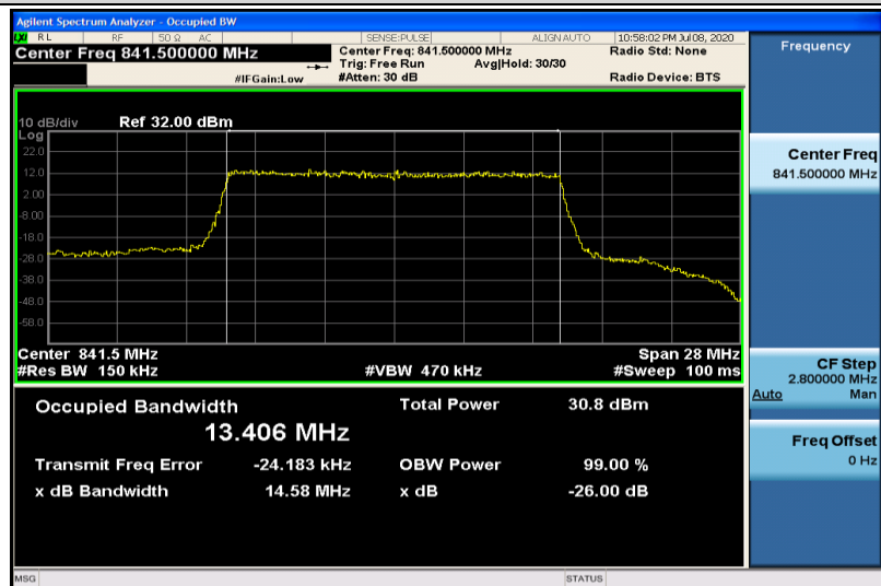
Band26-15MHz-QPSK-26965-75RB#0-13.406
