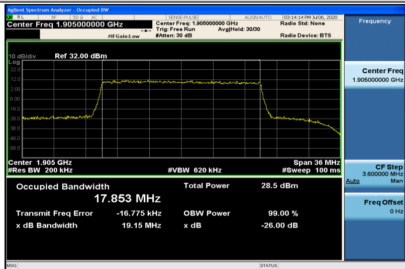
Band25-20MHz-16QAM-26590-100RB#0-17.853
