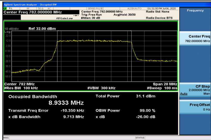
Band13-10MHz-QPSK-23230-50RB#0-8.9333
