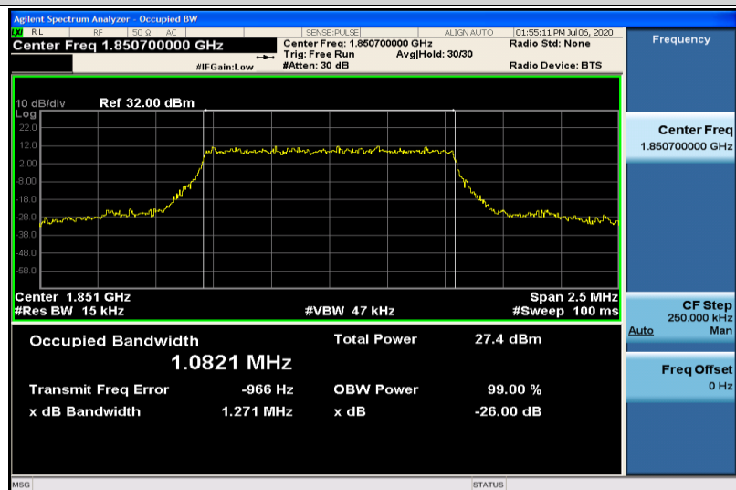
Band25-1.4MHz-16QAM-26047-6RB#0-1.0821
