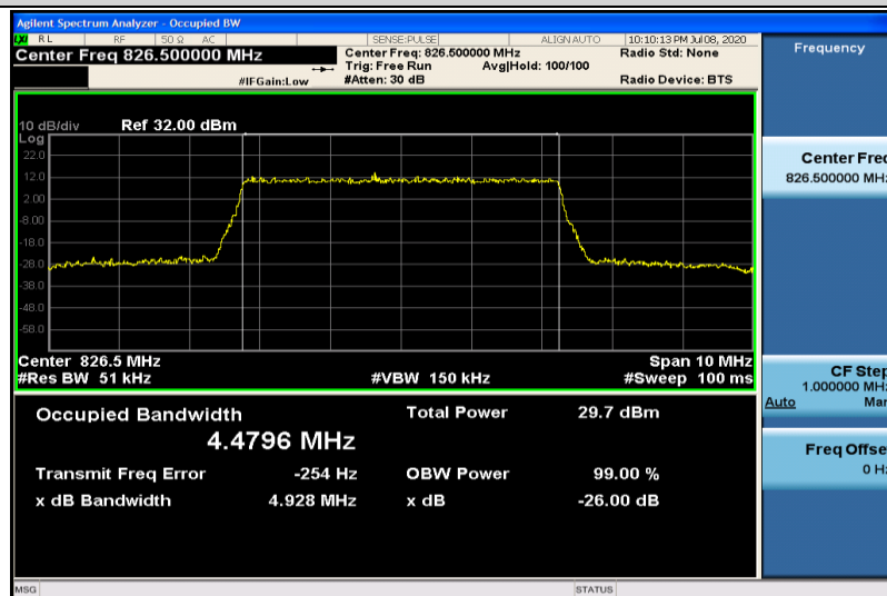
Band26-5MHz-16QAM-26815-25RB#0-4.4796
