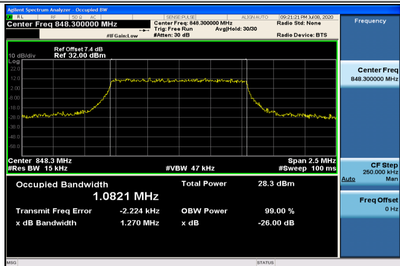
Band26-1.4MHz-16QAM-27033-6RB#0-1.0821
