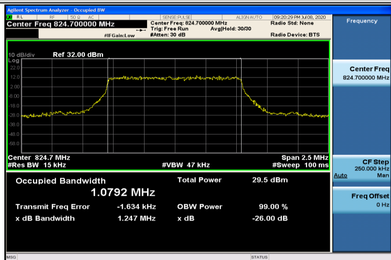
Band26-1.4MHz-QPSK-26797-6RB#0-1.0792
