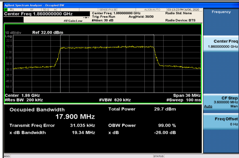
Band25-20MHz-QPSK-26140-100RB#0-17.900
