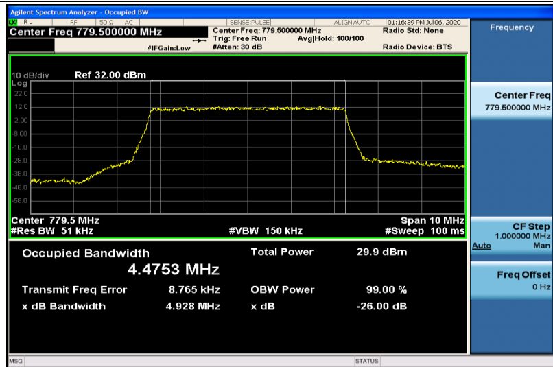
Band13-5MHz-16QAM-23205-25RB#0-4.4753
