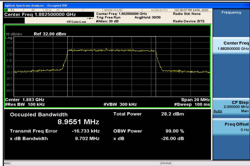
Band25-10MHz-16QAM-26365-50RB#0-8.9551
