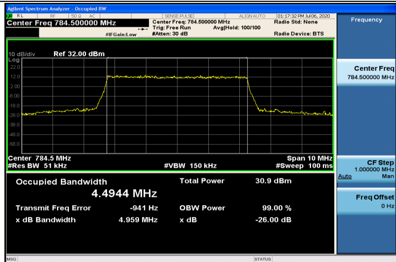
Band13-5MHz-QPSK-23255-25RB#0-4.4944
