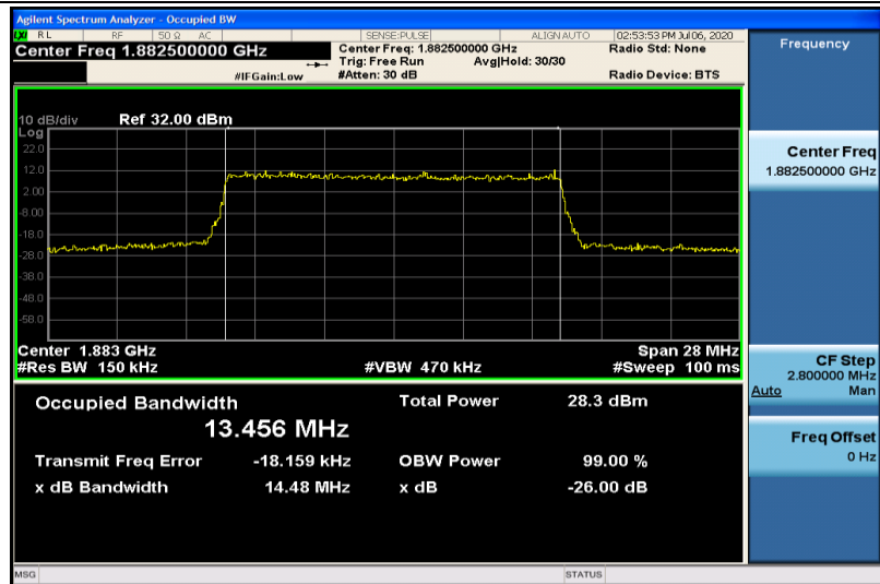
Band25-15MHz-16QAM-26365-75RB#0-13.456
