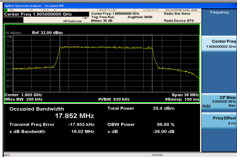
Band25-20MHz-QPSK-26590-100RB#0-17.852
