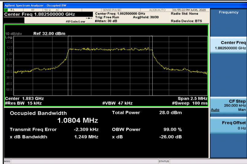
Band25-1.4MHz-QPSK-26365-6RB#0-1.0804
