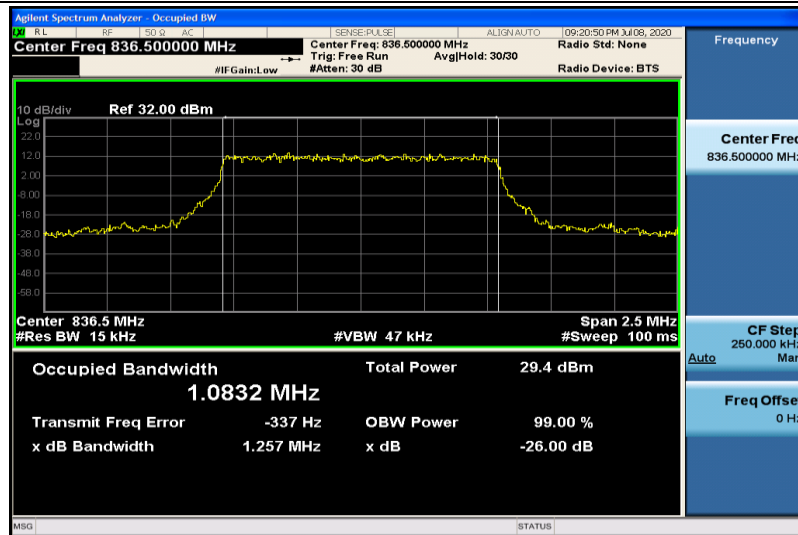
Band26-1.4MHz-QPSK-26915-6RB#0-1.0832
