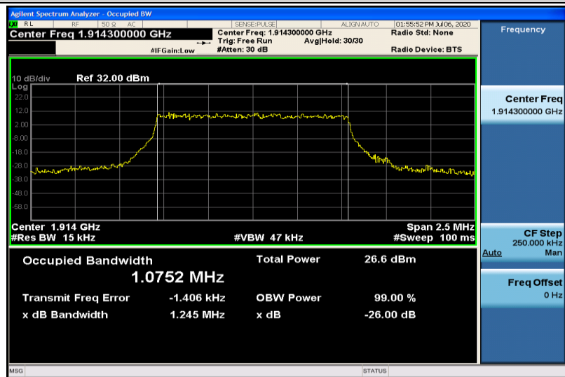
Band25-1.4MHz-16QAM-26683-6RB#0-1.0752
