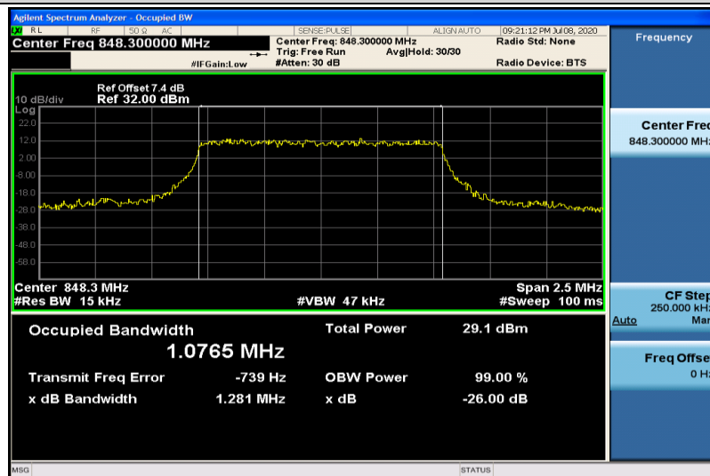
Band26-1.4MHz-QPSK-27033-6RB#0-1.0765
