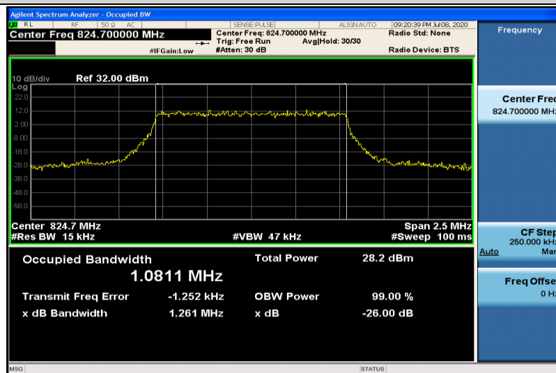
Band26-1.4MHz-16QAM-26797-6RB#0-1.0811
