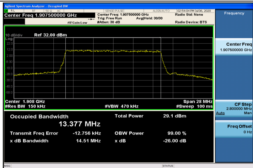
Band25-15MHz-QPSK-26615-75RB#0-13.377
