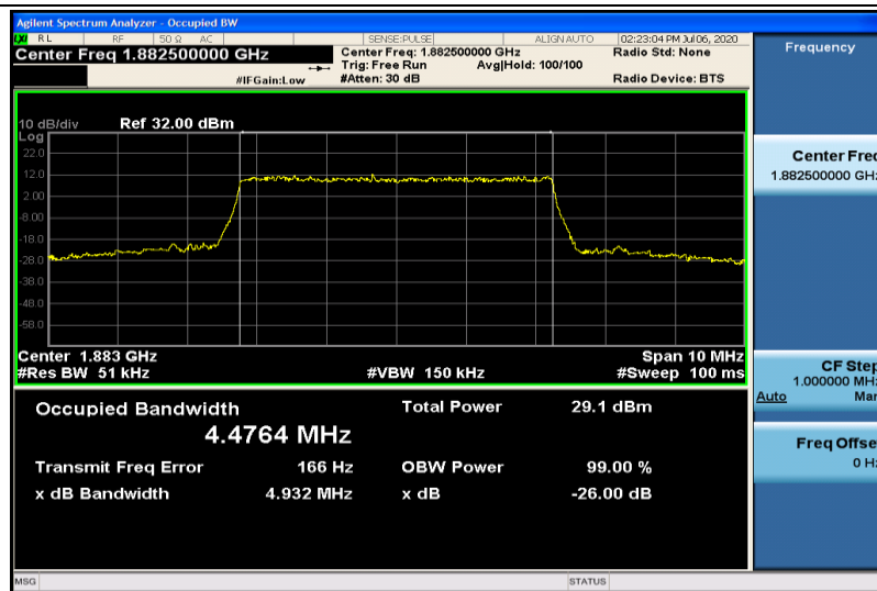
Band25-5MHz-QPSK-26365-25RB#0-4.4764
