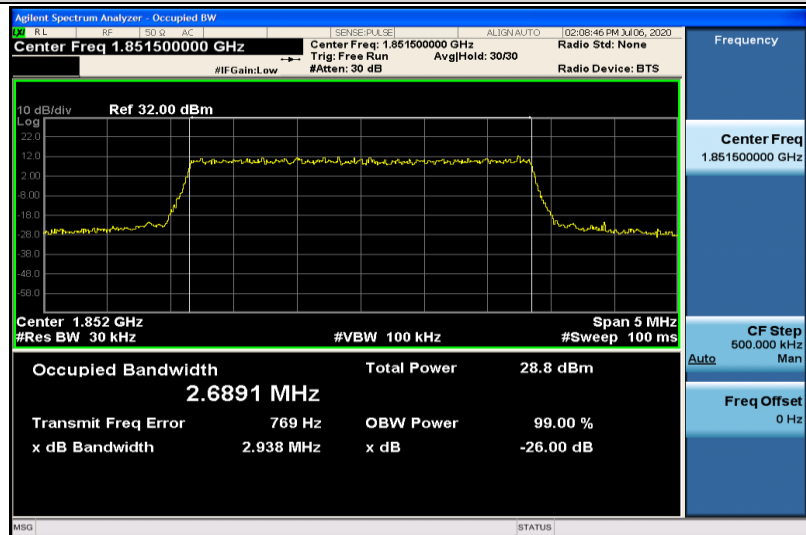
Band25-3MHz-QPSK-26055-15RB#0-2.6891
