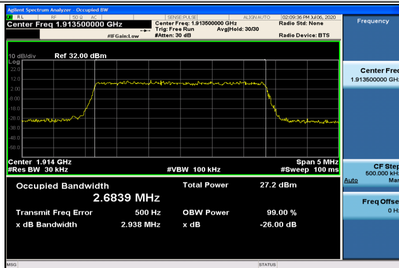
Band25-3MHz-16QAM-26675-15RB#0-2.6839
