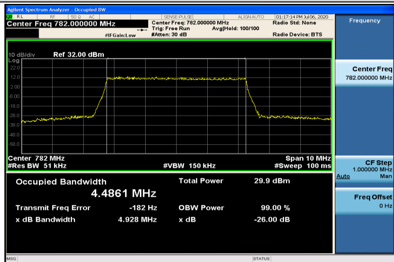
Band13-5MHz-16QAM-23230-25RB#0-4.4861
