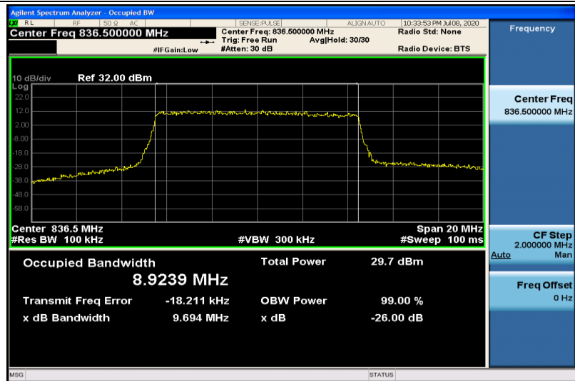
Band26-10MHz-16QAM-26915-50RB#0-8.9239
