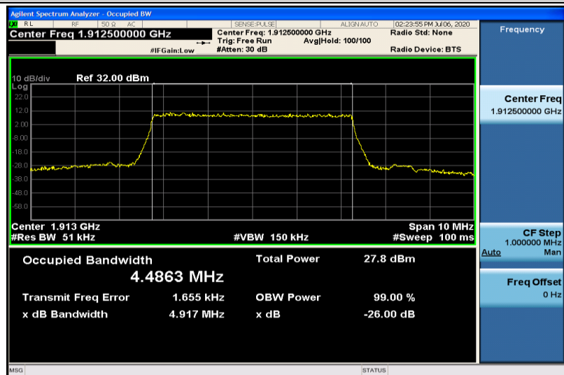
Band25-5MHz-16QAM-26665-25RB#0-4.4863
