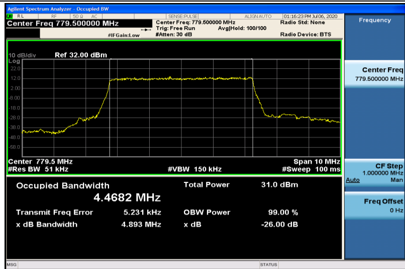
Band13-5MHz-QPSK-23205-25RB#0-4.4682
