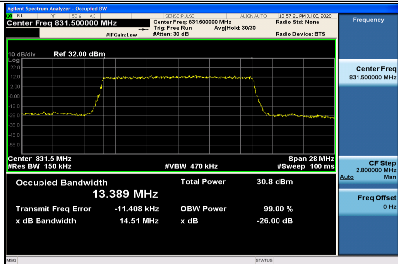
Band26-15MHz-QPSK-26865-75RB#0-13.389
