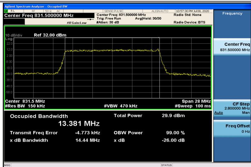
Band26-15MHz-16QAM-26865-75RB#0-13.381
