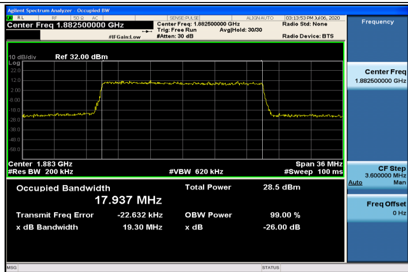
Band25-20MHz-16QAM-26365-100RB#0-17.937
