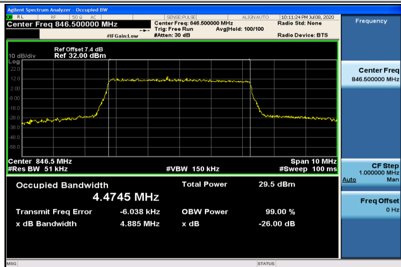
Band26-5MHz-16QAM-27015-25RB#0-4.4745
