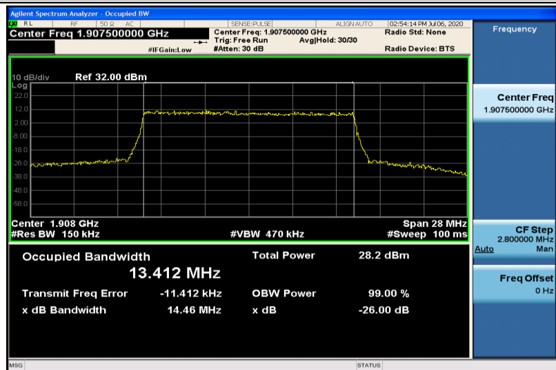
Band25-15MHz-16QAM-26615-75RB#0-13.412
