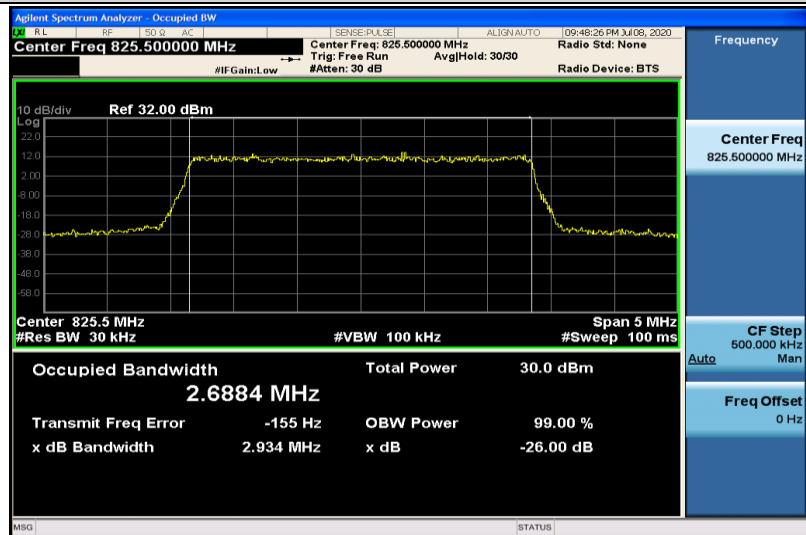
Band26-3MHz-QPSK-26805-15RB#0-2.6884
