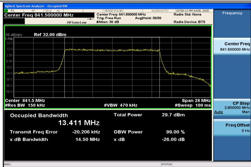
Band26-15MHz-16QAM-26965-75RB#0-13.411
