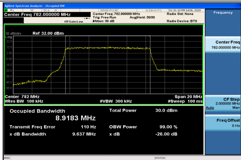
Band13-10MHz-16QAM-23230-50RB#0-8.9183
