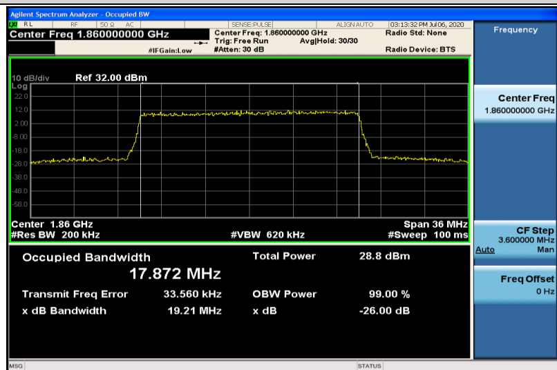
Band25-20MHz-16QAM-26140-100RB#0-17.872
