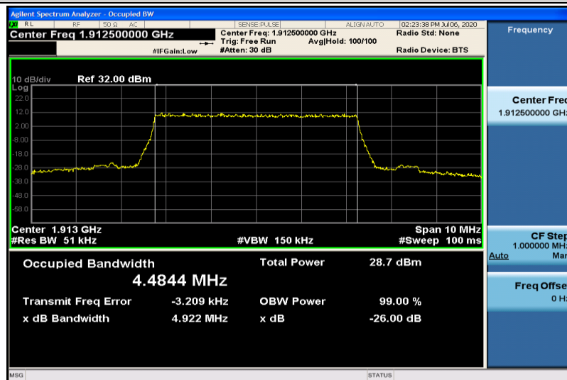
Band25-5MHz-QPSK-26665-25RB#0-4.4844
