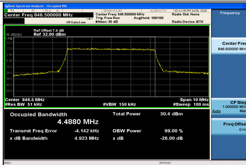
Band26-5MHz-QPSK-27015-25RB#0-4.4880
