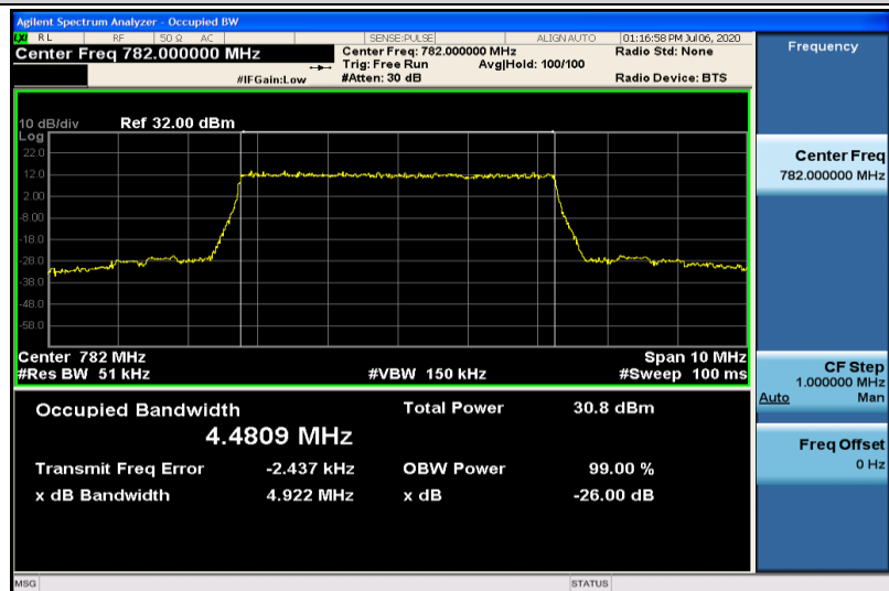
Band13-5MHz-QPSK-23230-25RB#0-4.4809
