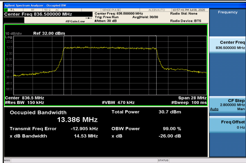
Band26-15MHz-QPSK-26915-75RB#0-13.386
