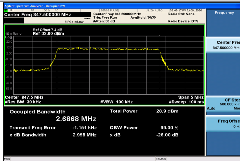
Band26-3MHz-16QAM-27025-15RB#0-2.6868
