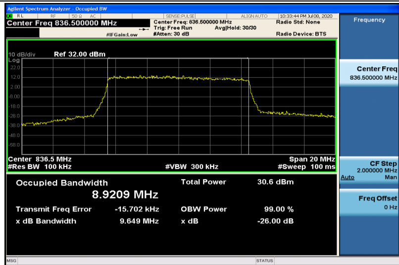
Band26-10MHz-QPSK-26915-50RB#0-8.9209
