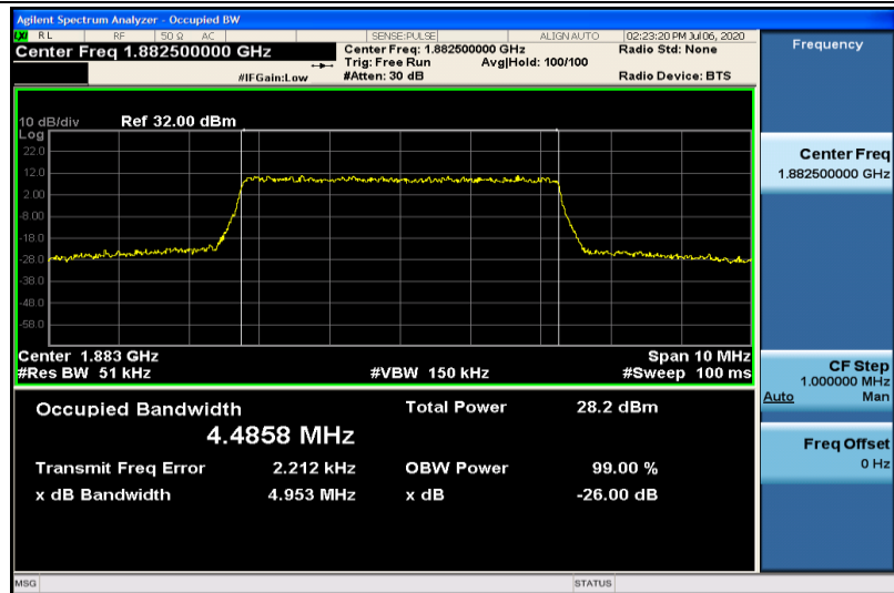
Band25-5MHz-16QAM-26365-25RB#0-4.4858
