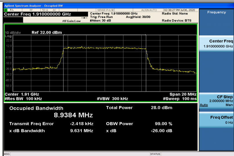
Band25-10MHz-16QAM-26640-50RB#0-8.9384
