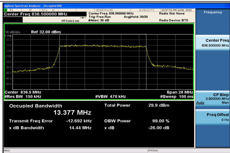
Band26-15MHz-16QAM-26915-75RB#0-13.377
