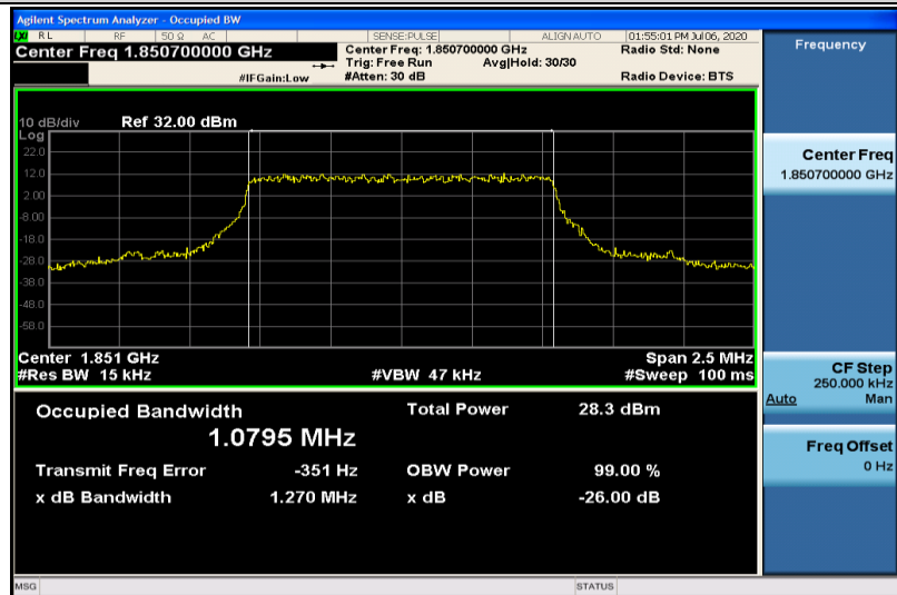
Band25-1.4MHz-QPSK-26047-6RB#0-1.0795
