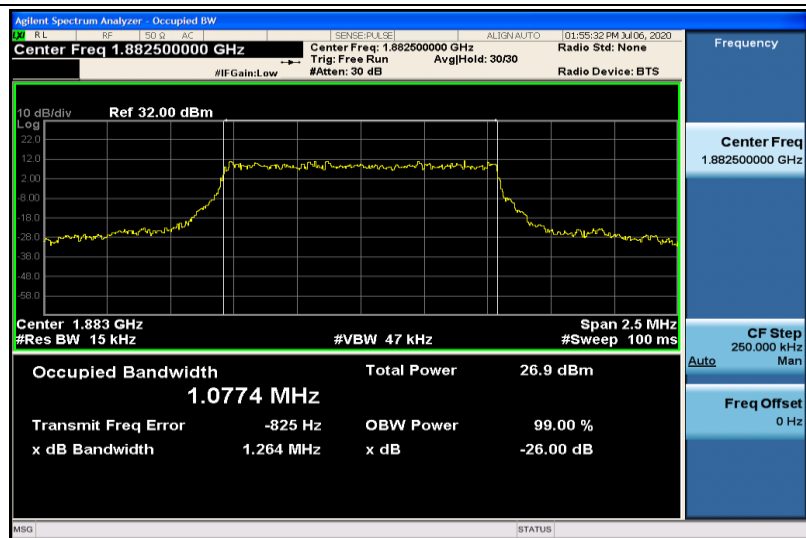
Band25-1.4MHz-16QAM-26365-6RB#0-1.0774
