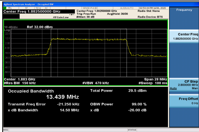
Band25-15MHz-QPSK-26365-75RB#0-13.439
