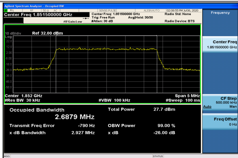
Band25-3MHz-16QAM-26055-15RB#0-2.6879
