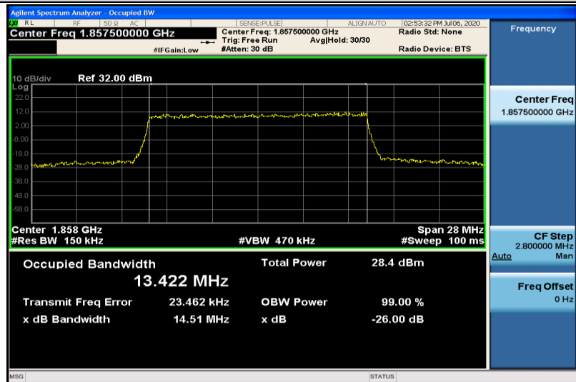
Band25-15MHz-16QAM-26115-75RB#0-13.422
