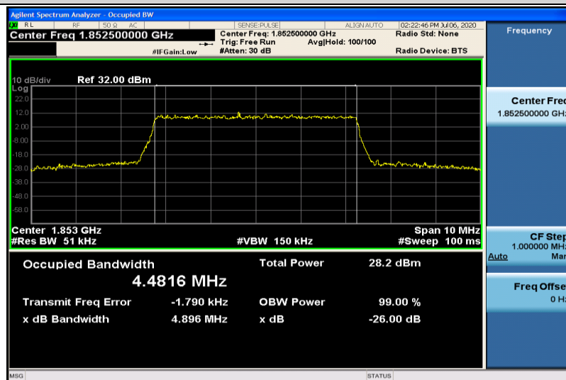
Band25-5MHz-16QAM-26065-25RB#0-4.4816
