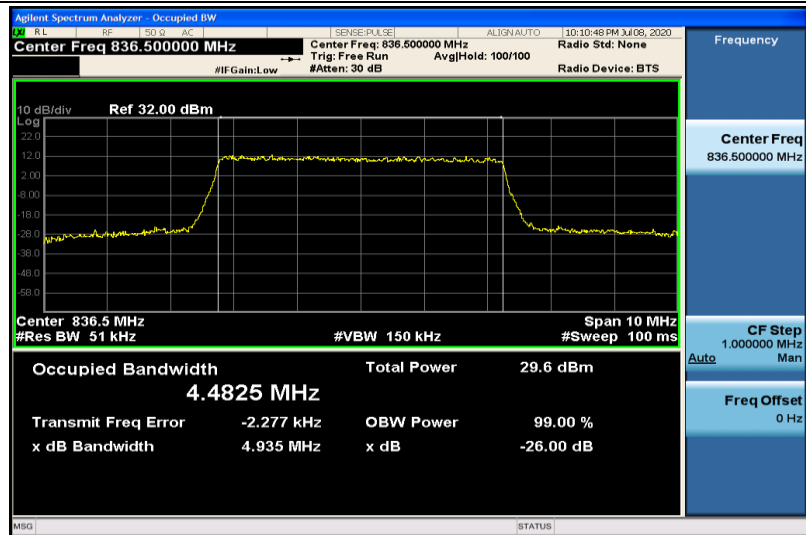
Band26-5MHz-16QAM-26915-25RB#0-4.4825
