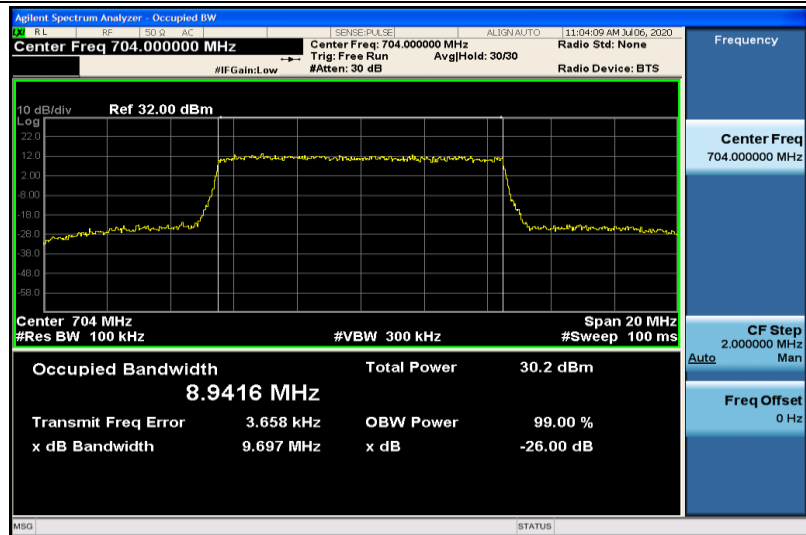
Band12-10MHz-16QAM-23060-50RB#0-8.9416
