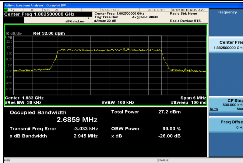
Band25-3MHz-16QAM-26365-15RB#0-2.6859
