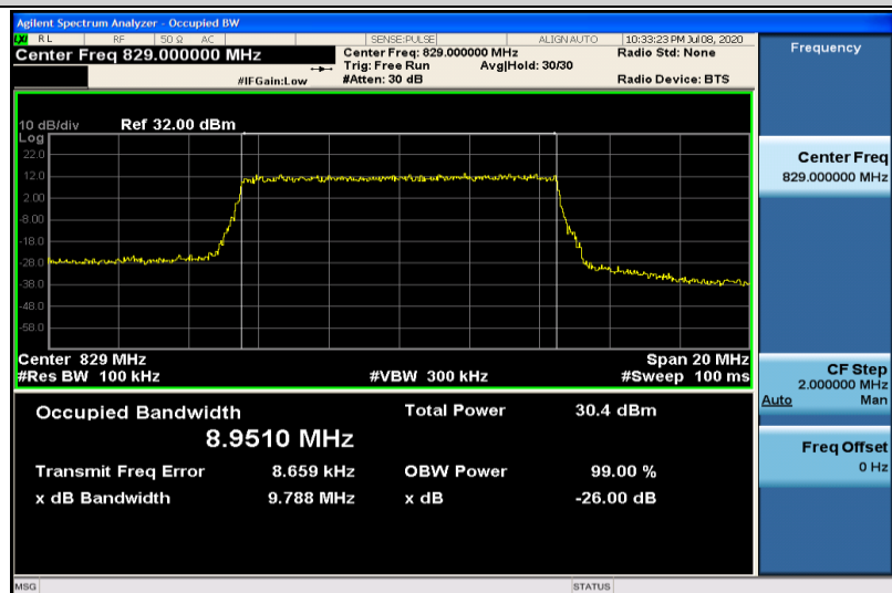
Band26-10MHz-QPSK-26840-50RB#0-8.9510
