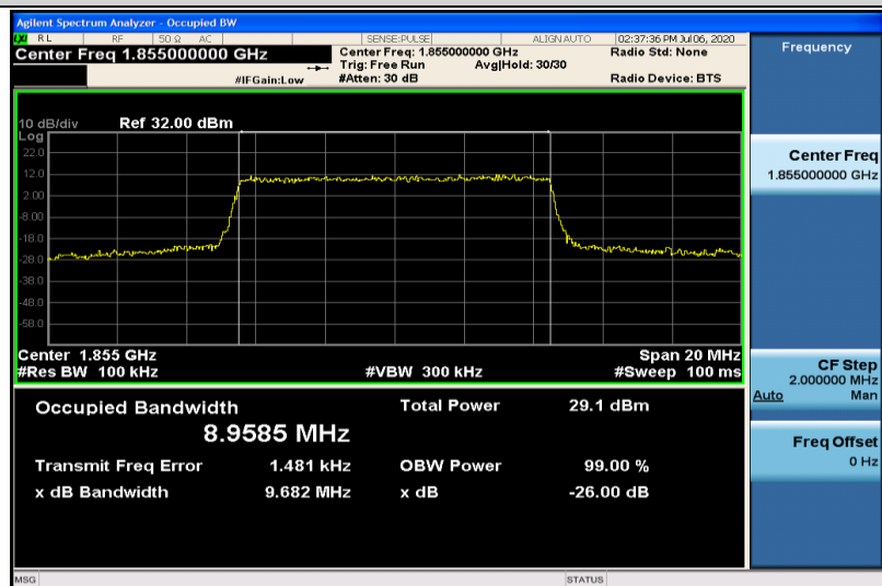
Band25-10MHz-QPSK-26090-50RB#0-8.9585
