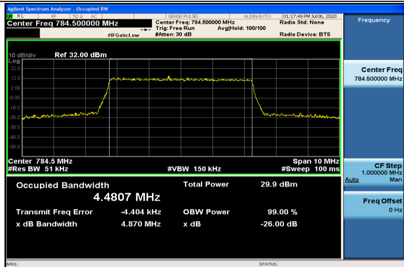
Band13-5MHz-16QAM-23255-25RB#0-4.4807
