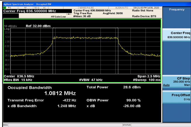
Band26-1.4MHz-16QAM-26915-6RB#0-1.0812
