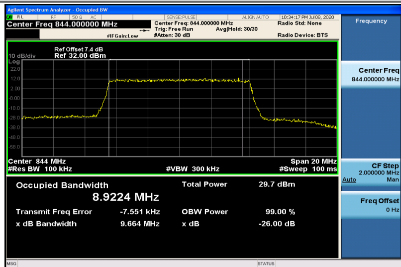
Band26-10MHz-16QAM-26990-50RB#0-8.9224
