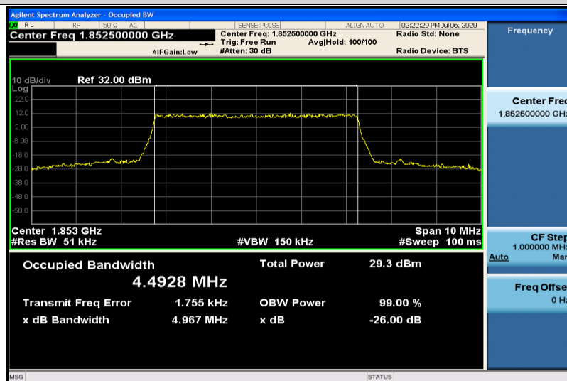
Band25-5MHz-QPSK-26065-25RB#0-4.4928
