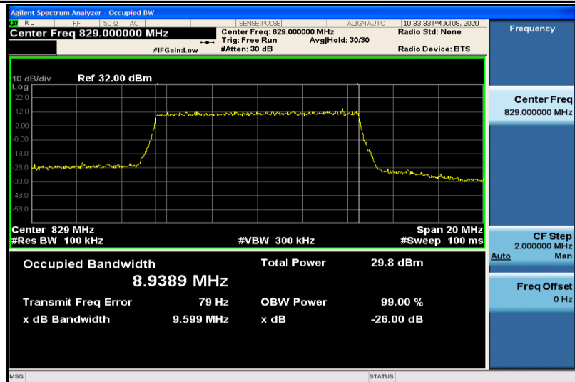
Band26-10MHz-16QAM-26840-50RB#0-8.9389
