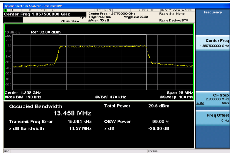
Band25-15MHz-QPSK-26115-75RB#0-13.458
