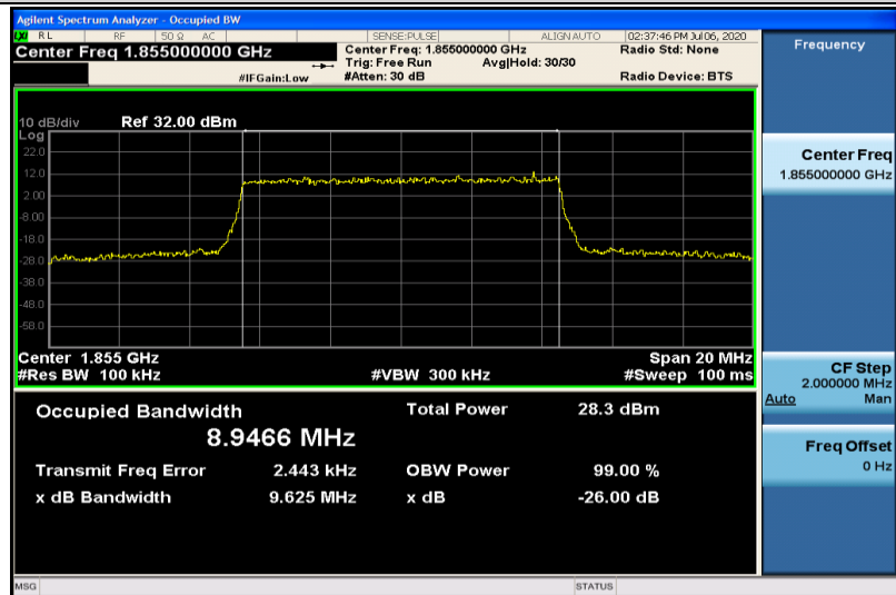
Band25-10MHz-16QAM-26090-50RB#0-8.9466
