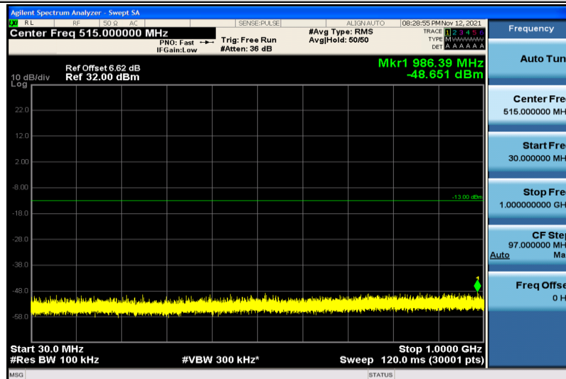
Band4-15MHz-QPSK-20175-1RB#0-30~1000MHz
