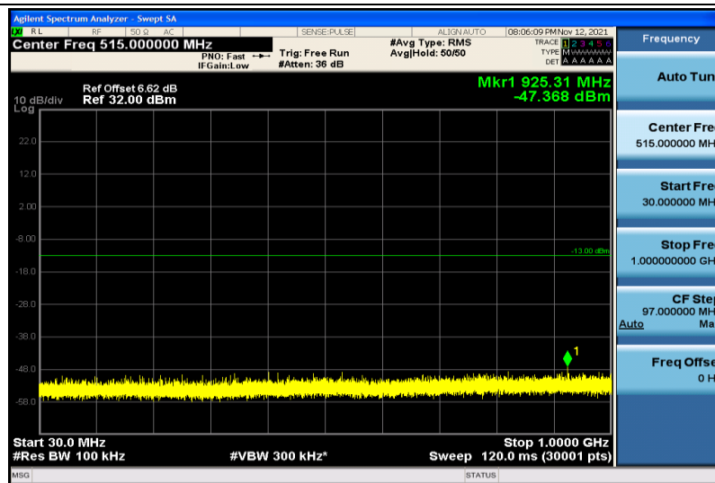
Band4-10MHz-16QAM-20000-1RB#0-30~1000MHz
