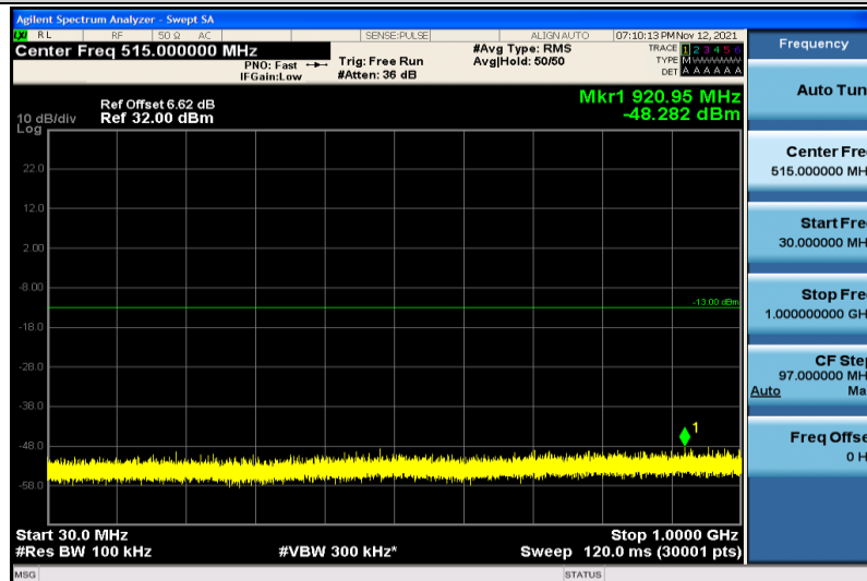
Band4-1.4MHz-16QAM-20175-1RB#0-30~1000MHz
