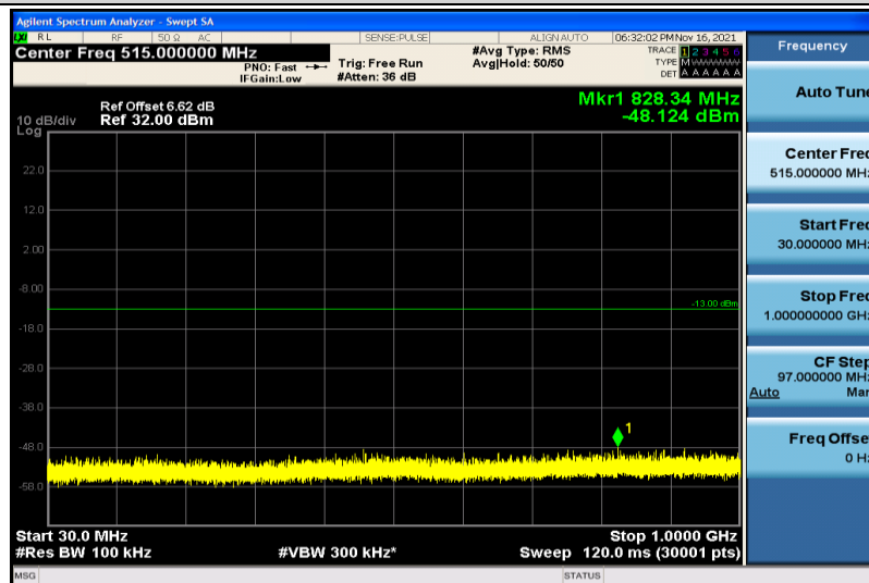
Band25-3MHz-16QAM-26055-1RB#0-30~1000MHz
