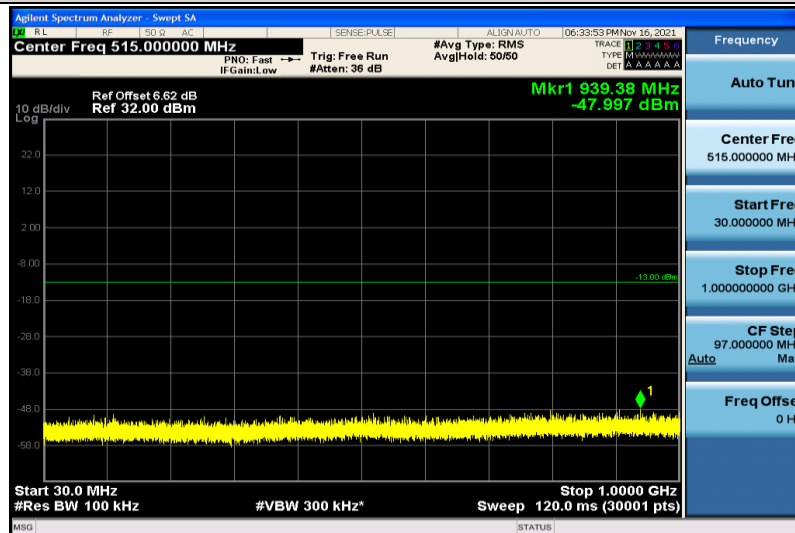
Band25-3MHz-QPSK-26675-1RB#0-30~1000MHz
