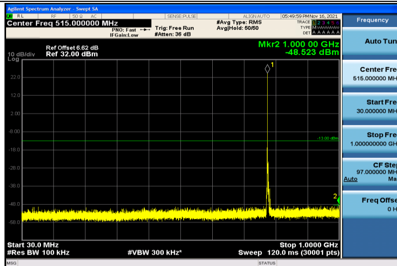
Band13-5MHz-16QAM-23230-1RB#0-30~1000MHz
