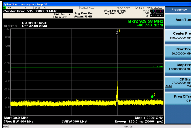
Band12-3MHz-16QAM-23095-1RB#0-30~1000MHz
