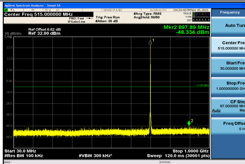
Band12-1.4MHz-16QAM-23095-1RB#0-30~1000MHz
