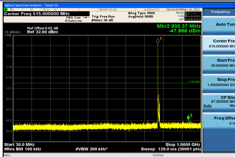
Band13-10MHz-16QAM-23230-1RB#0-30~1000MHz
