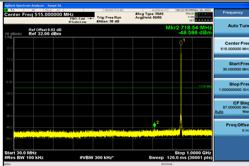
Band26-1.4MHz-16QAM-27033-1RB#0-30~1000MHz
