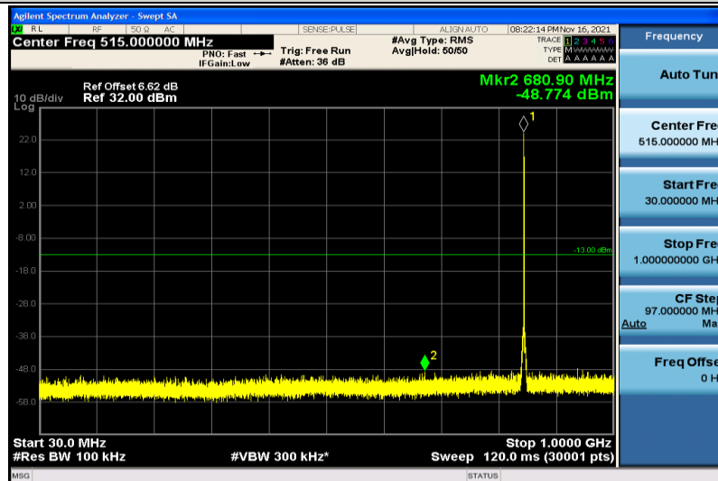
Band26-1.4MHz-QPSK-27033-1RB#0-30~1000MHz
