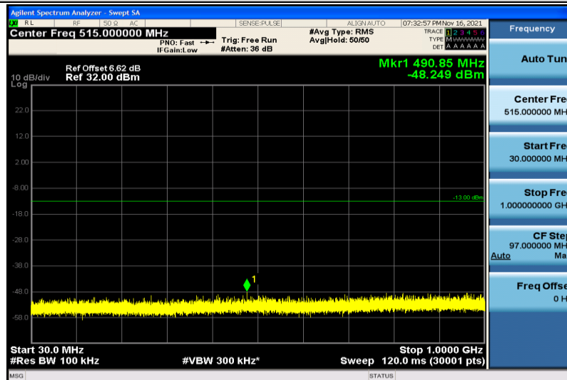
Band25-15MHz-16QAM-26615-1RB#0-30~1000MHz
