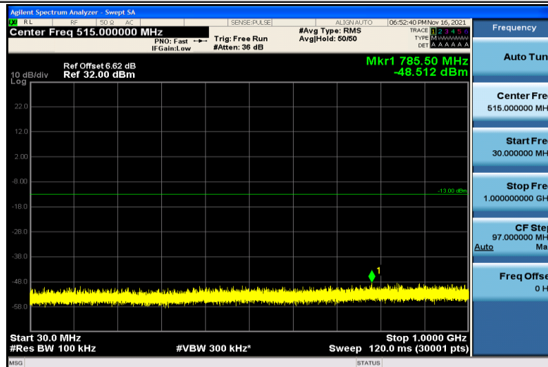
Band25-5MHz-QPSK-26665-1RB#0-30~1000MHz
