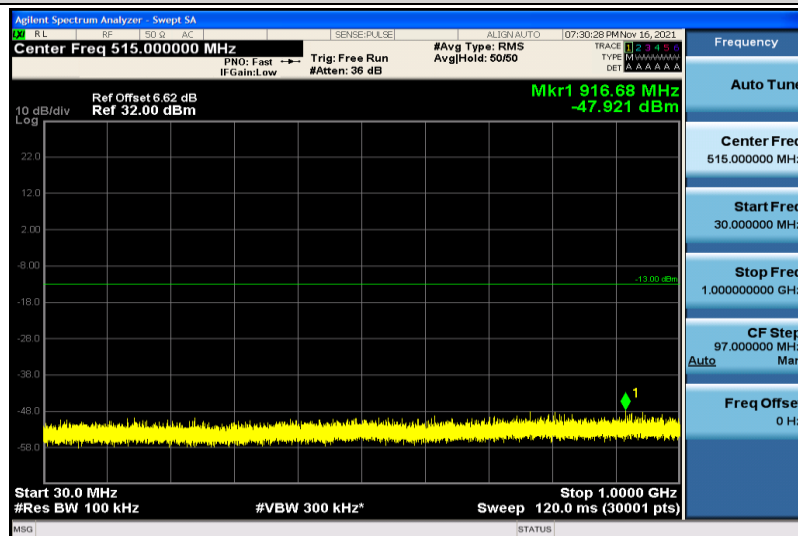
Band25-15MHz-16QAM-26115-1RB#0-30~1000MHz
