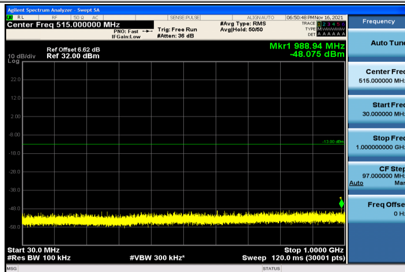
Band25-5MHz-16QAM-26065-1RB#0-30~1000MHz
