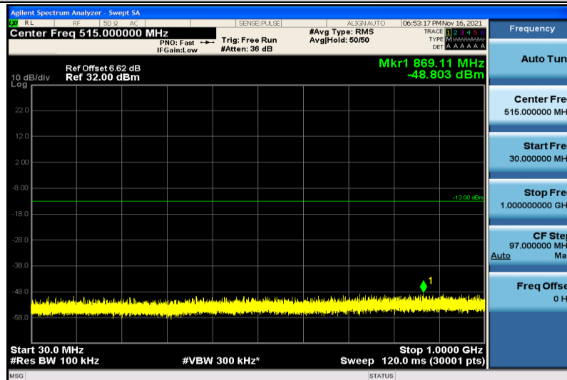
Band25-5MHz-16QAM-26665-1RB#0-30~1000MHz
