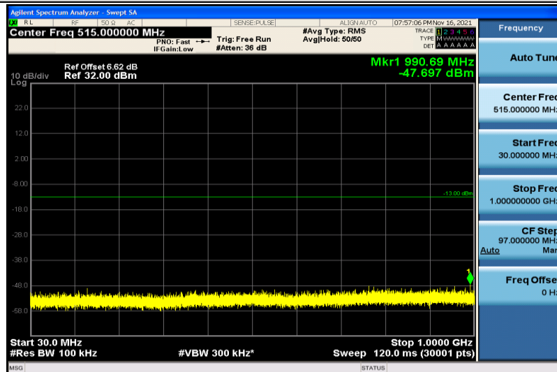
Band25-20MHz-16QAM-26590-1RB#0-30~1000MHz
