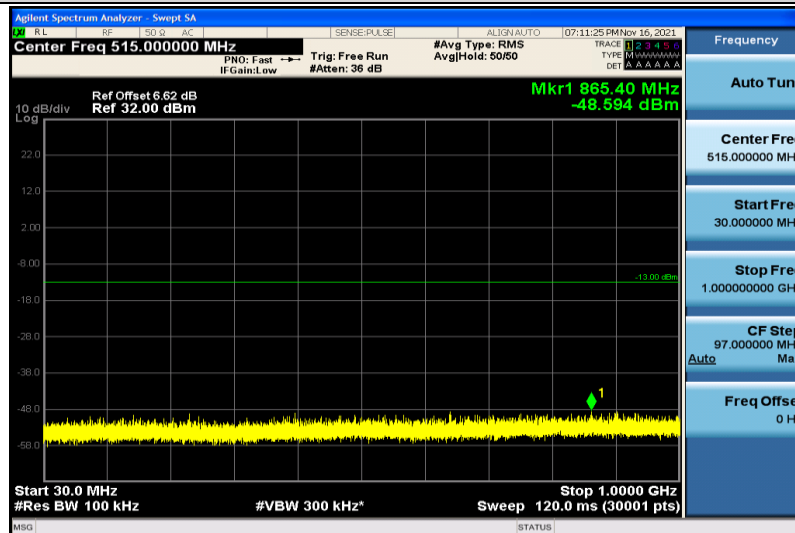
Band25-10MHz-QPSK-26640-1RB#0-30~1000MHz
