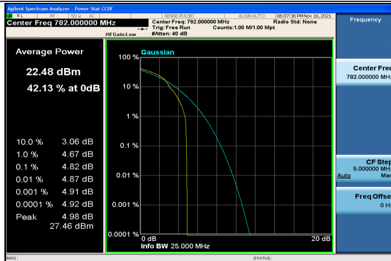
Band13-10MHz-16QAM-23230-1RB#0
