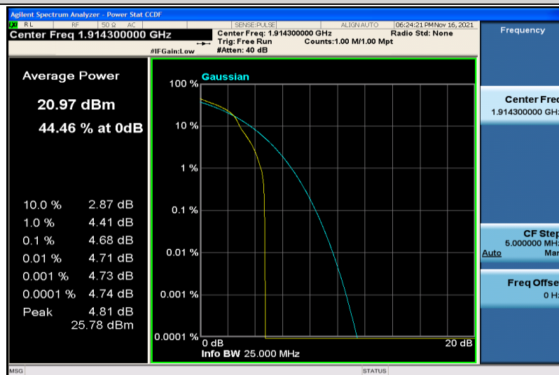
Band25-1.4MHz-16QAM-26683-1RB#0
