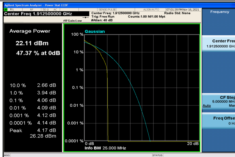
Band25-5MHz-QPSK-26665-1RB#0
