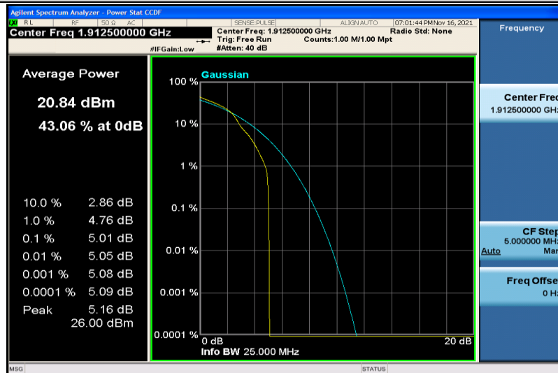
Band25-5MHz-16QAM-26665-1RB#0
