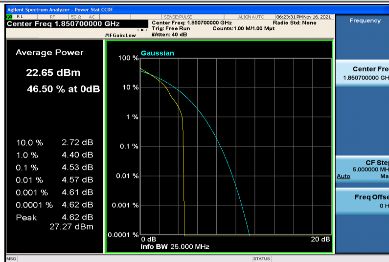
Band25-1.4MHz-QPSK-26047-1RB#0
