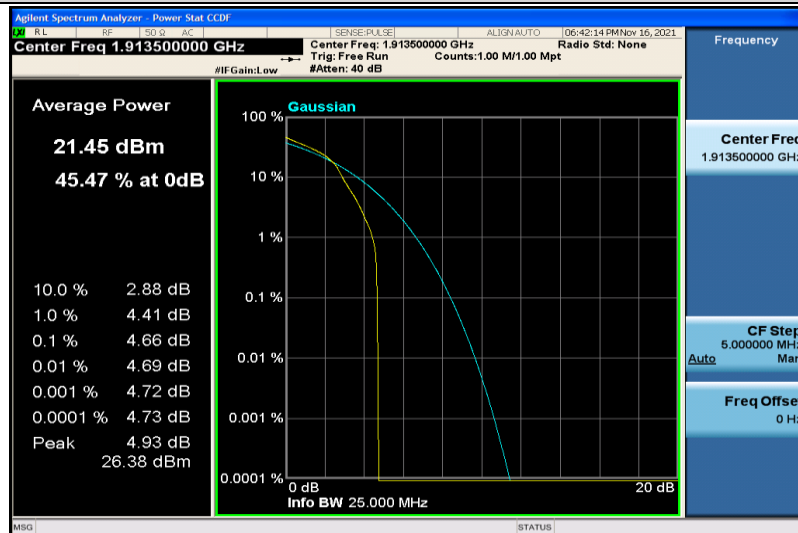
Band25-3MHz-16QAM-26675-1RB#0
