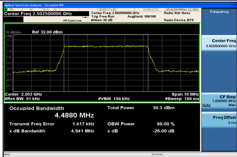
Band7-5MHz-QPSK-20775-25RB#0-4.4880
