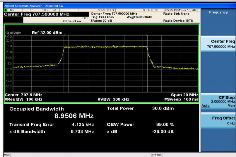
Band12-10MHz-QPSK-23095-50RB#0-8.9506
