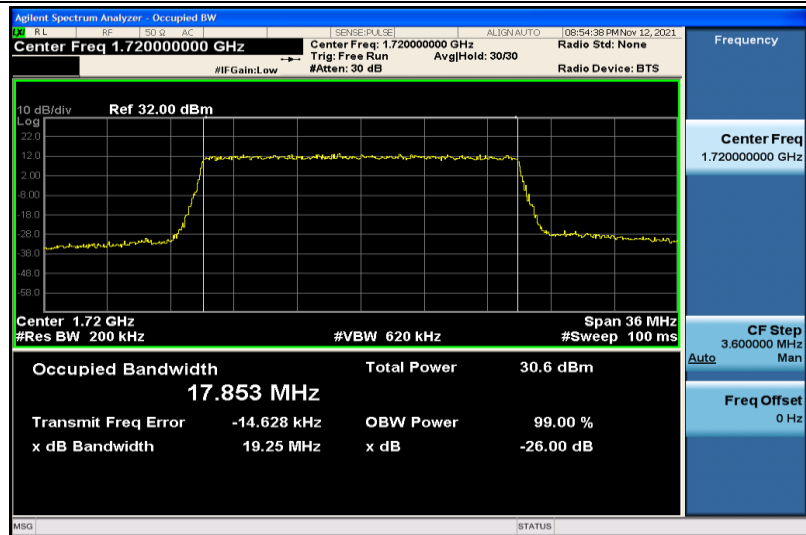
Band4-20MHz-QPSK-20050-100RB#0-17.853
