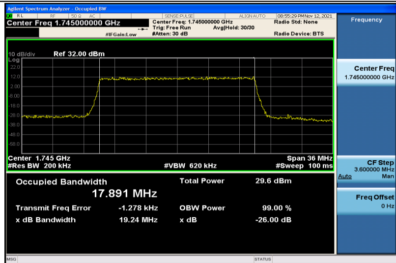
Band4-20MHz-16QAM-20300-100RB#0-17.891
