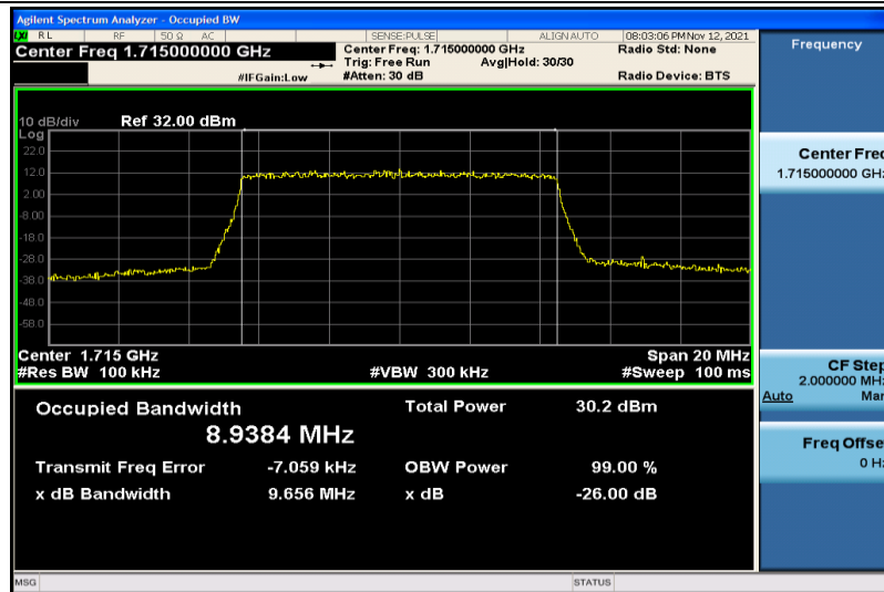
Band4-10MHz-QPSK-20000-50RB#0-8.9384
