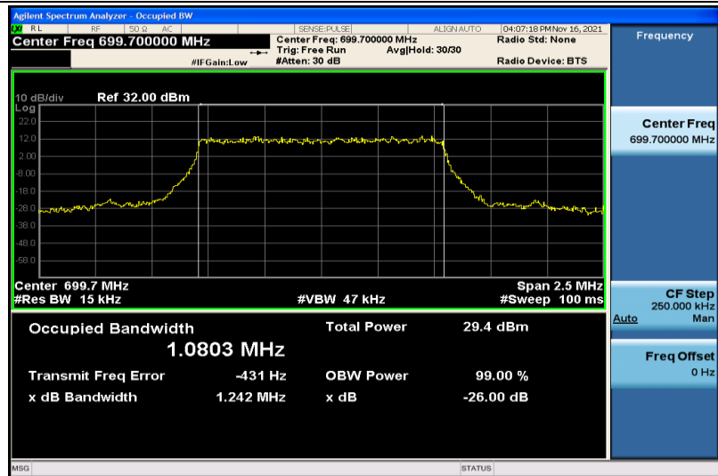
Band12-1.4MHz-QPSK-23017-6RB#0-1.0803
