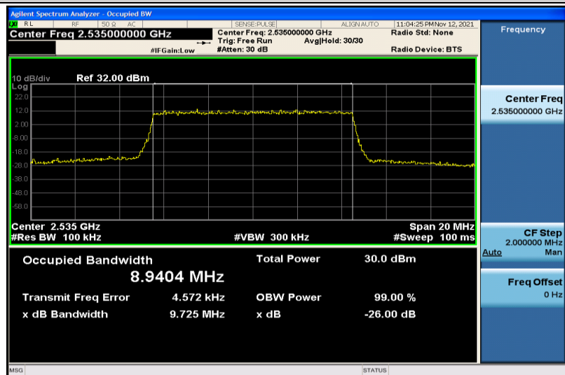
Band7-10MHz-16QAM-21100-50RB#0-8.9404
