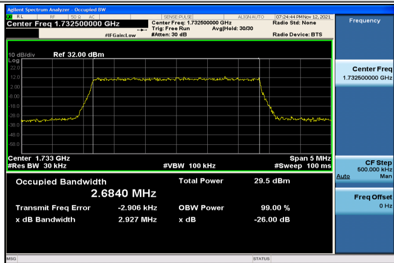
Band4-3MHz-QPSK-20175-15RB#0-2.6840
