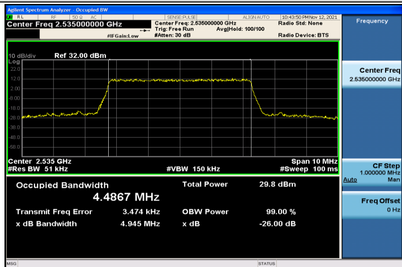
Band7-5MHz-16QAM-21100-25RB#0-4.4867
