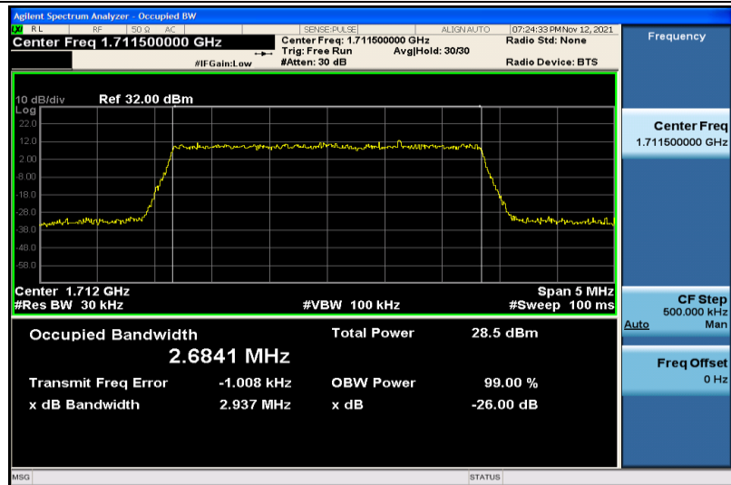
Band4-3MHz-16QAM-19965-15RB#0-2.6841
