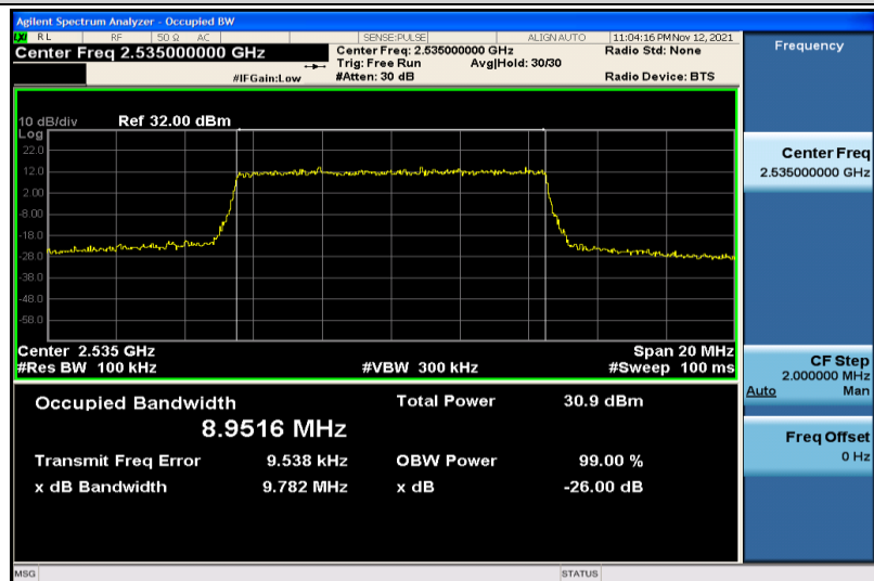
Band7-10MHz-QPSK-21100-50RB#0-8.9516
