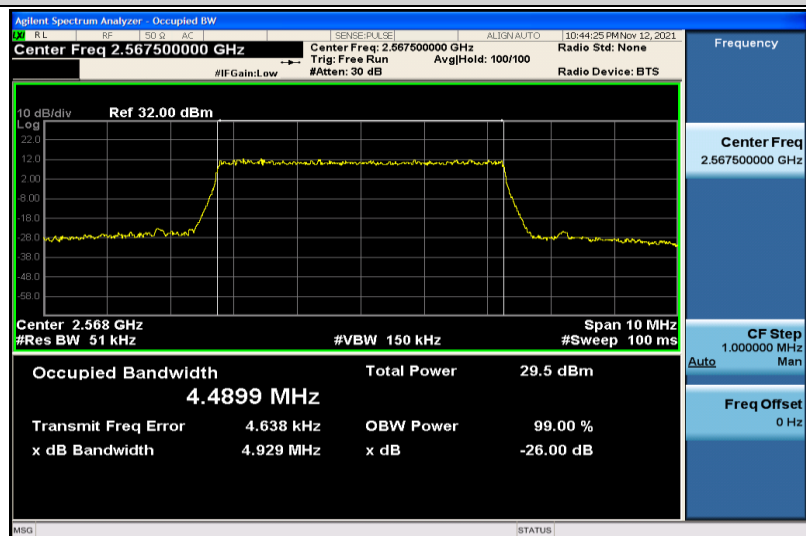
Band7-5MHz-16QAM-21425-25RB#0-4.4899
