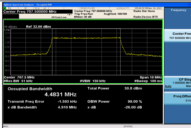
Band12-5MHz-QPSK-23095-25RB#0-4.4831
