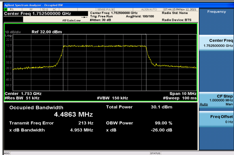
Band4-5MHz-QPSK-20375-25RB#0-4.4863
