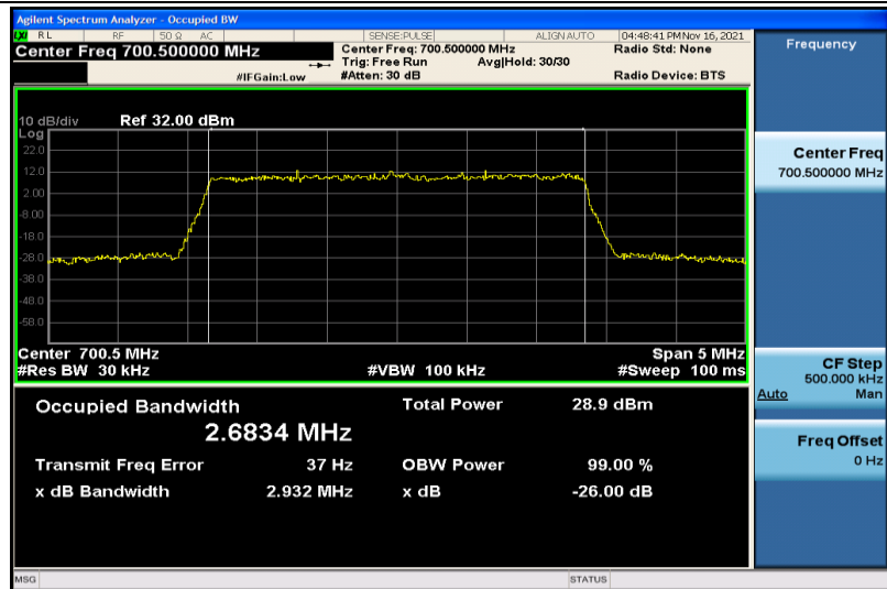
Band12-3MHz-16QAM-23025-15RB#0-2.6834
