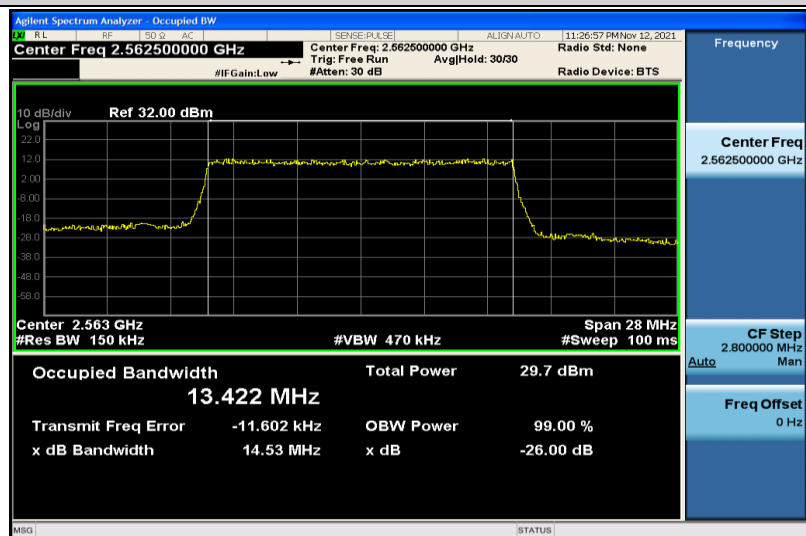
Band7-15MHz-16QAM-21375-75RB#0-13.422
