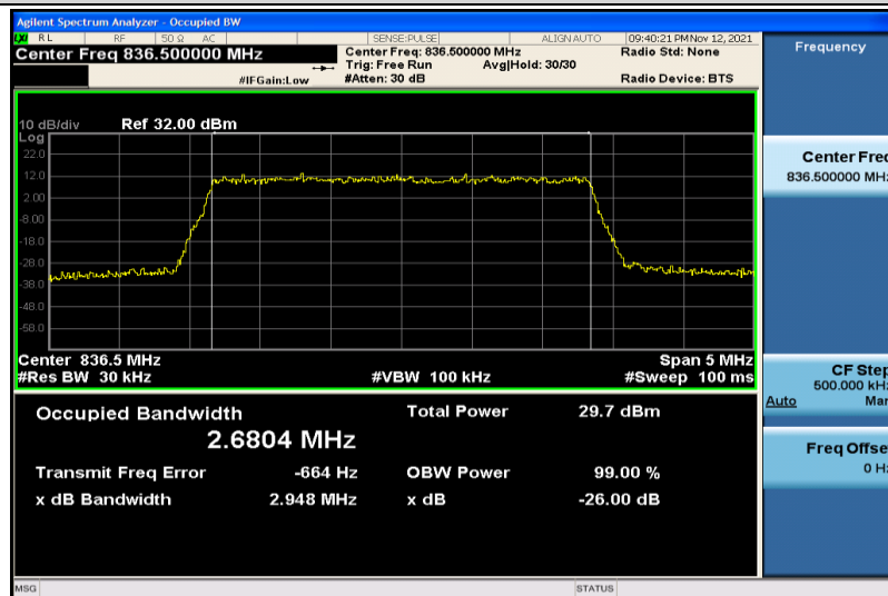
Band5-3MHz-16QAM-20525-15RB#0-2.6804
