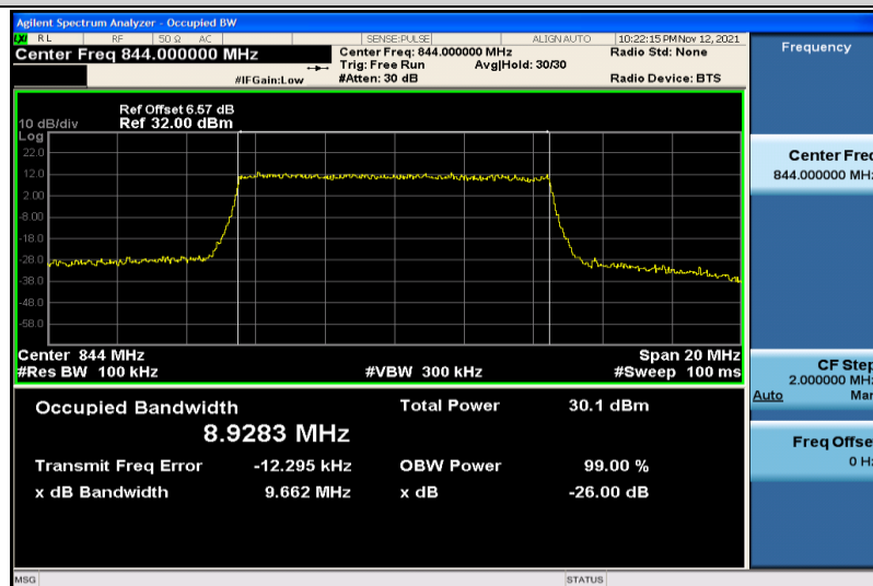
Band5-10MHz-16QAM-20600-50RB#0-8.9283
