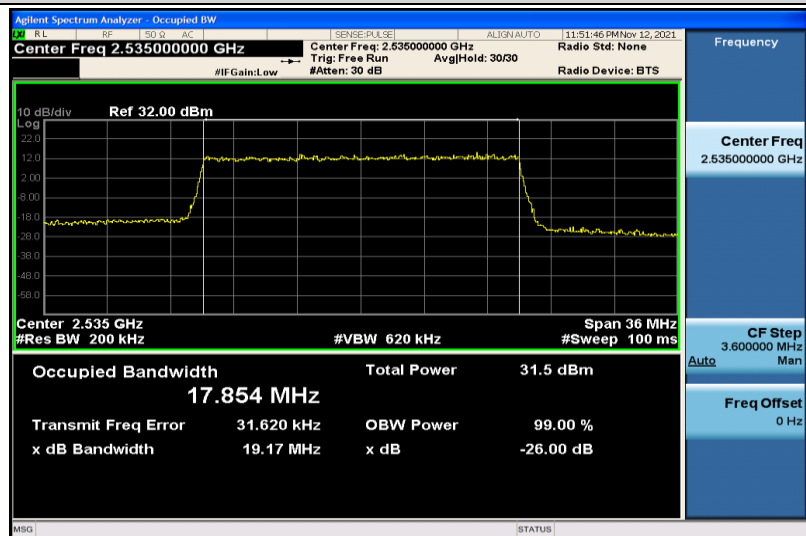
Band7-20MHz-QPSK-21100-100RB#0-17.854
