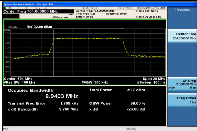
Band12-10MHz-QPSK-23060-50RB#0-8.9403
