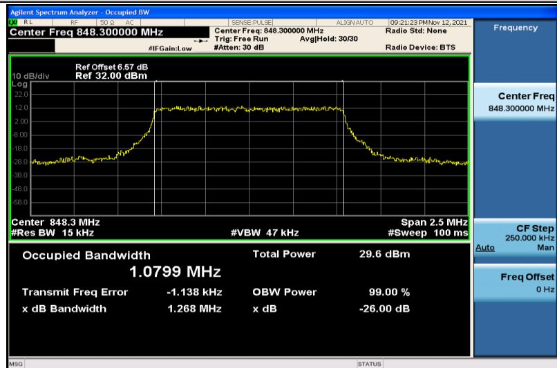
Band5-1.4MHz-QPSK-20643-6RB#0-1.0799
