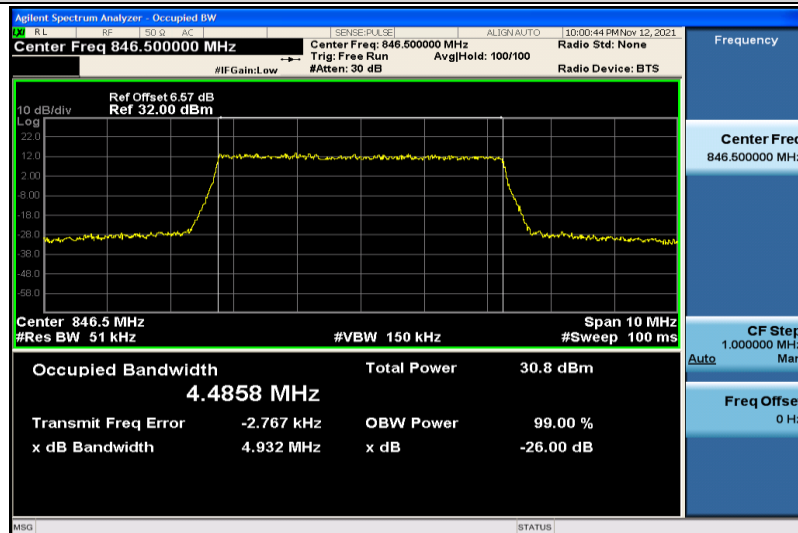
Band5-5MHz-QPSK-20625-25RB#0-4.4858
