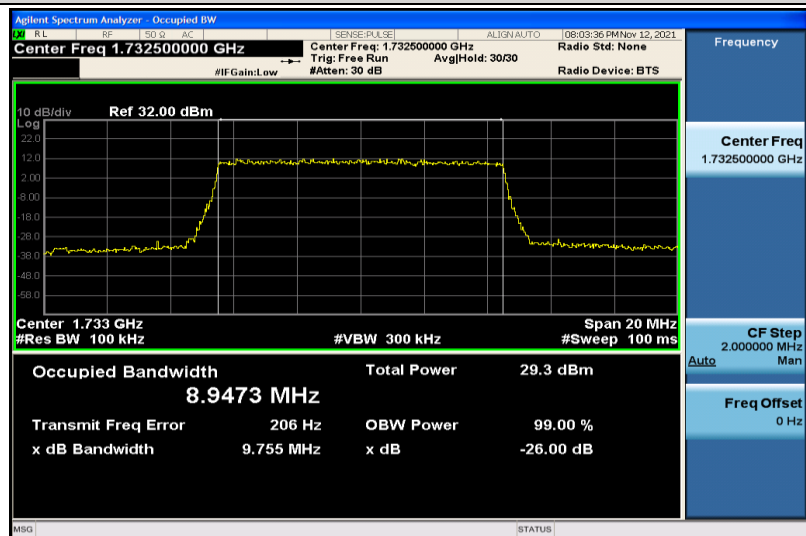
Band4-10MHz-16QAM-20175-50RB#0-8.9473
