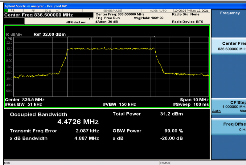
Band5-5MHz-QPSK-20525-25RB#0-4.4726
