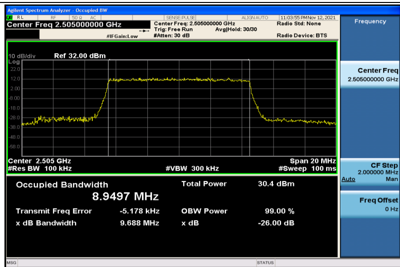
Band7-10MHz-QPSK-20800-50RB#0-8.9497
