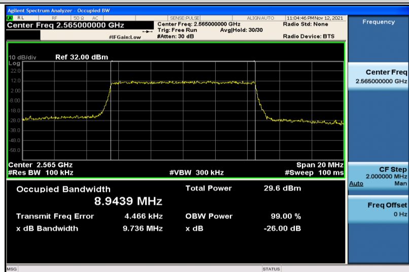
Band7-10MHz-16QAM-21400-50RB#0-8.9439
