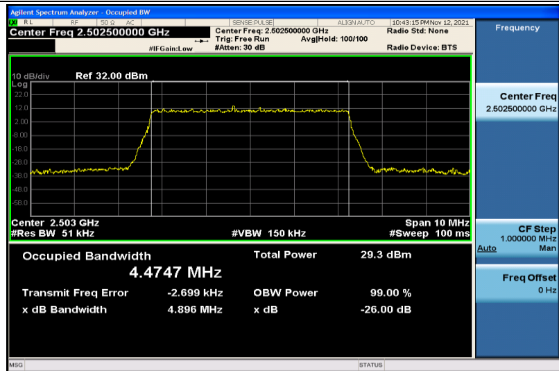
Band7-5MHz-16QAM-20775-25RB#0-4.4747
