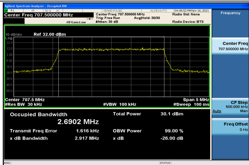
Band12-3MHz-QPSK-23095-15RB#0-2.6902
