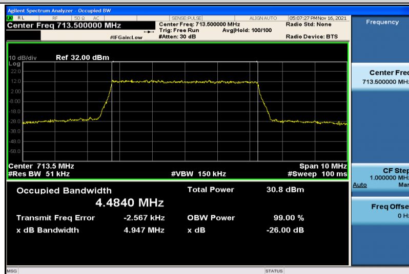
Band12-5MHz-QPSK-23155-25RB#0-4.4840
