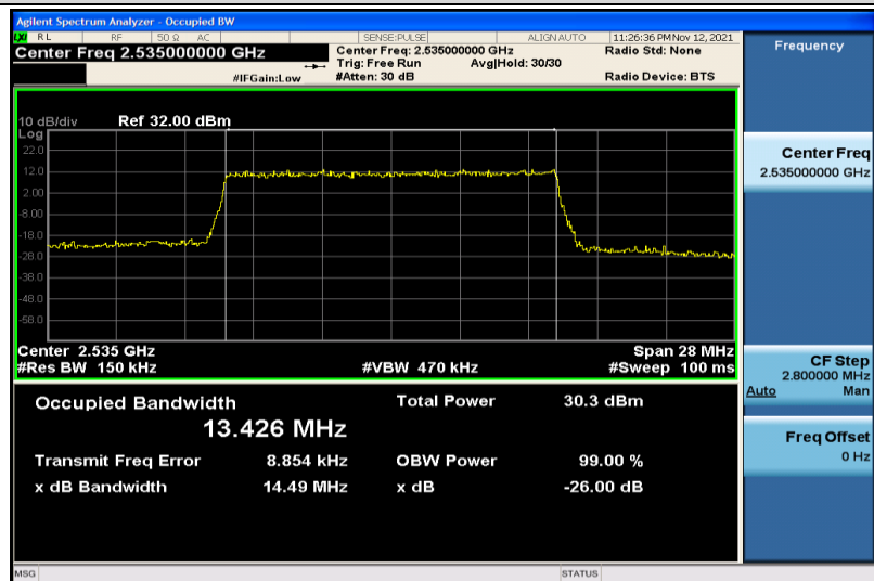
Band7-15MHz-16QAM-21100-75RB#0-13.426
