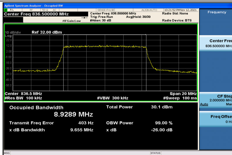
Band5-10MHz-16QAM-20525-50RB#0-8.9289
