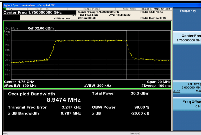
Band4-10MHz-QPSK-20350-50RB#0-8.9474
