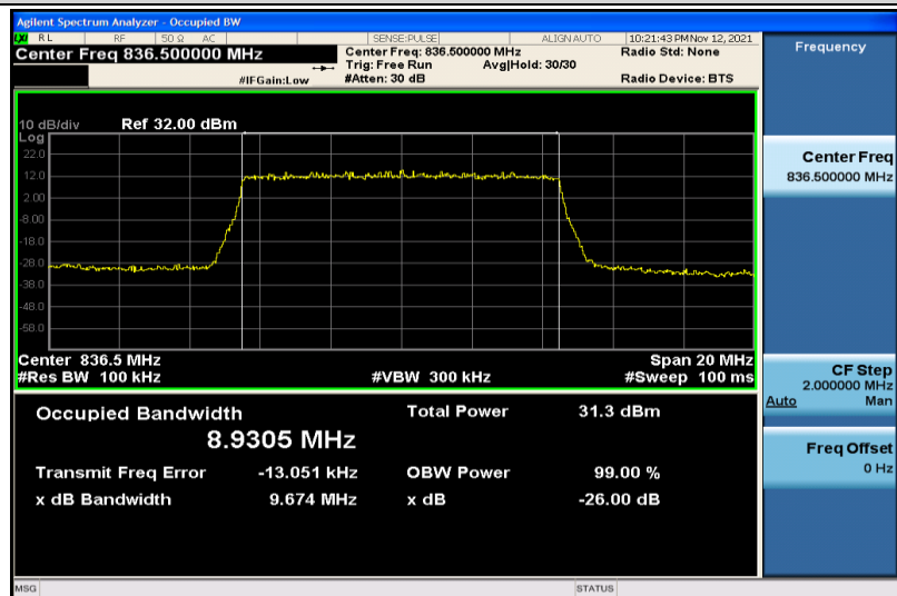
Band5-10MHz-QPSK-20525-50RB#0-8.9305
