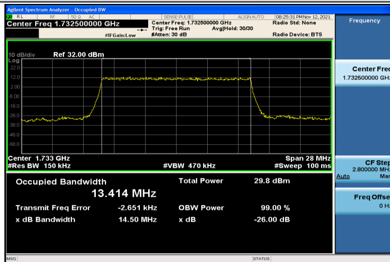
Band4-15MHz-QPSK-20175-75RB#0-13.414
