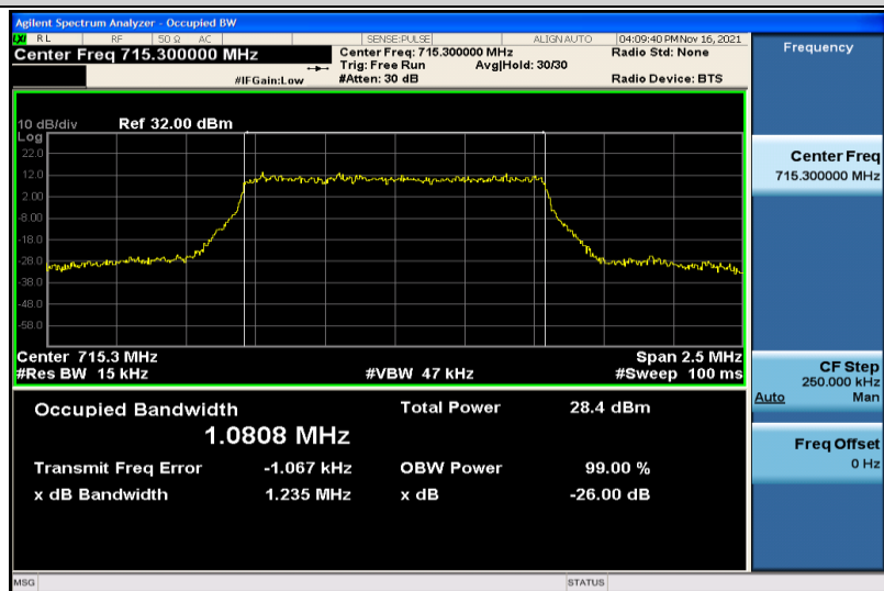
Band12-1.4MHz-16QAM-23173-6RB#0-1.0808
