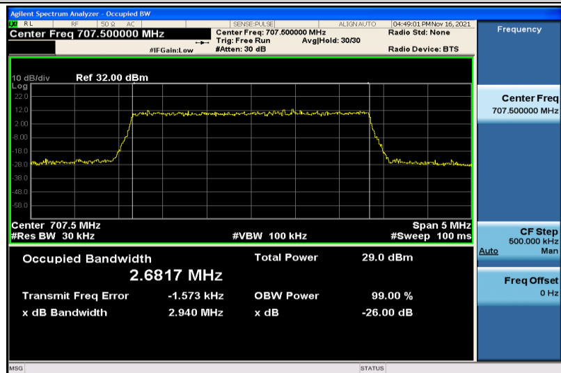
Band12-3MHz-16QAM-23095-15RB#0-2.6817
