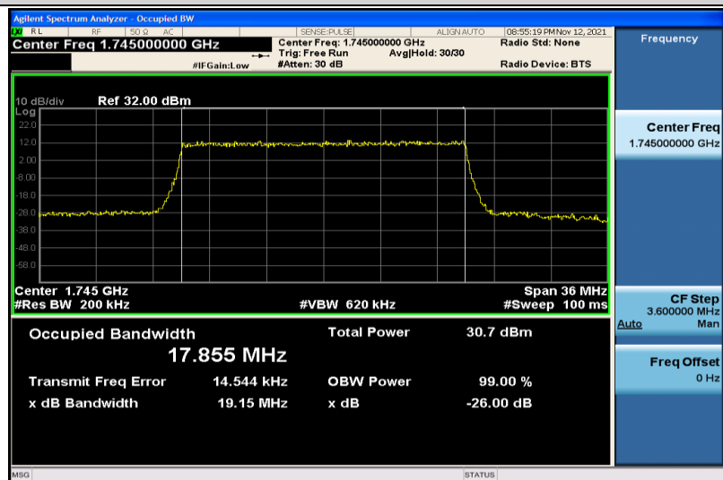
Band4-20MHz-QPSK-20300-100RB#0-17.855
