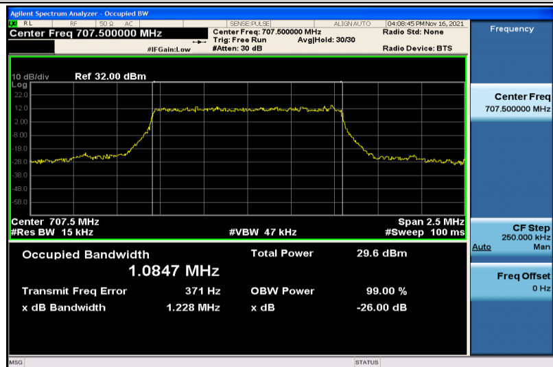
Band12-1.4MHz-QPSK-23095-6RB#0-1.0847
