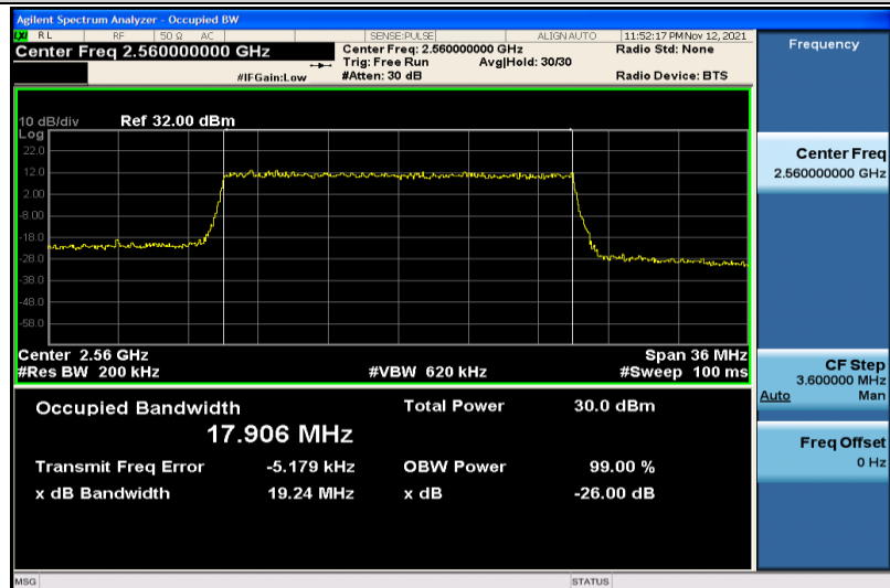
Band7-20MHz-16QAM-21350-100RB#0-17.906
