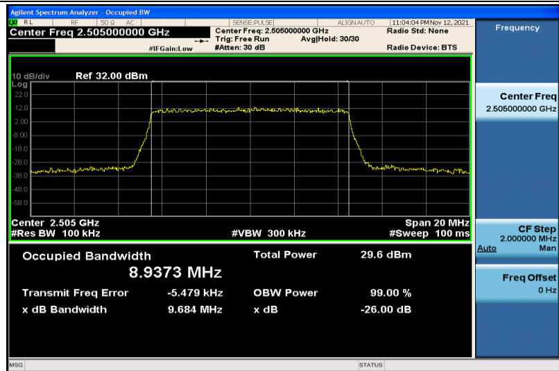
Band7-10MHz-16QAM-20800-50RB#0-8.9373
