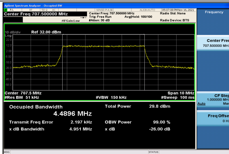
Band12-5MHz-16QAM-23095-25RB#0-4.4896
