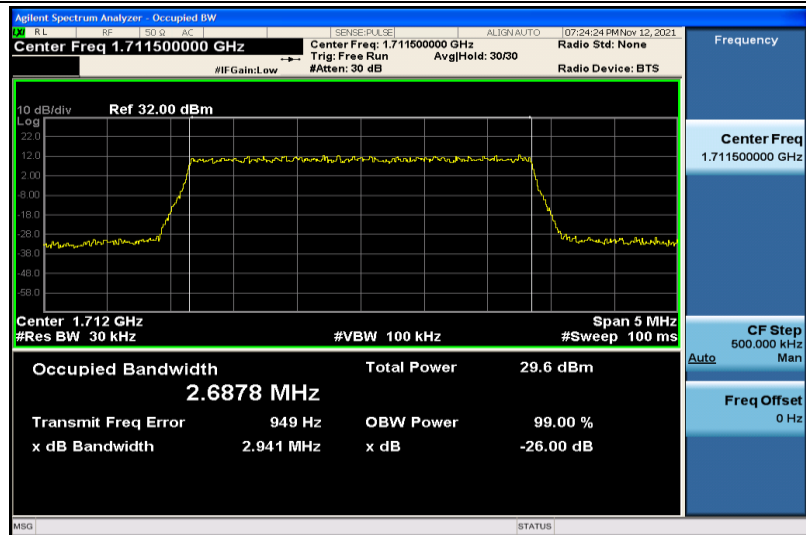
Band4-3MHz-QPSK-19965-15RB#0-2.6878
