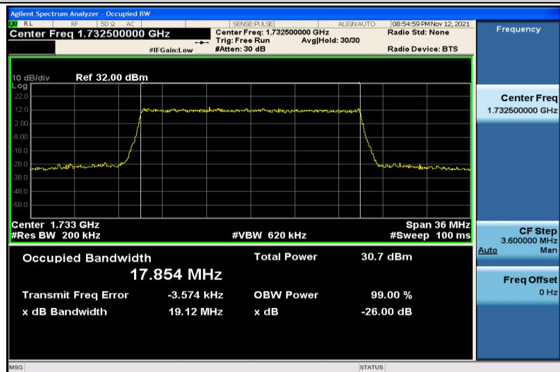
Band4-20MHz-QPSK-20175-100RB#0-17.854
