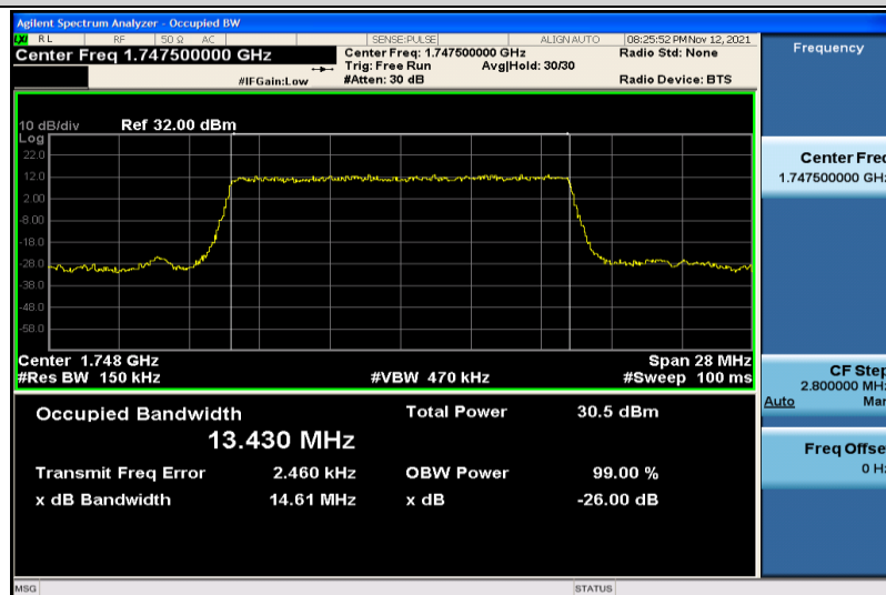
Band4-15MHz-QPSK-20325-75RB#0-13.430
