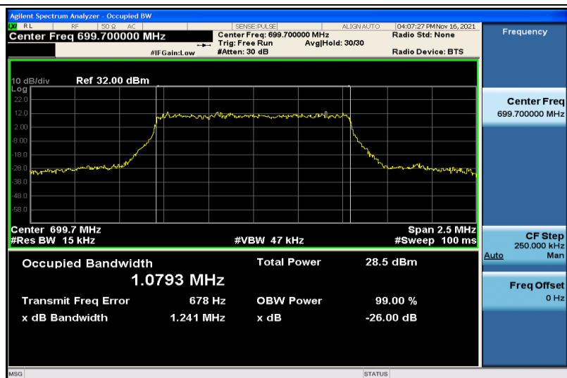
Band12-1.4MHz-16QAM-23017-6RB#0-1.0793
