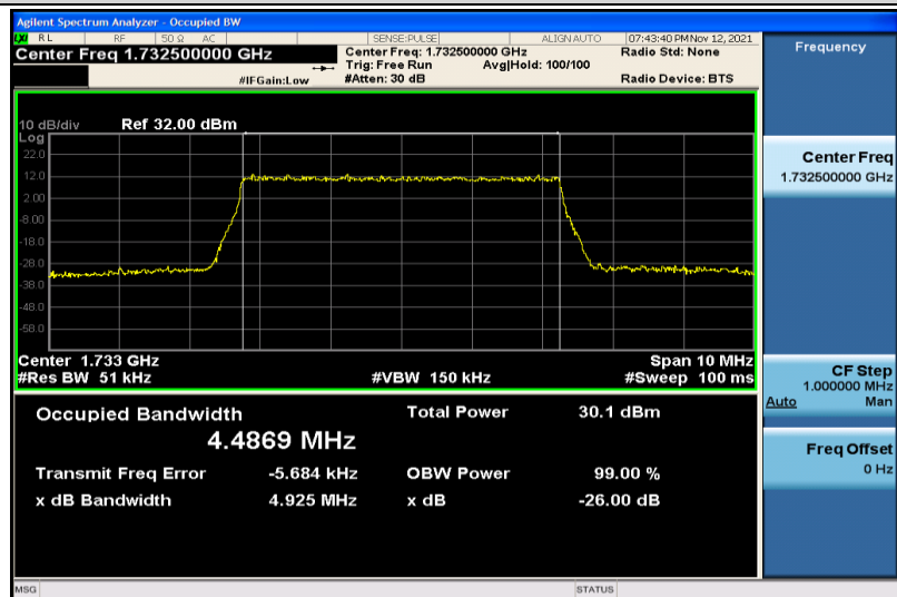
Band4-5MHz-QPSK-20175-25RB#0-4.4869
