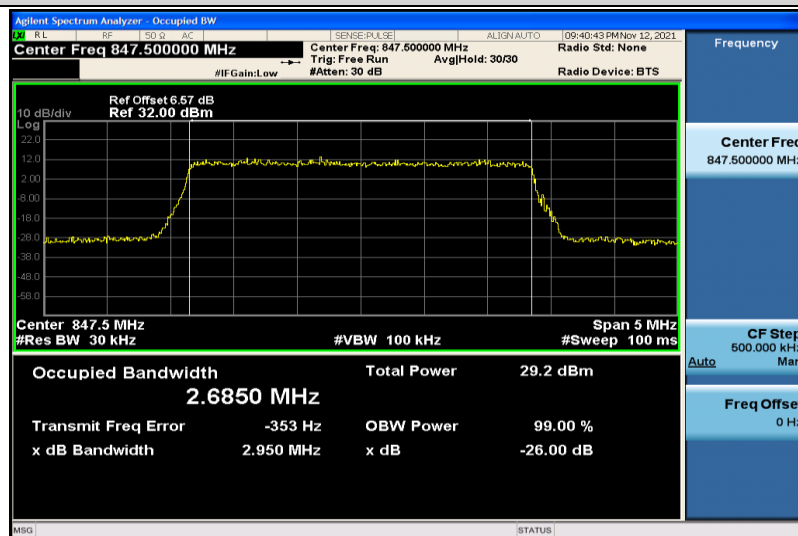
Band5-3MHz-16QAM-20635-15RB#0-2.6850
