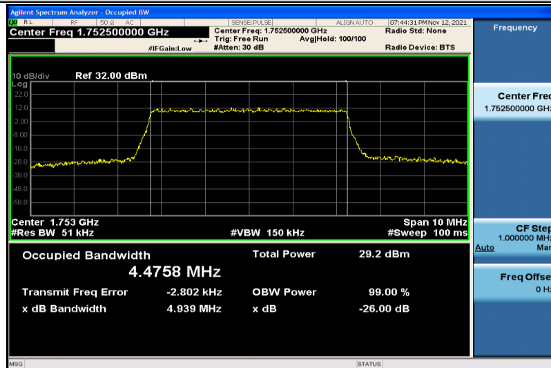
Band4-5MHz-16QAM-20375-25RB#0-4.4758
