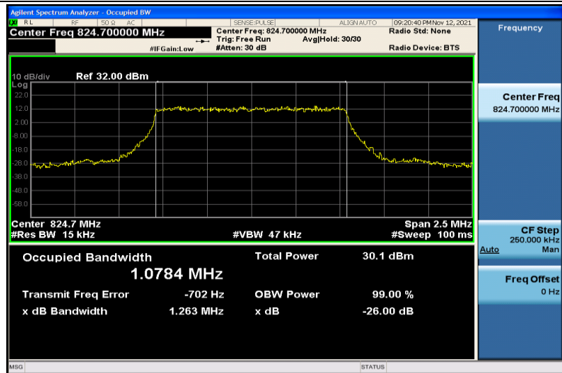
Band5-1.4MHz-QPSK-20407-6RB#0-1.0784
