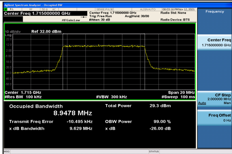
Band4-10MHz-16QAM-20000-50RB#0-8.9478
