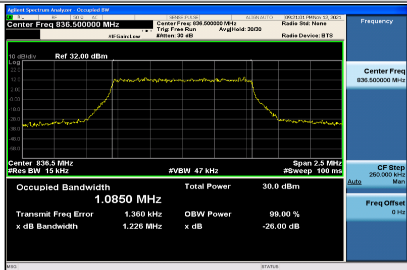
Band5-1.4MHz-QPSK-20525-6RB#0-1.0850
