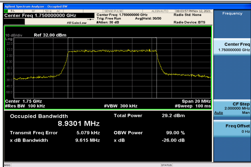
Band4-10MHz-16QAM-20350-50RB#0-8.9301
