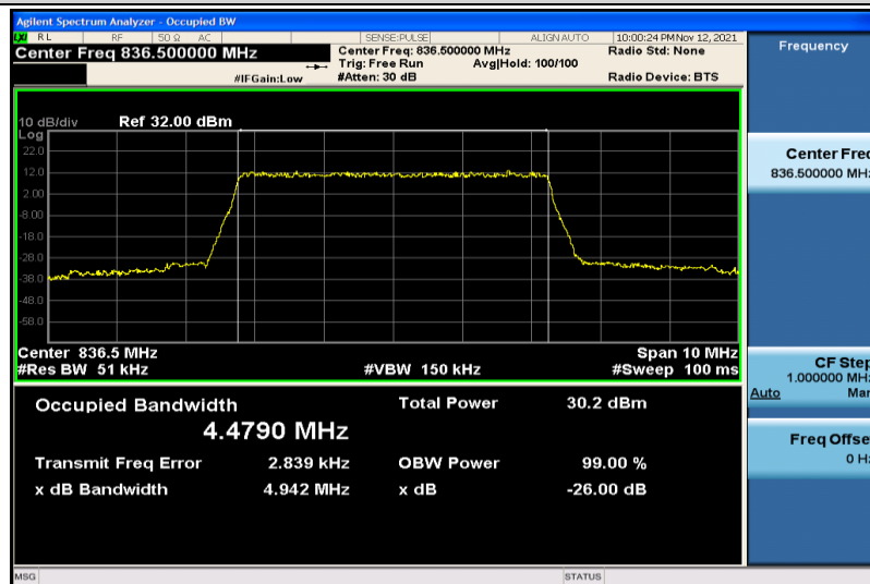
Band5-5MHz-16QAM-20525-25RB#0-4.4790
