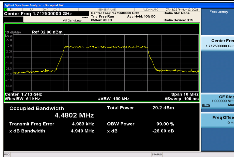
Band4-5MHz-16QAM-19975-25RB#0-4.4802
