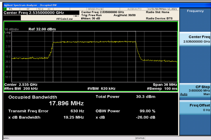
Band7-20MHz-16QAM-21100-100RB#0-17.896
