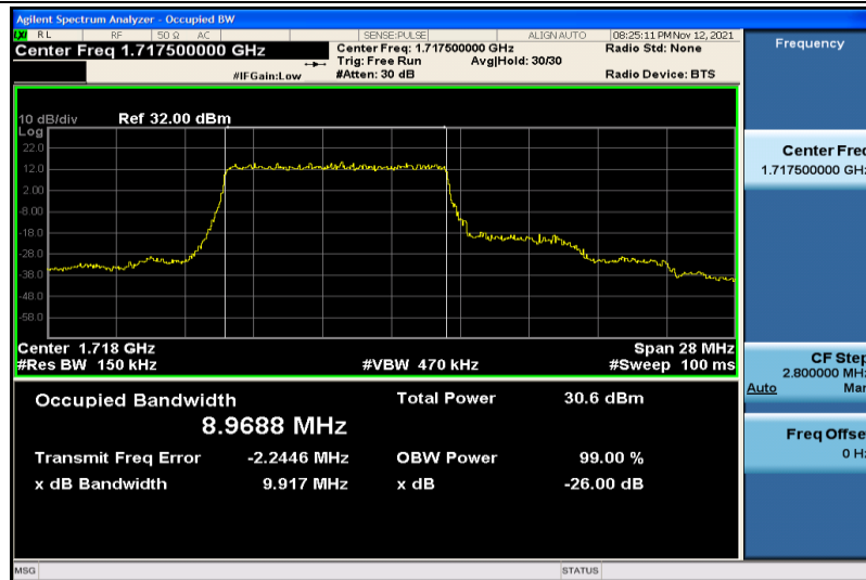
Band4-15MHz-QPSK-20025-75RB#0-8.9688
