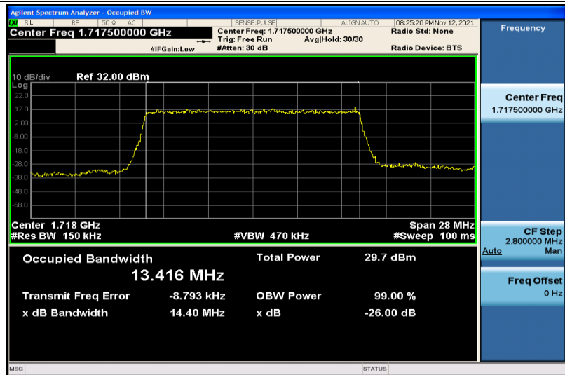
Band4-15MHz-16QAM-20025-75RB#0-13.416
