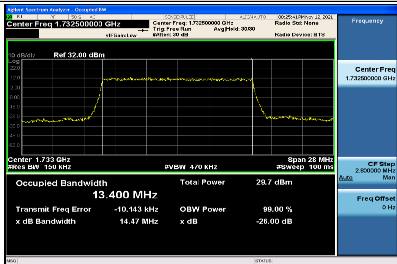
Band4-15MHz-16QAM-20175-75RB#0-13.400
