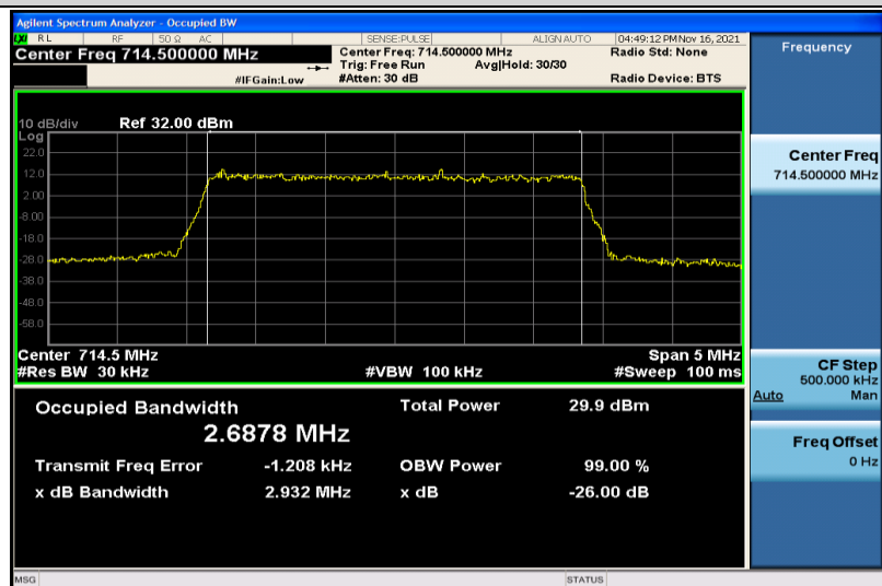
Band12-3MHz-QPSK-23165-15RB#0-2.6878
