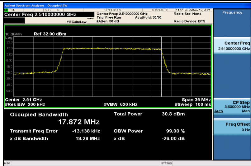
Band7-20MHz-QPSK-20850-100RB#0-17.872
