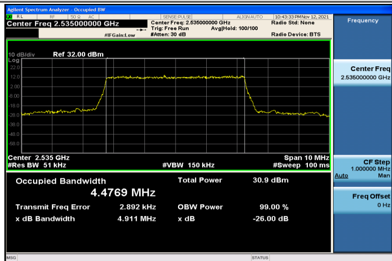
Band7-5MHz-QPSK-21100-25RB#0-4.4769
