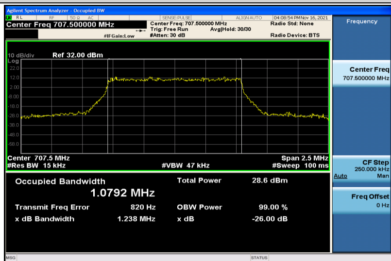
Band12-1.4MHz-16QAM-23095-6RB#0-1.0792
