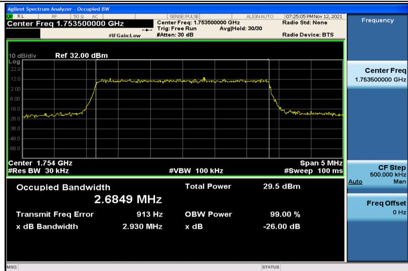
Band4-3MHz-QPSK-20385-15RB#0-2.6849
