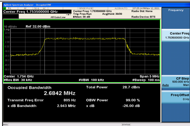
Band4-3MHz-16QAM-20385-15RB#0-2.6842
