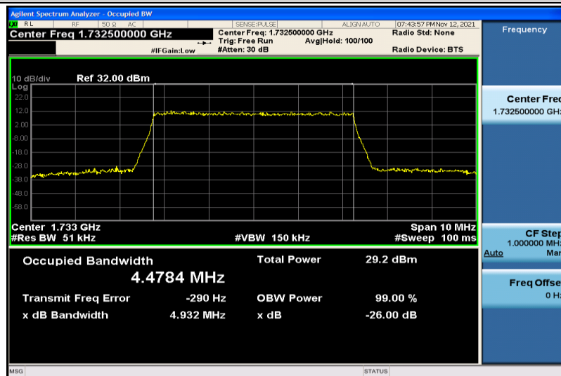
Band4-5MHz-16QAM-20175-25RB#0-4.4784
