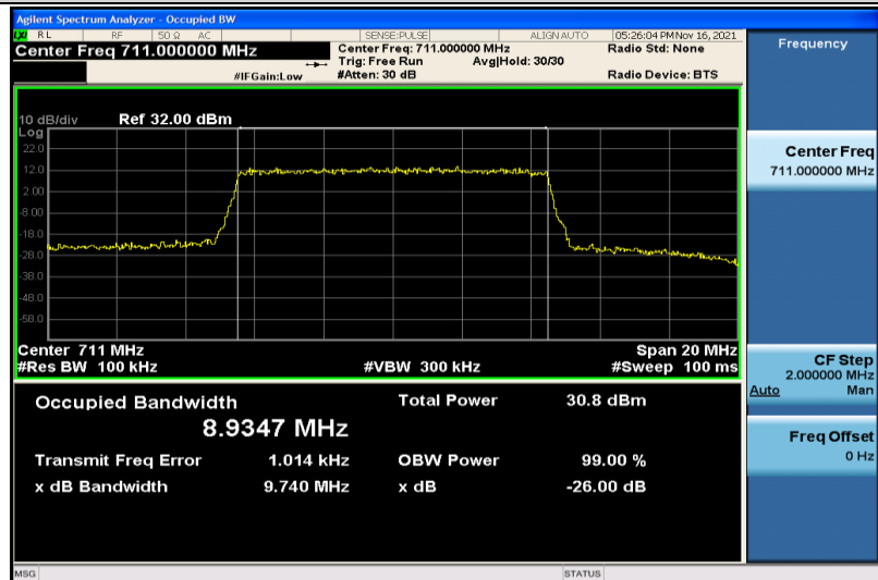
Band12-10MHz-QPSK-23130-50RB#0-8.9347
