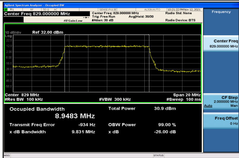
Band5-10MHz-QPSK-20450-50RB#0-8.9483
