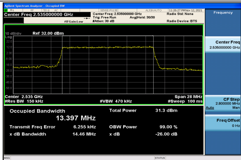
Band7-15MHz-QPSK-21100-75RB#0-13.397
