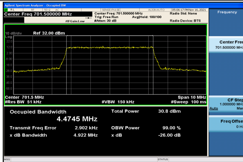
Band12-5MHz-QPSK-23035-25RB#0-4.4745
