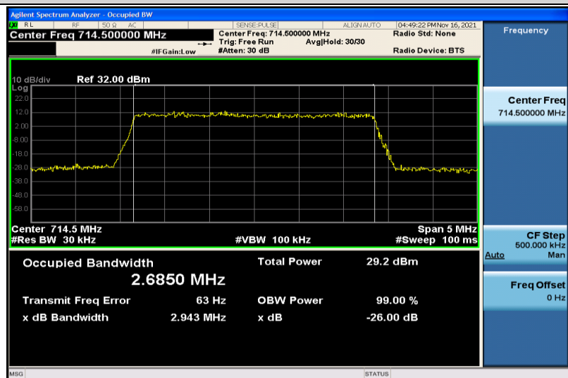
Band12-3MHz-16QAM-23165-15RB#0-2.6850
