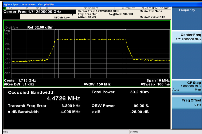
Band4-5MHz-QPSK-19975-25RB#0-4.4726
