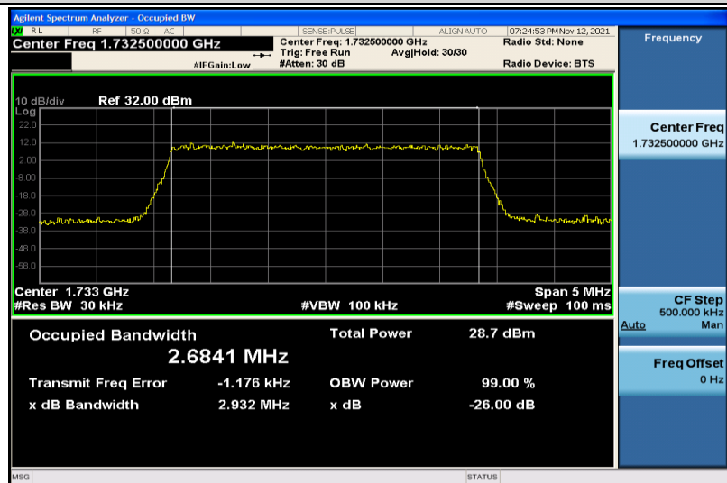
Band4-3MHz-16QAM-20175-15RB#0-2.6841
