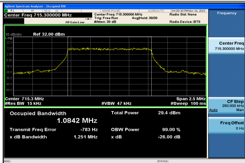
Band12-1.4MHz-QPSK-23173-6RB#0-1.0842
