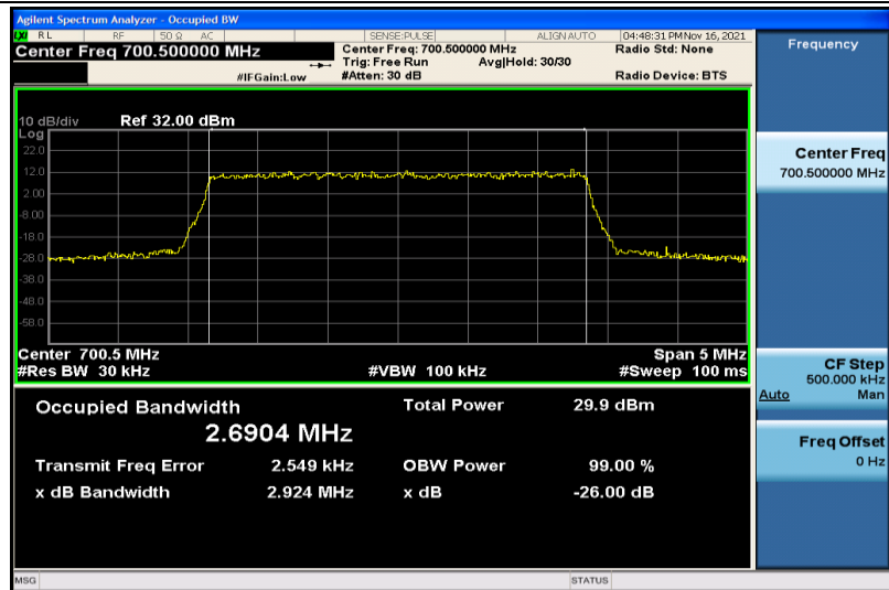
Band12-3MHz-QPSK-23025-15RB#0-2.6904
