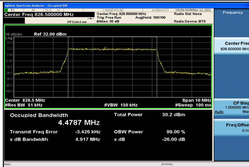
Band5-5MHz-16QAM-20425-25RB#0-4.4787
