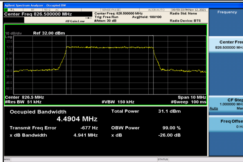
Band5-5MHz-QPSK-20425-25RB#0-4.4904
