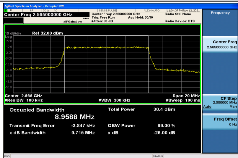
Band7-10MHz-QPSK-21400-50RB#0-8.9588
