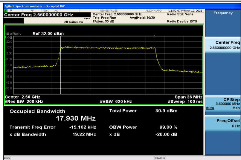
Band7-20MHz-QPSK-21350-100RB#0-17.930
