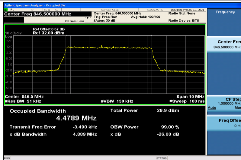
Band5-5MHz-16QAM-20625-25RB#0-4.4789
