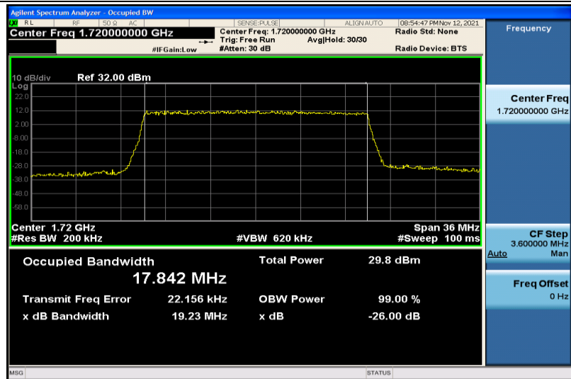
Band4-20MHz-16QAM-20050-100RB#0-17.842
