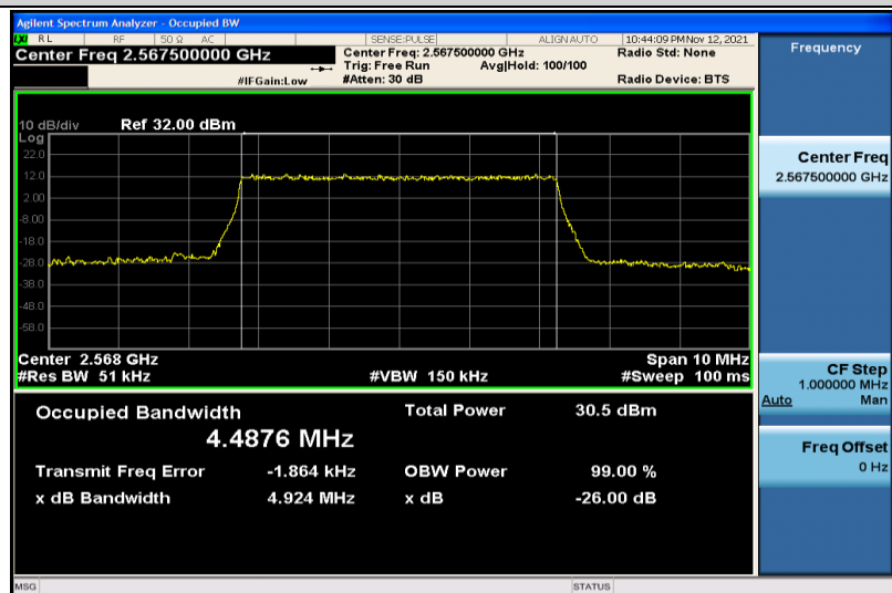
Band7-5MHz-QPSK-21425-25RB#0-4.4876
