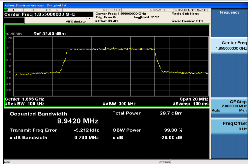
Band25-10MHz-16QAM-26090-50RB#0-8.9420
