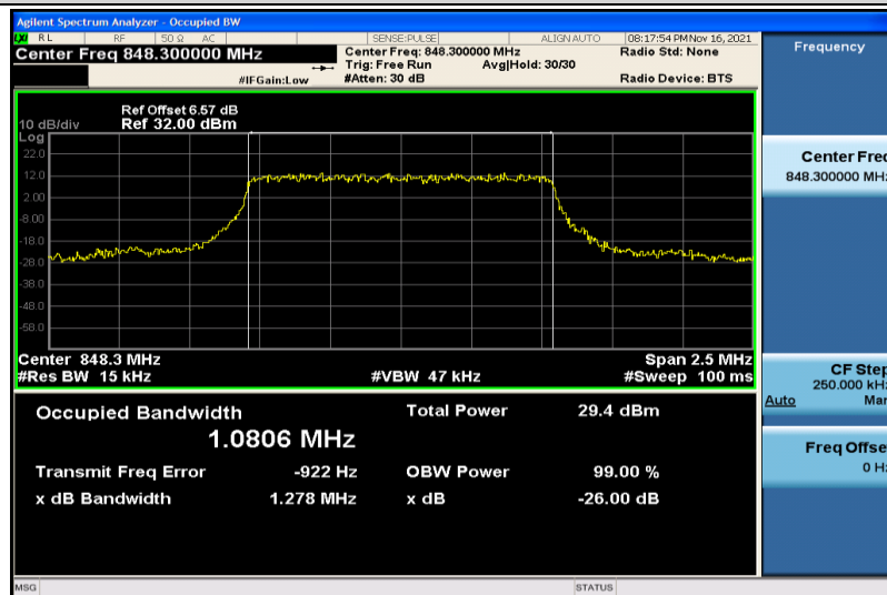
Band26-1.4MHz-QPSK-27033-6RB#0-1.0806
