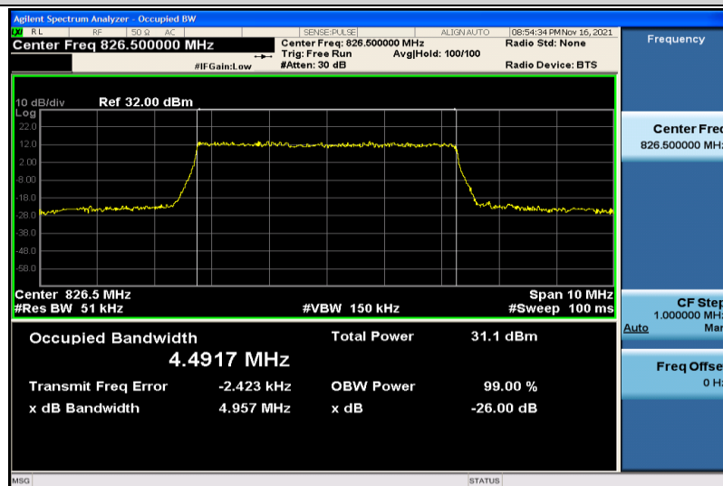
Band26-5MHz-QPSK-26815-25RB#0-4.4917
