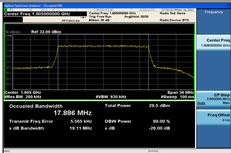
Band25-20MHz-16QAM-26590-100RB#0-17.886
