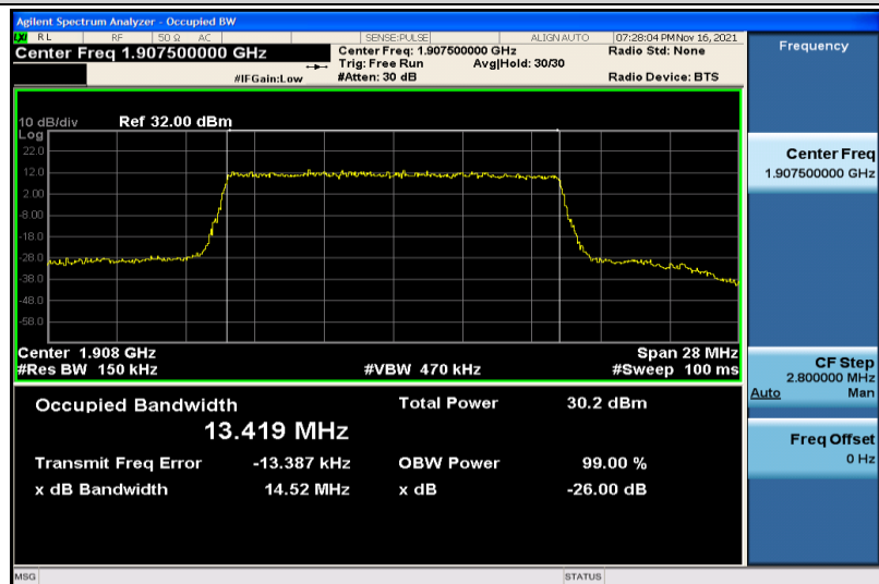
Band25-15MHz-QPSK-26615-75RB#0-13.419
