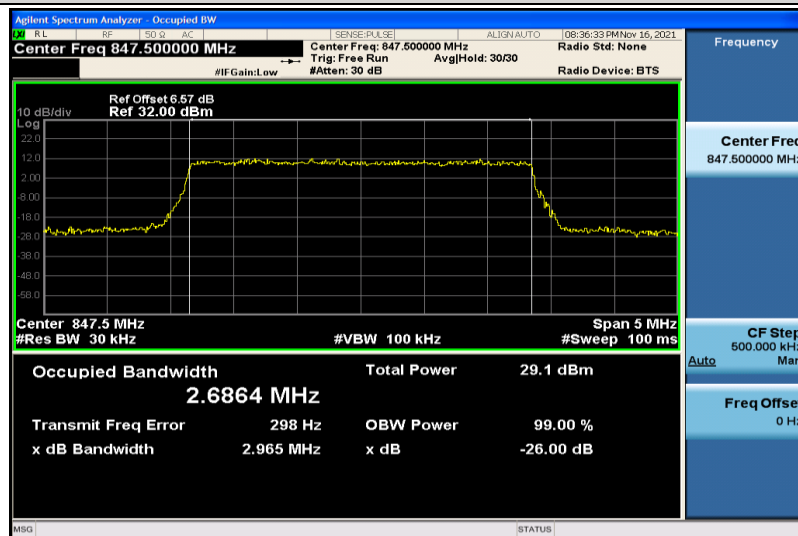
Band26-3MHz-16QAM-27025-15RB#0-2.6864
