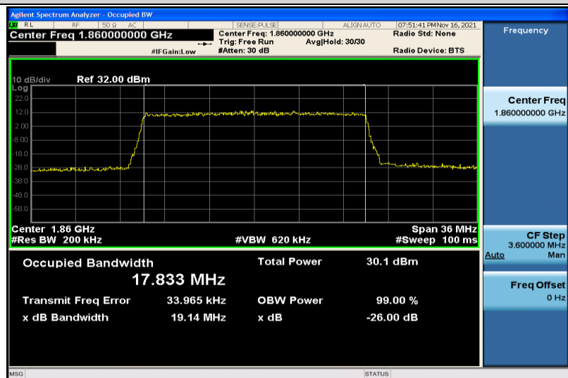
Band25-20MHz-16QAM-26140-100RB#0-17.833
