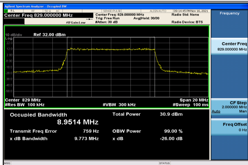
Band26-10MHz-QPSK-26840-50RB#0-8.9514
