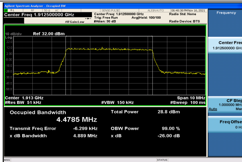
Band25-5MHz-16QAM-26665-25RB#0-4.4785
