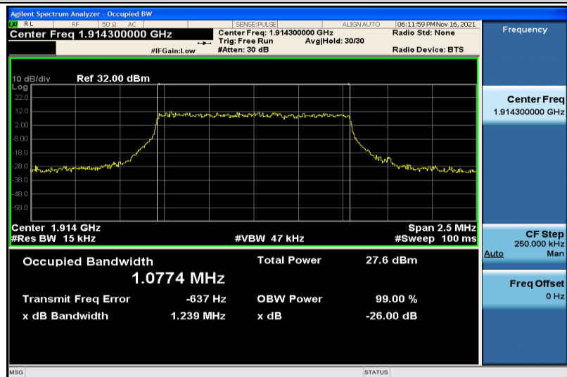
Band25-1.4MHz-16QAM-26683-6RB#0-1.0774
