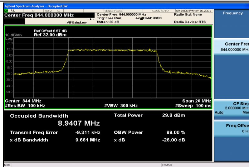
Band26-10MHz-16QAM-26990-50RB#0-8.9407
