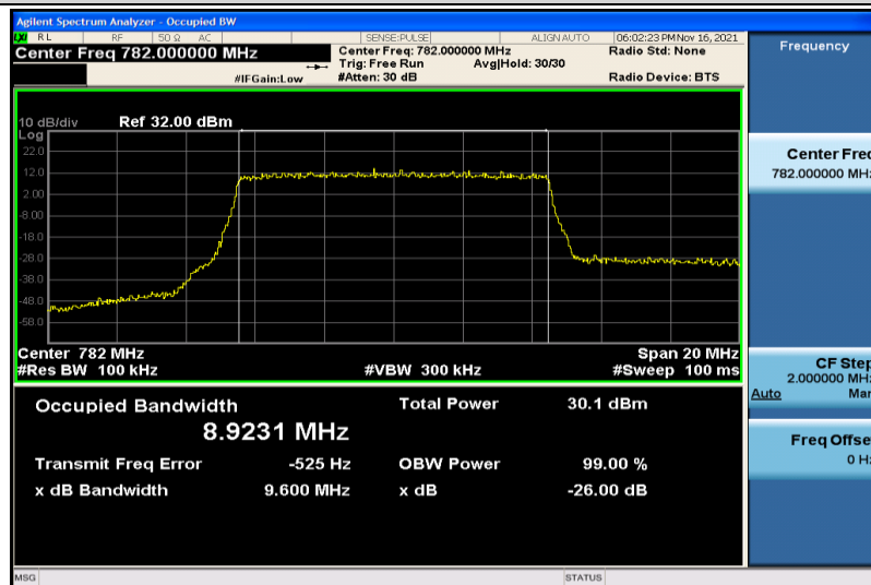
Band13-10MHz-16QAM-23230-50RB#0-8.9231
