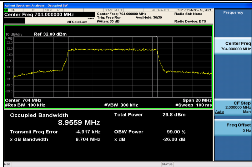
Band12-10MHz-16QAM-23060-50RB#0-8.9559
