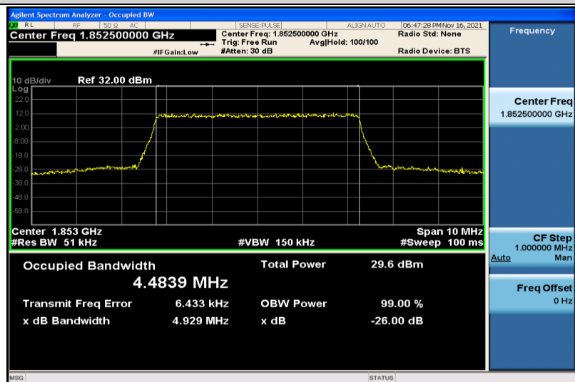
Band25-5MHz-16QAM-26065-25RB#0-4.4839
