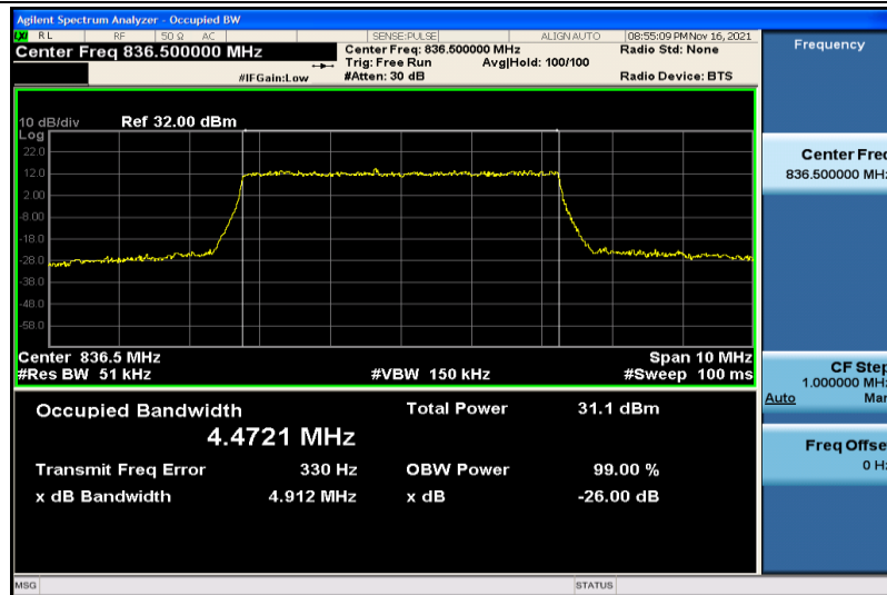
Band26-5MHz-QPSK-26915-25RB#0-4.4721
