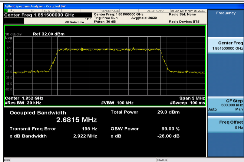
Band25-3MHz-16QAM-26055-15RB#0-2.6815
