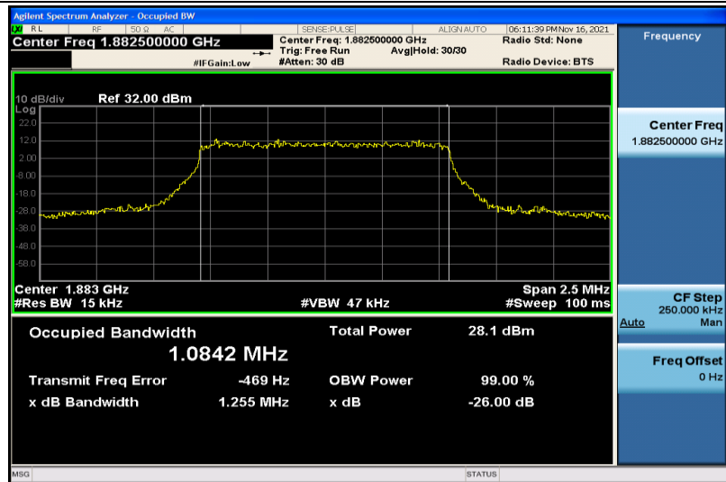
Band25-1.4MHz-16QAM-26365-6RB#0-1.0842
