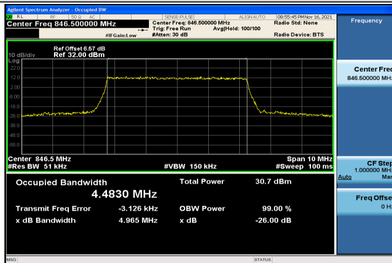
Band26-5MHz-QPSK-27015-25RB#0-4.4830
