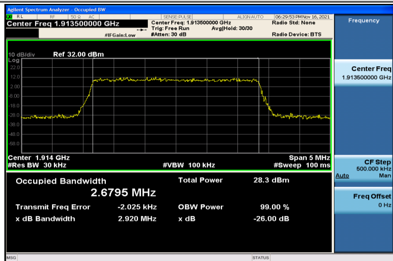
Band25-3MHz-16QAM-26675-15RB#0-2.6795
