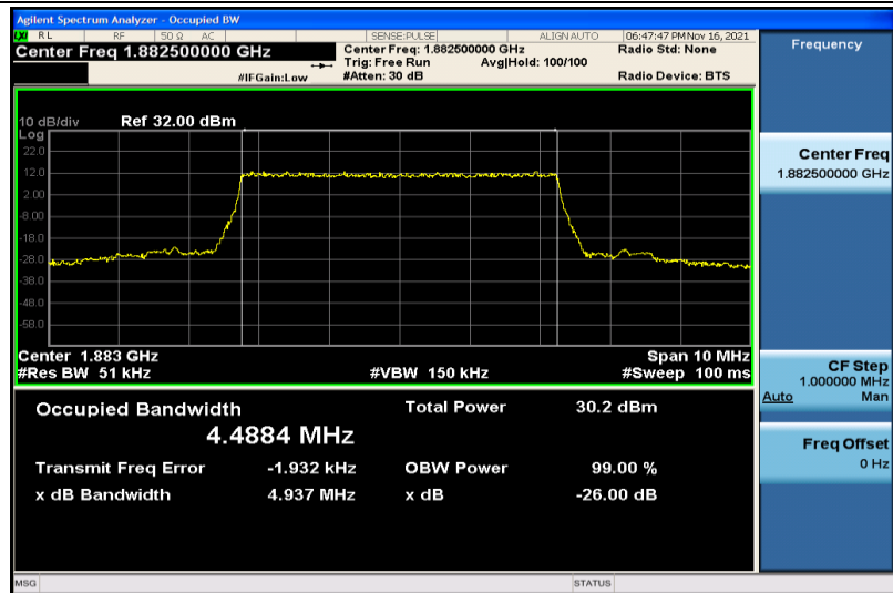
Band25-5MHz-QPSK-26365-25RB#0-4.4884
