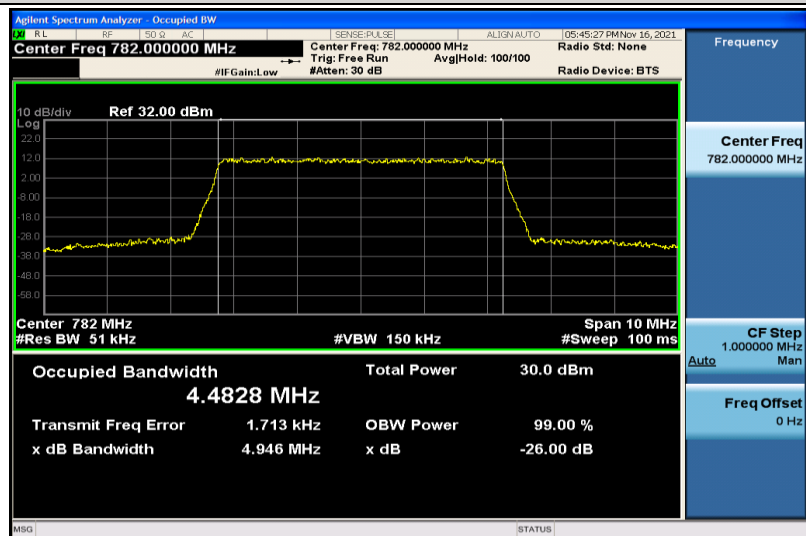
Band13-5MHz-16QAM-23230-25RB#0-4.4828
