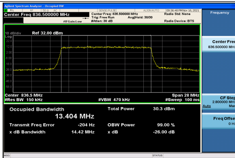
Band26-15MHz-16QAM-26915-75RB#0-13.404
