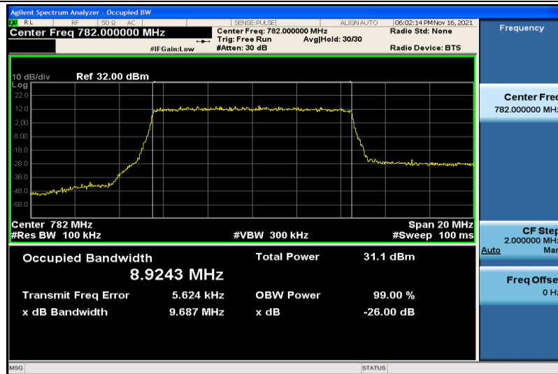
Band13-10MHz-QPSK-23230-50RB#0-8.9243
