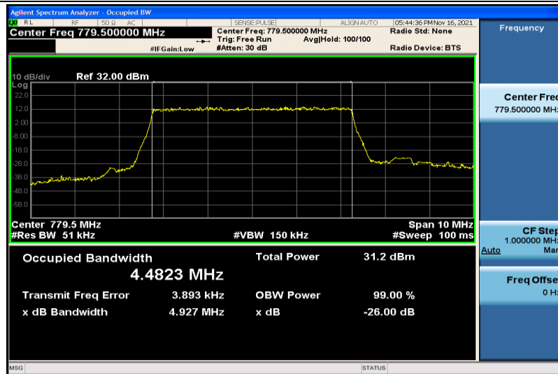
Band13-5MHz-QPSK-23205-25RB#0-4.4823
