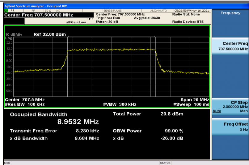
Band12-10MHz-16QAM-23095-50RB#0-8.9532
