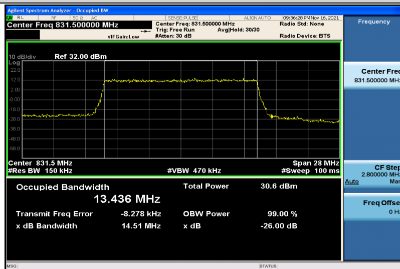
Band26-15MHz-16QAM-26865-75RB#0-13.436
