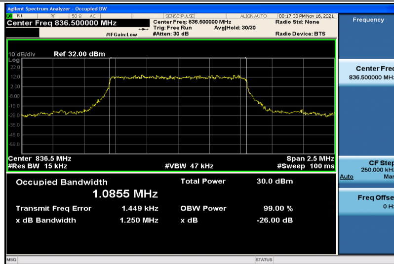
Band26-1.4MHz-QPSK-26915-6RB#0-1.0855
