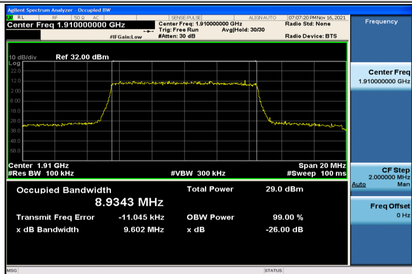
Band25-10MHz-16QAM-26640-50RB#0-8.9343
