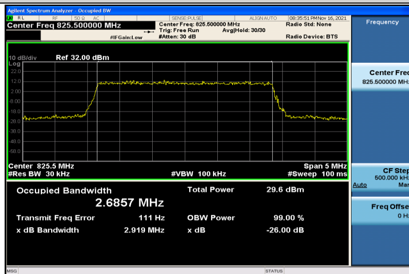
Band26-3MHz-16QAM-26805-15RB#0-2.6857
