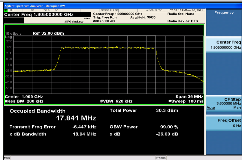
Band25-20MHz-QPSK-26590-100RB#0-17.841
