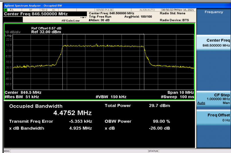
Band26-5MHz-16QAM-27015-25RB#0-4.4752
