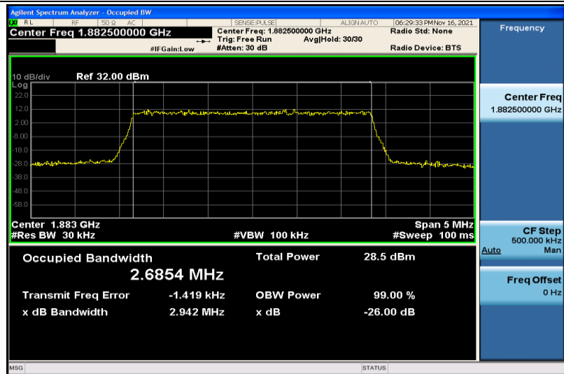
Band25-3MHz-16QAM-26365-15RB#0-2.6854
