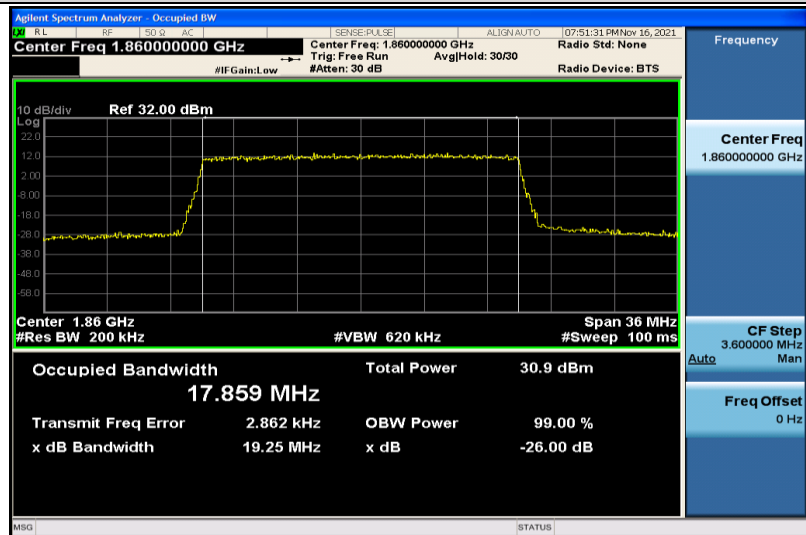
Band25-20MHz-QPSK-26140-100RB#0-17.859
