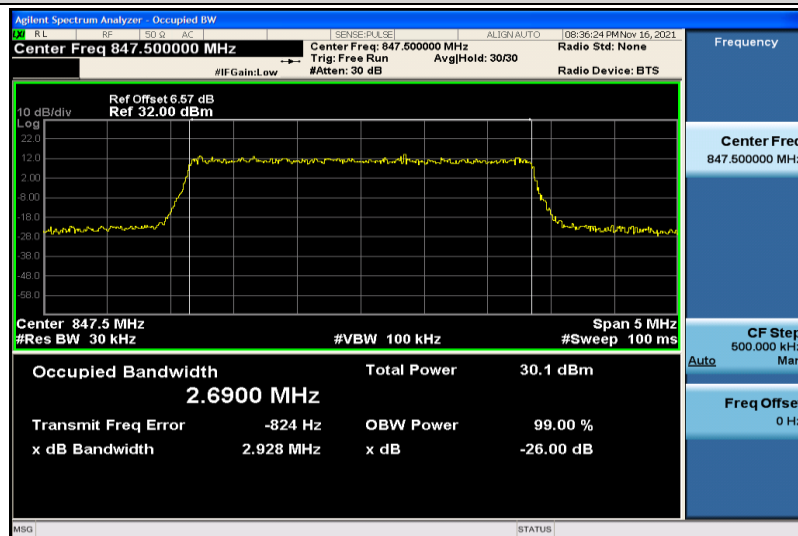
Band26-3MHz-QPSK-27025-15RB#0-2.6900
