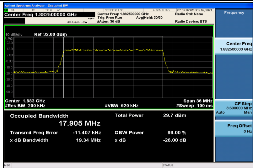
Band25-20MHz-16QAM-26365-100RB#0-17.905
