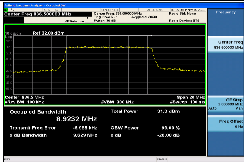
Band26-10MHz-QPSK-26915-50RB#0-8.9232
