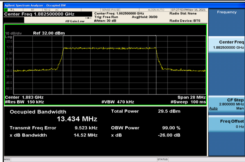
Band25-15MHz-16QAM-26365-75RB#0-13.434
