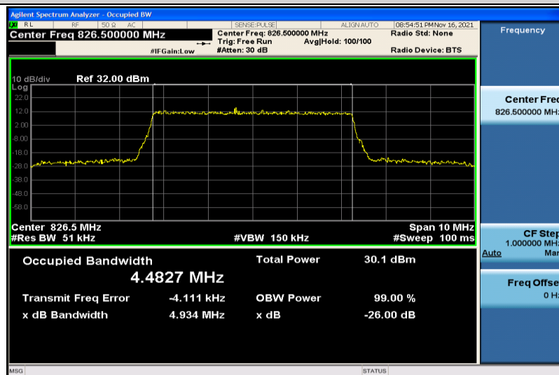
Band26-5MHz-16QAM-26815-25RB#0-4.4827
