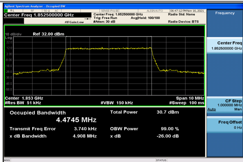
Band25-5MHz-QPSK-26065-25RB#0-4.4745
