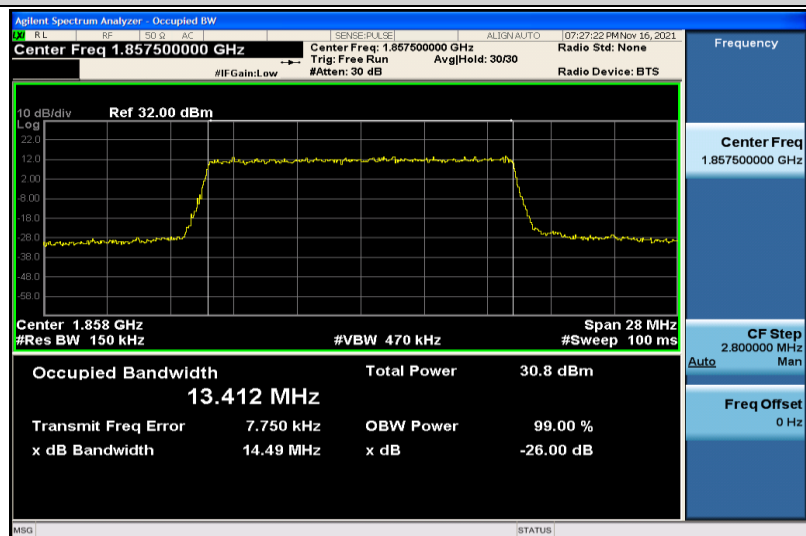
Band25-15MHz-QPSK-26115-75RB#0-13.412
