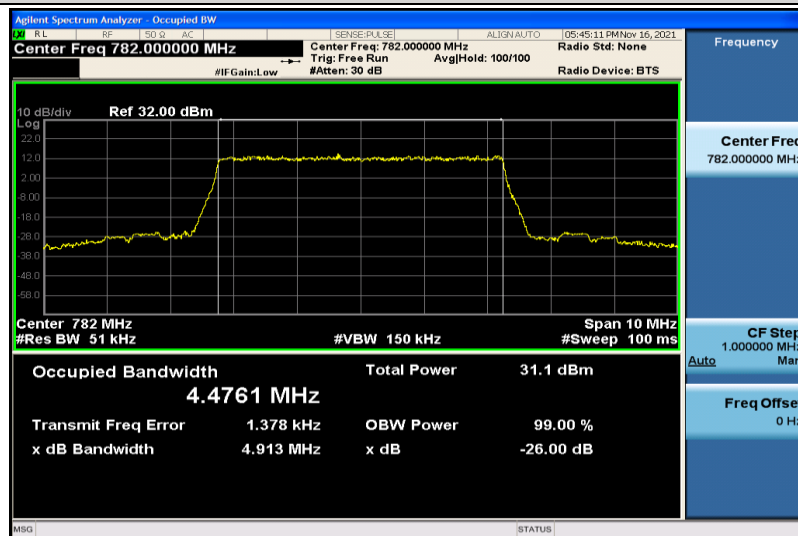
Band13-5MHz-QPSK-23230-25RB#0-4.4761
