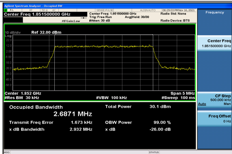
Band25-3MHz-QPSK-26055-15RB#0-2.6871
