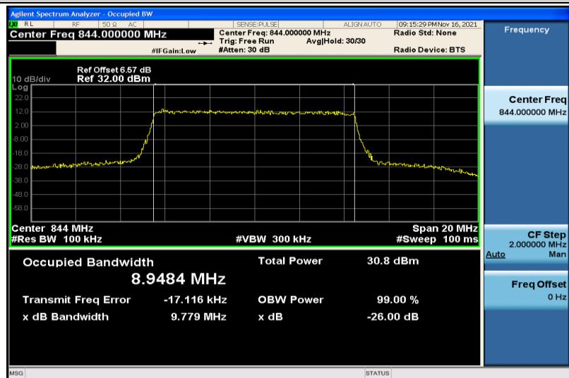
Band26-10MHz-QPSK-26990-50RB#0-8.9484
