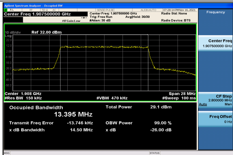
Band25-15MHz-16QAM-26615-75RB#0-13.395
