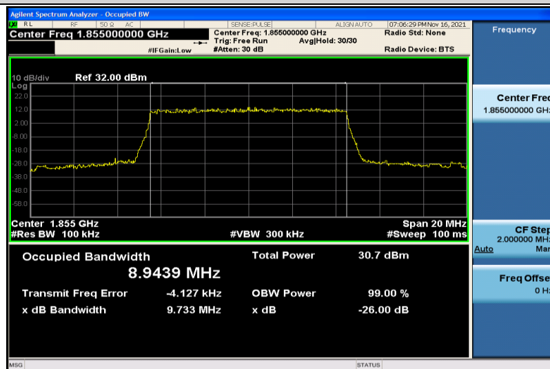
Band25-10MHz-QPSK-26090-50RB#0-8.9439
