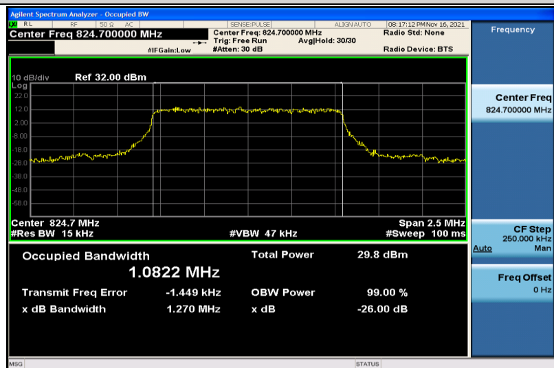
Band26-1.4MHz-QPSK-26797-6RB#0-1.0822
