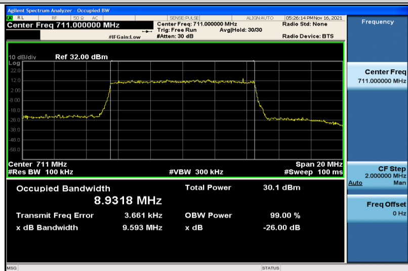
Band12-10MHz-16QAM-23130-50RB#0-8.9318
