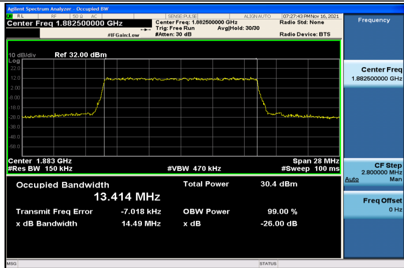
Band25-15MHz-QPSK-26365-75RB#0-13.414
