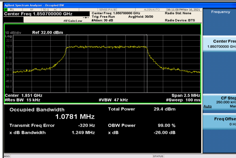
Band25-1.4MHz-QPSK-26047-6RB#0-1.0781
