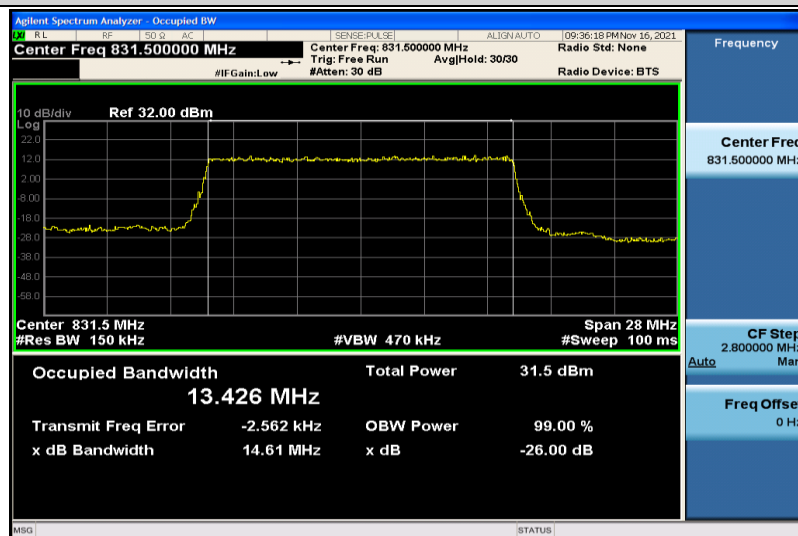
Band26-15MHz-QPSK-26865-75RB#0-13.426
