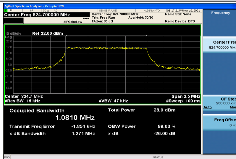
Band26-1.4MHz-16QAM-26797-6RB#0-1.0810
