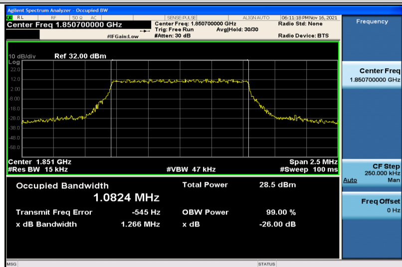
Band25-1.4MHz-16QAM-26047-6RB#0-1.0824
