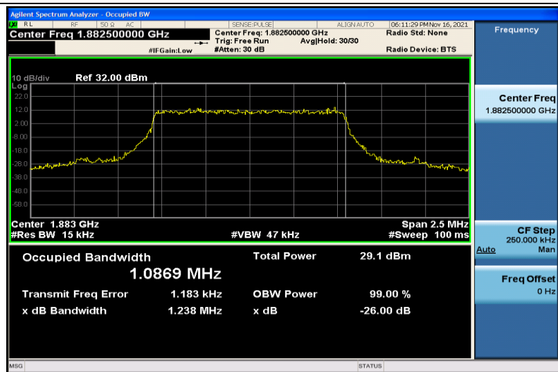
Band25-1.4MHz-QPSK-26365-6RB#0-1.0869
