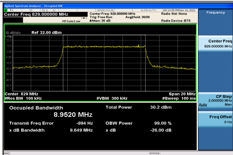
Band26-10MHz-16QAM-26840-50RB#0-8.9520
