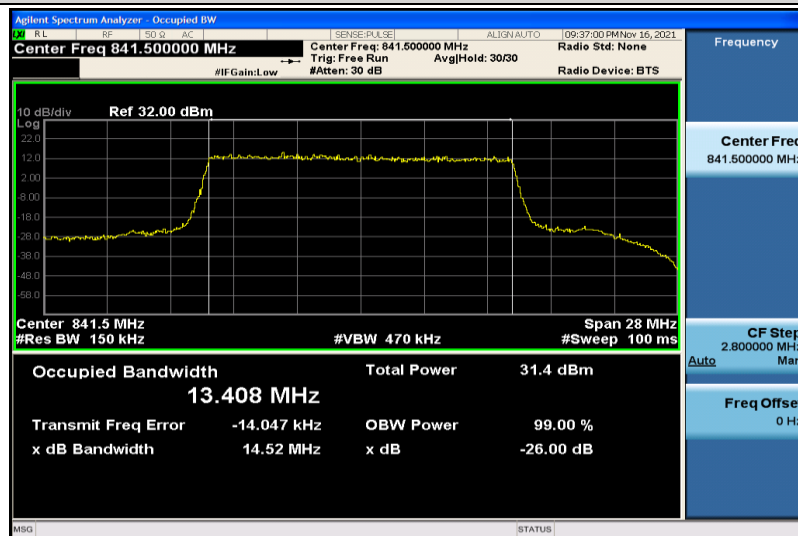
Band26-15MHz-QPSK-26965-75RB#0-13.408
