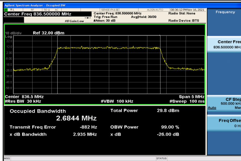
Band26-3MHz-16QAM-26915-15RB#0-2.6844
