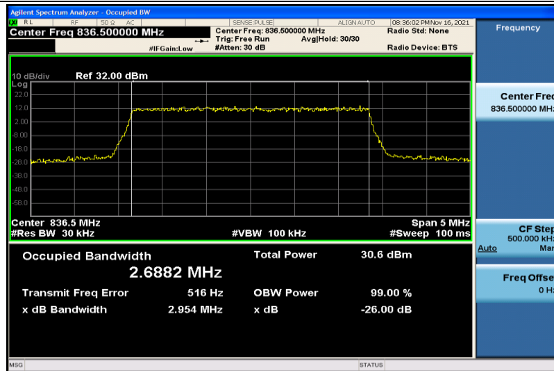
Band26-3MHz-QPSK-26915-15RB#0-2.6882
