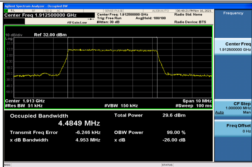
Band25-5MHz-QPSK-26665-25RB#0-4.4849
