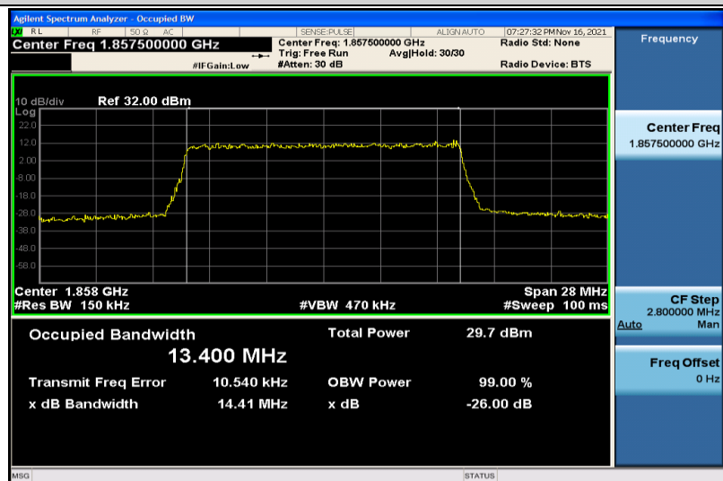
Band25-15MHz-16QAM-26115-75RB#0-13.400
