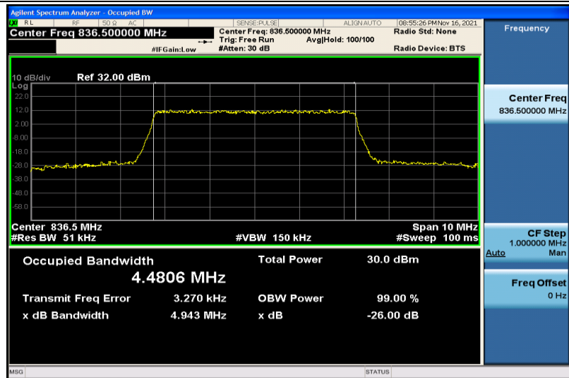
Band26-5MHz-16QAM-26915-25RB#0-4.4806
