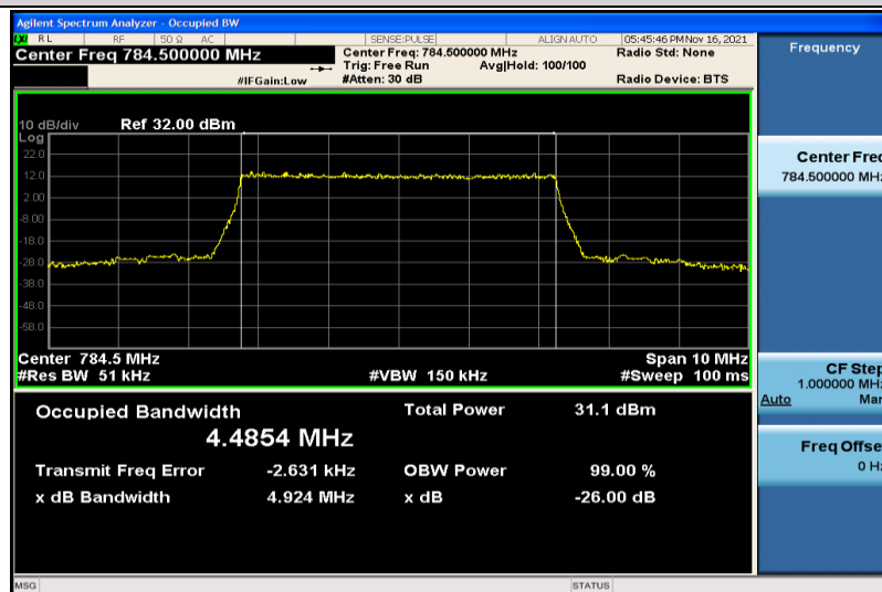
Band13-5MHz-QPSK-23255-25RB#0-4.4854
