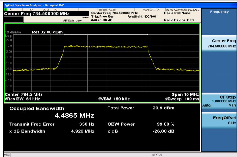
Band13-5MHz-16QAM-23255-25RB#0-4.4865
