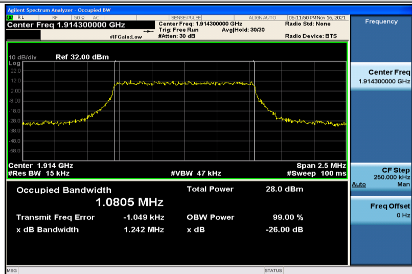
Band25-1.4MHz-QPSK-26683-6RB#0-1.0805
