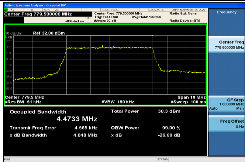
Band13-5MHz-16QAM-23205-25RB#0-4.4733
