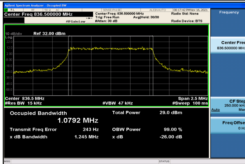
Band26-1.4MHz-16QAM-26915-6RB#0-1.0792
