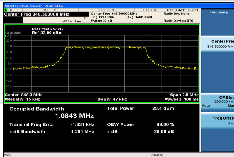
Band26-1.4MHz-16QAM-27033-6RB#0-1.0843
