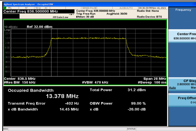
Band26-15MHz-QPSK-26915-75RB#0-13.378
