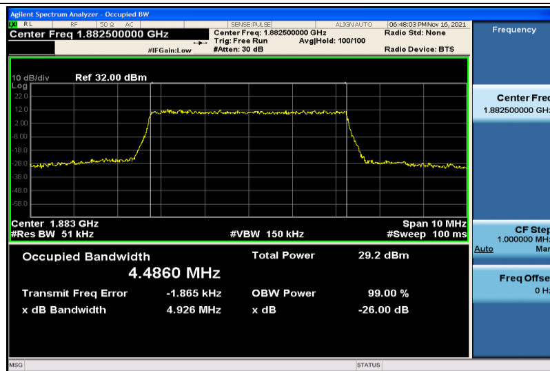
Band25-5MHz-16QAM-26365-25RB#0-4.4860
