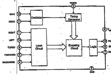
TRANSMITTER Tx2 Block Diagram
