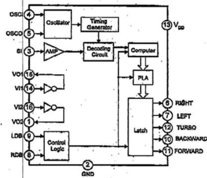
RECEIVER Rx2 Block Diagram
