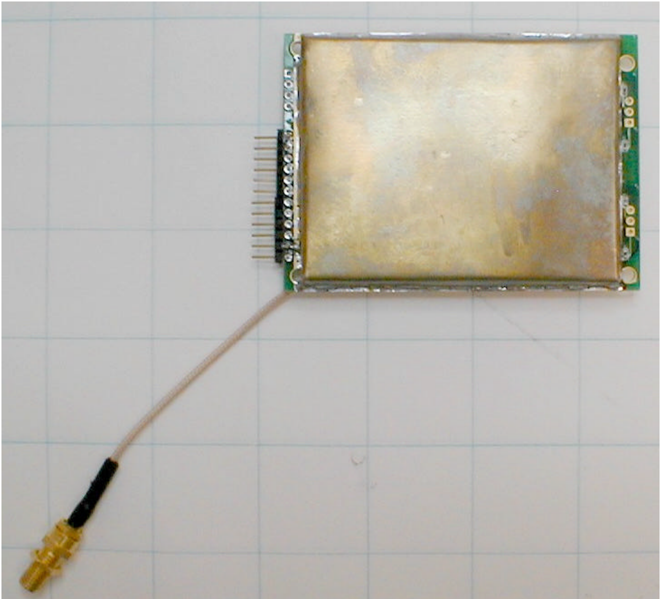
Top View
