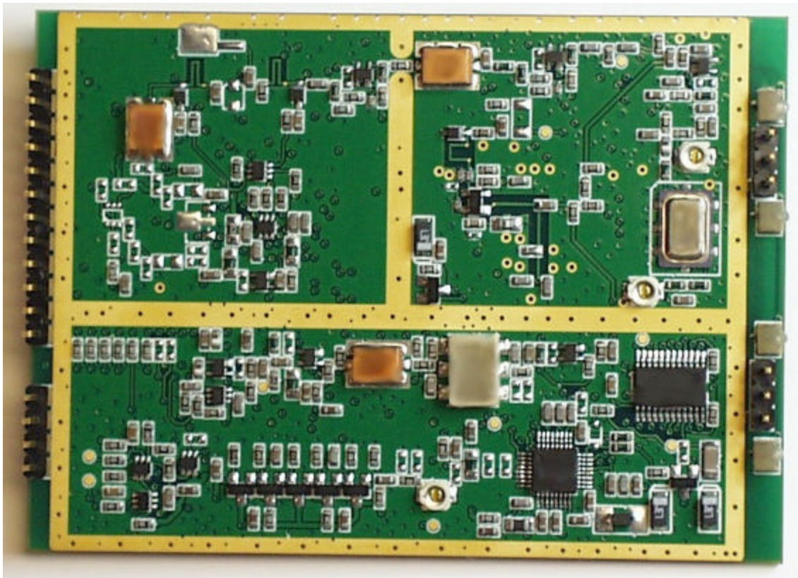
Top View (Shields Removed)
