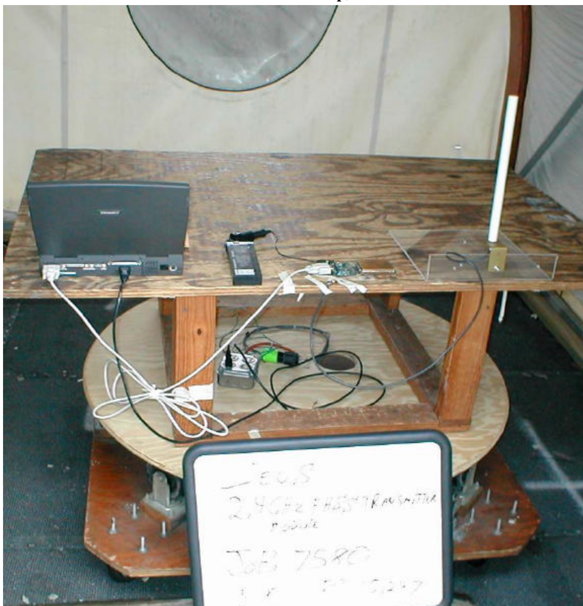
Emissions Test Setup, Back
