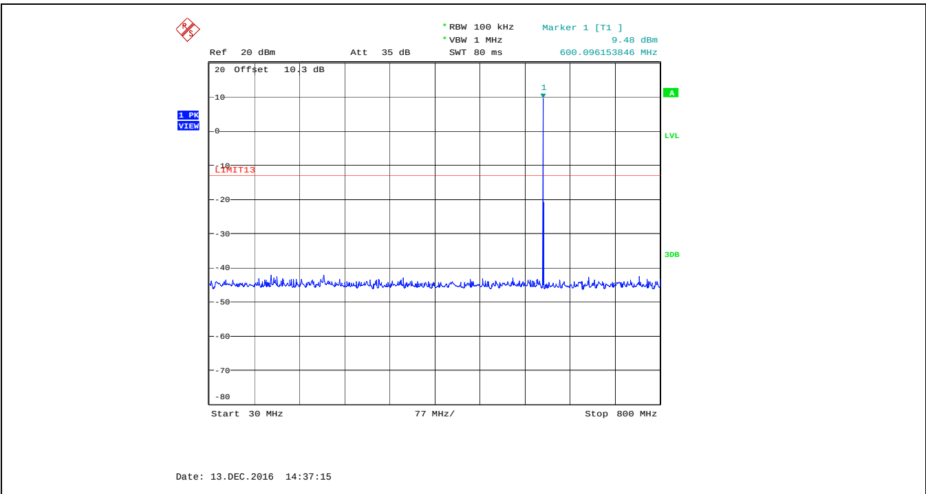
Plot 5.5.4.16. Spurious Emissions at Antenna Terminal, 600.0 MHz, Low Power, Audio Input 15 kHz 1 Vrms 30 MHz - 800 MHz
