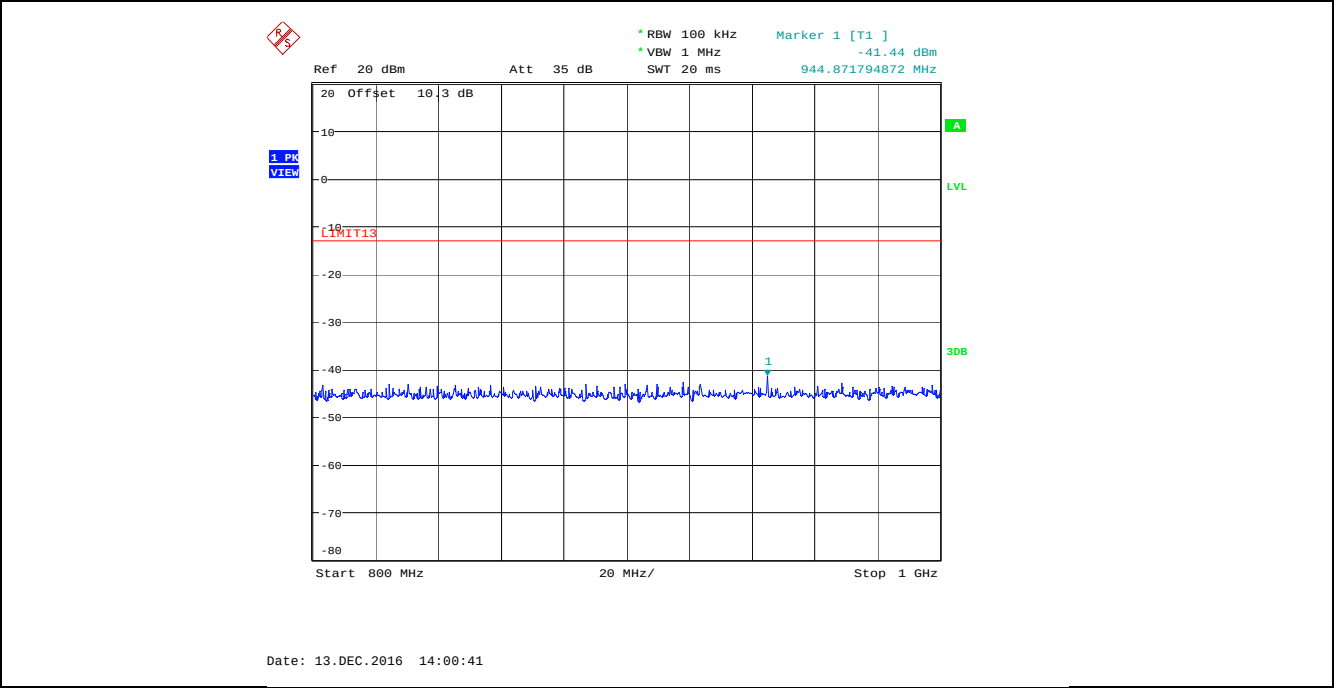
Plot 5.5.4.2. Spurious Emissions at Antenna Terminal, 525.0 MHz, High Power, Audio Input 15 kHz 1 Vrms 800 MHz - 1 GHz
