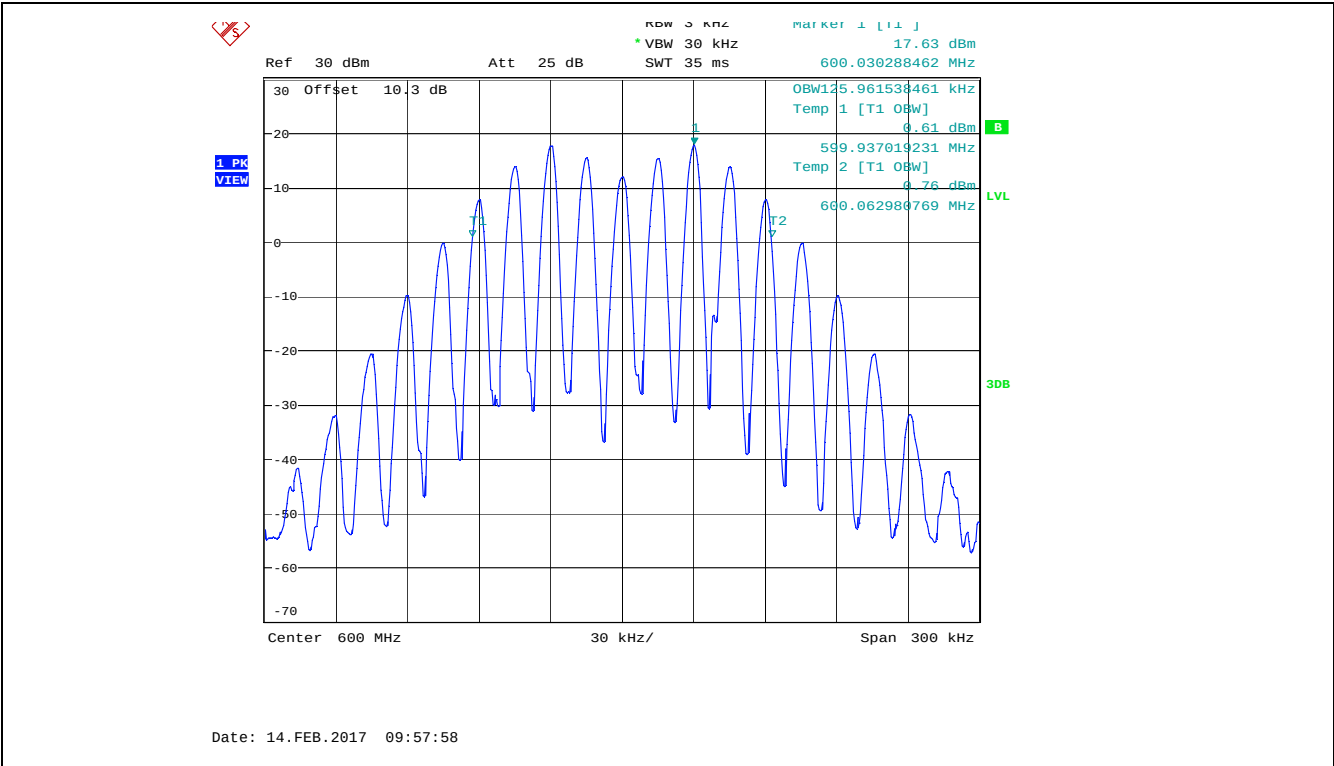
Plot 5.4.4.1.3. Occupied Bandwidth 99%, 600.0 MHz, Audio input 15 kHz 1 Vrms, High Power
