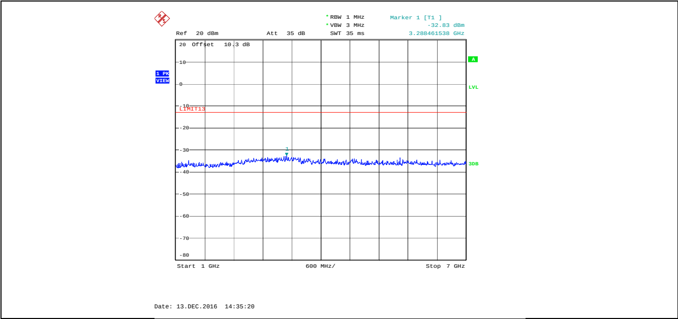
Plot 5.5.4.18. Spurious Emissions at Antenna Terminal, 600.0 MHz, Low Power, Audio Input 15 kHz 1 Vrms 1 GHz - 7 GHz
