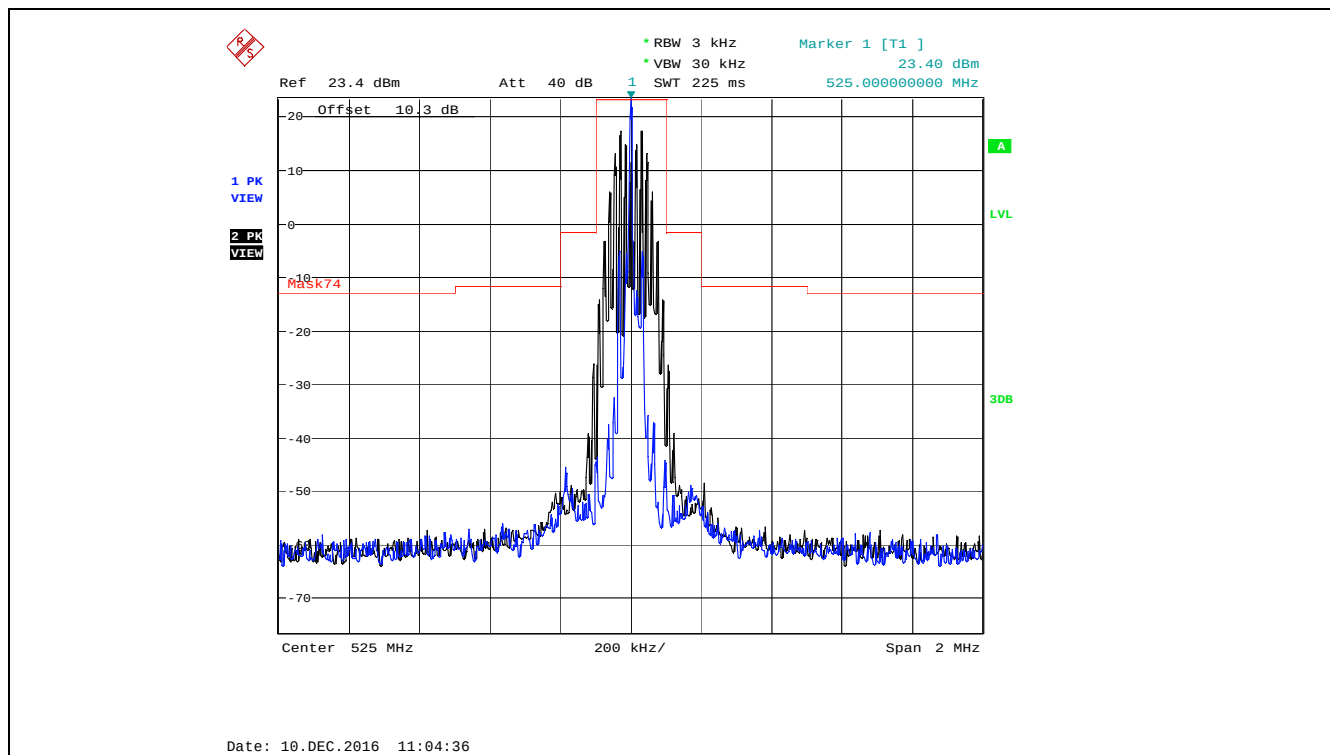
Plot 5.4.4.2.1. Emission Mask of §74.861(e)(6), 525.0 MHz, High Power, Audio input 15 kHz 1 Vrms
