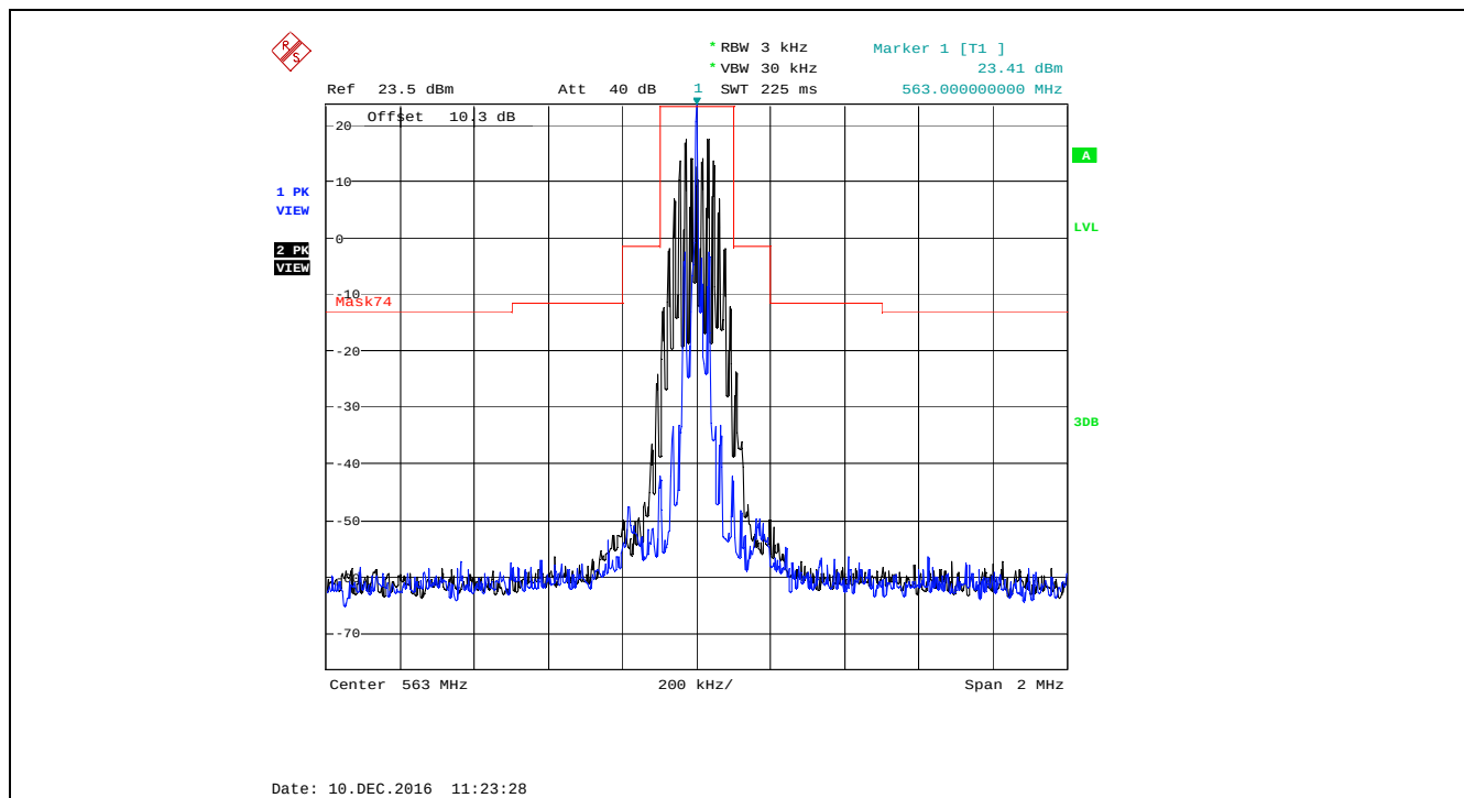
Plot 5.4.4.2.3. Emission Mask of §74.861(e)(6), 563.0 MHz, High Power, Audio input 15 kHz 1 Vrms
