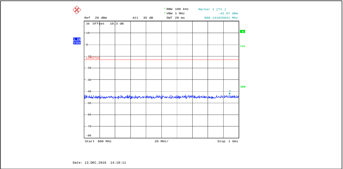
Plot 5.5.4.8. Spurious Emissions at Antenna Terminal, 563.0 MHz, High Power, Audio Input 15 kHz 1 Vrms 800 MHz - 1 GHz
