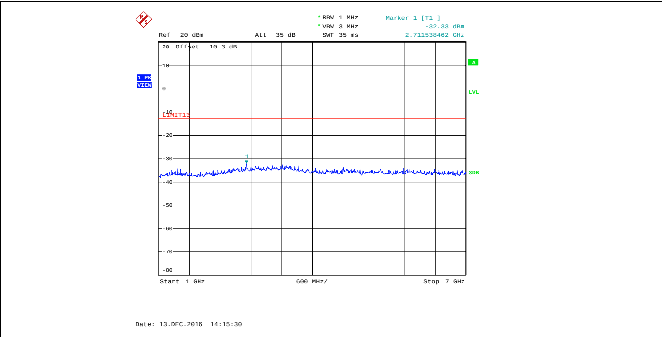
Plot 5.5.4.12. Spurious Emissions at Antenna Terminal, 563.0 MHz, Low Power, Audio Input 15 kHz 1 Vrms 1 GHz - 7 GHz
