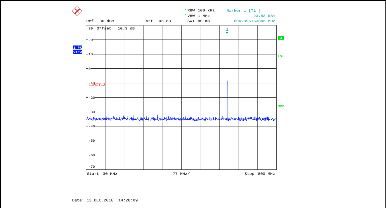
Plot 5.5.4.13. Spurious Emissions at Antenna Terminal, 600.0 MHz, High Power, Audio Input 15 kHz 1 Vrms 30 MHz - 800 MHz
