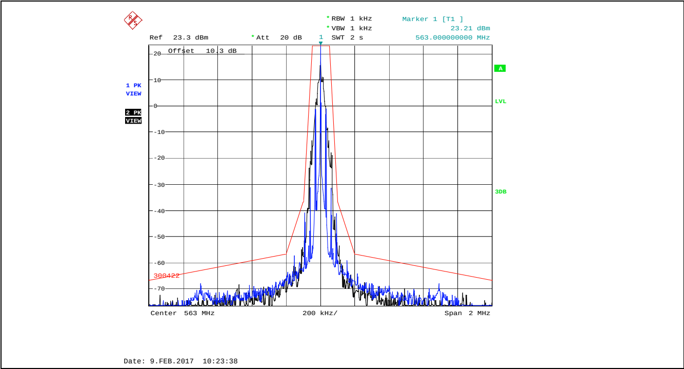
Plot 5.4.4.3.4. Emission Mask of §74.861(e)(7), 563.0 MHz, Low Power Audio input maximum 1 Vrms, Noise source input level 1V band limit to 15 kHz
