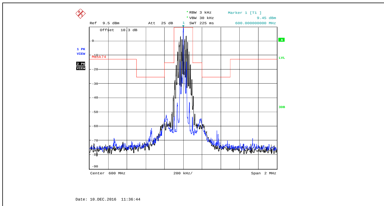
Plot 5.4.4.2.6. Emission Mask of §74.861(e)(6), 600.0 MHz, Low Power, Audio input 15 kHz 1 Vrms
