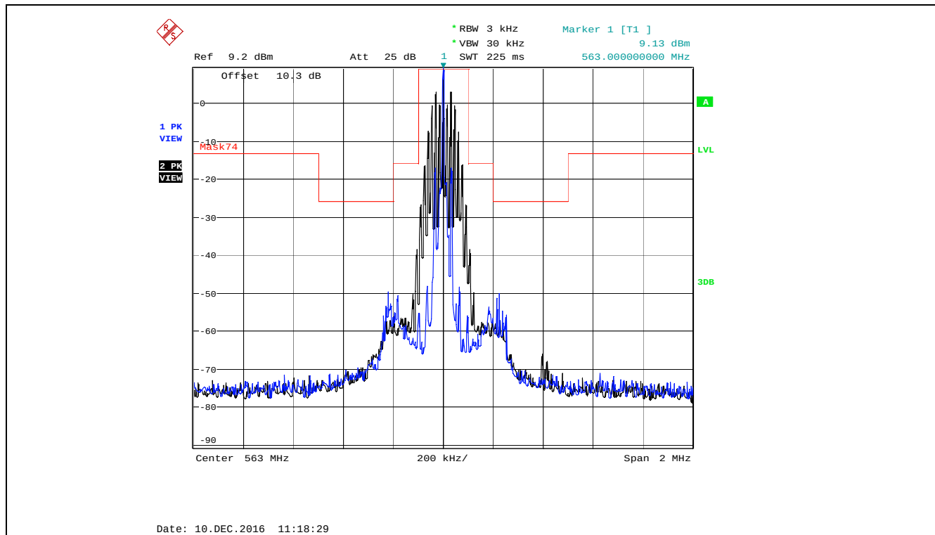
Plot 5.4.4.2.4. Emission Mask of §74.861(e)(6), 563.0 MHz, Low Power, Audio input 15 kHz 1 Vrms
