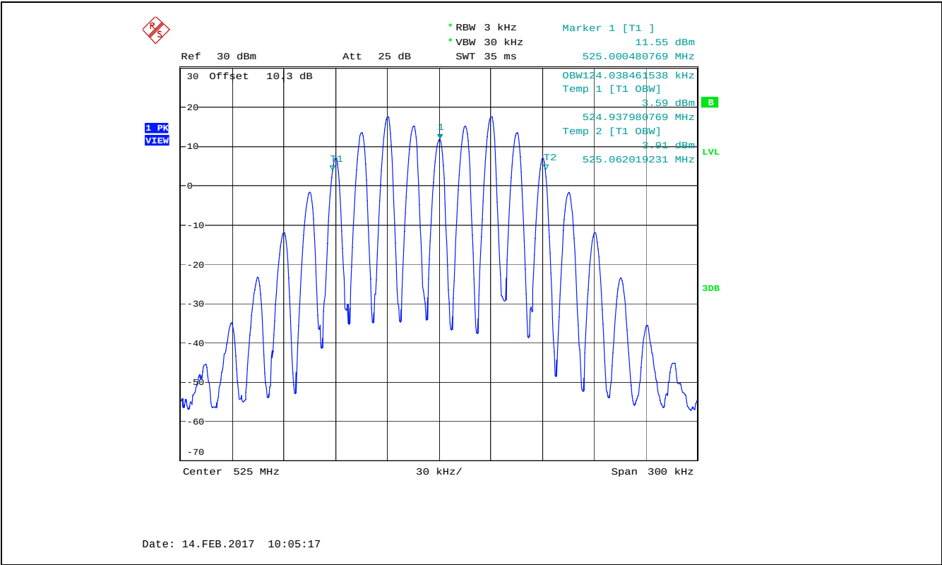
Plot 5.4.4.1.1. Occupied Bandwidth 99%, 525.0 MHz, Audio input 15 kHz 1 Vrms, High Power
