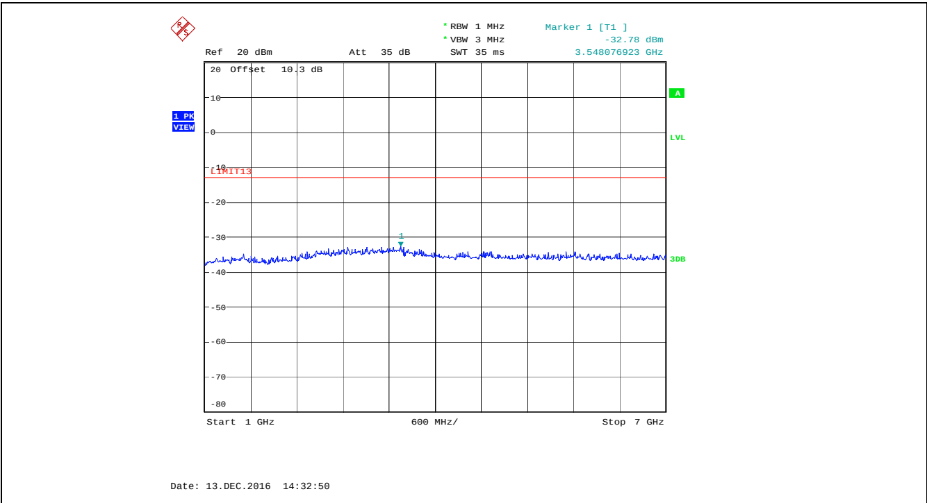
Plot 5.5.4.15. Spurious Emissions at Antenna Terminal, 600.0 MHz, High Power, Audio Input 15 kHz 1 Vrms 1 GHz - 7 GHz
