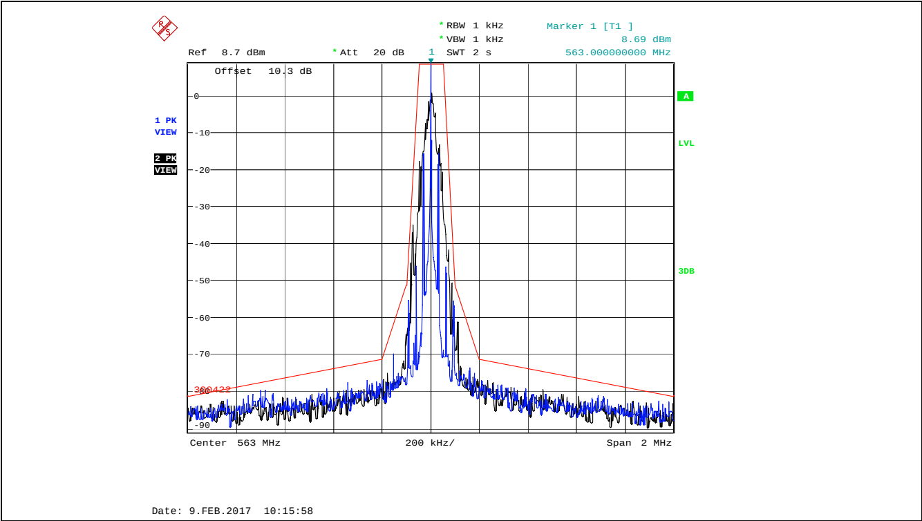
Plot 5.4.4.3.4. Emission Mask of §74.861(e)(7), 563.0 MHz, Low Power Audio input maximum 1 Vrms, Noise source input level 1V band limit to 15 kHz
