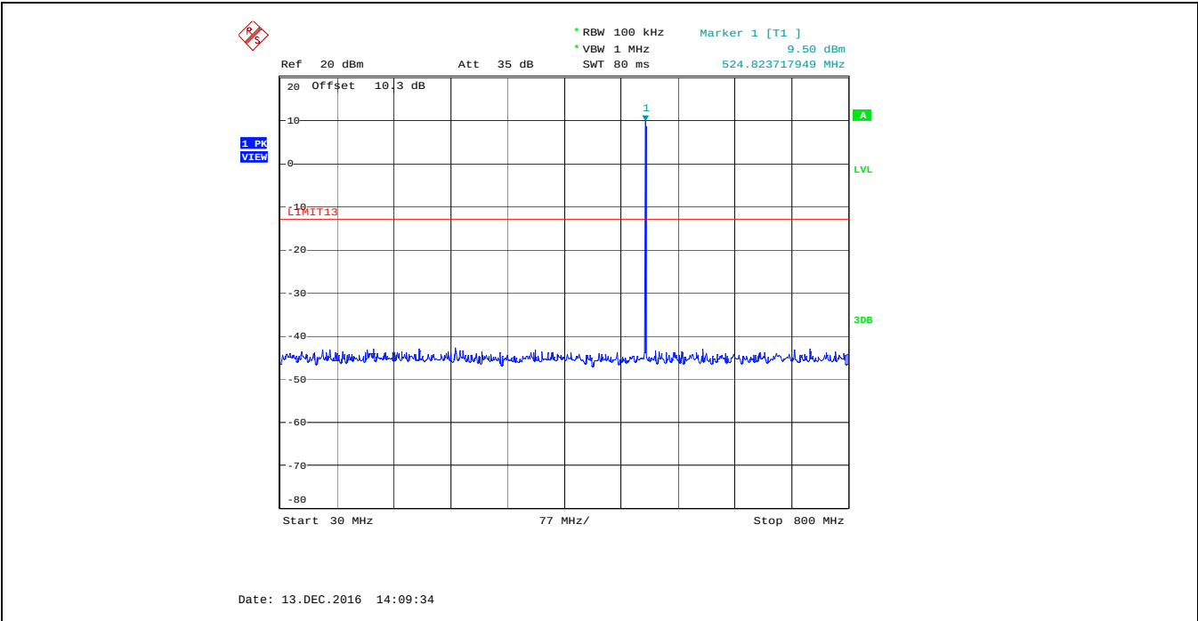
Plot 5.5.4.4. Spurious Emissions at Antenna Terminal, 525.0 MHz, Low Power, Audio Input 15 kHz 1 Vrms 30 MHz - 800 MHz
