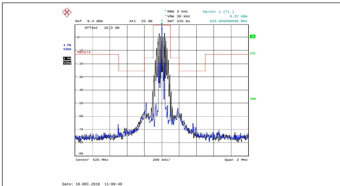
Plot 5.4.4.2.2. Emission Mask of §74.861(e)(6), 525.0 MHz, Low Power, Audio input 15 kHz 1 Vrms
