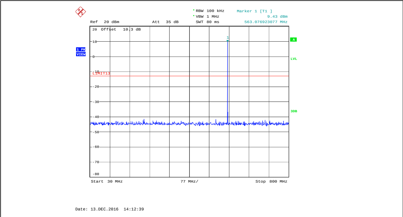
Plot 5.5.4.10. Spurious Emissions at Antenna Terminal, 563.0 MHz, Low Power, Audio Input 15 kHz 1 Vrms 30 MHz - 800 MHz
