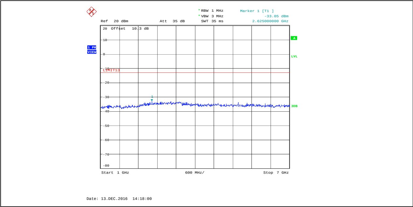
Plot 5.5.4.9. Spurious Emissions at Antenna Terminal, 563.0 MHz, High Power, Audio Input 15 kHz 1 Vrms 1 GHz - 7 GHz
