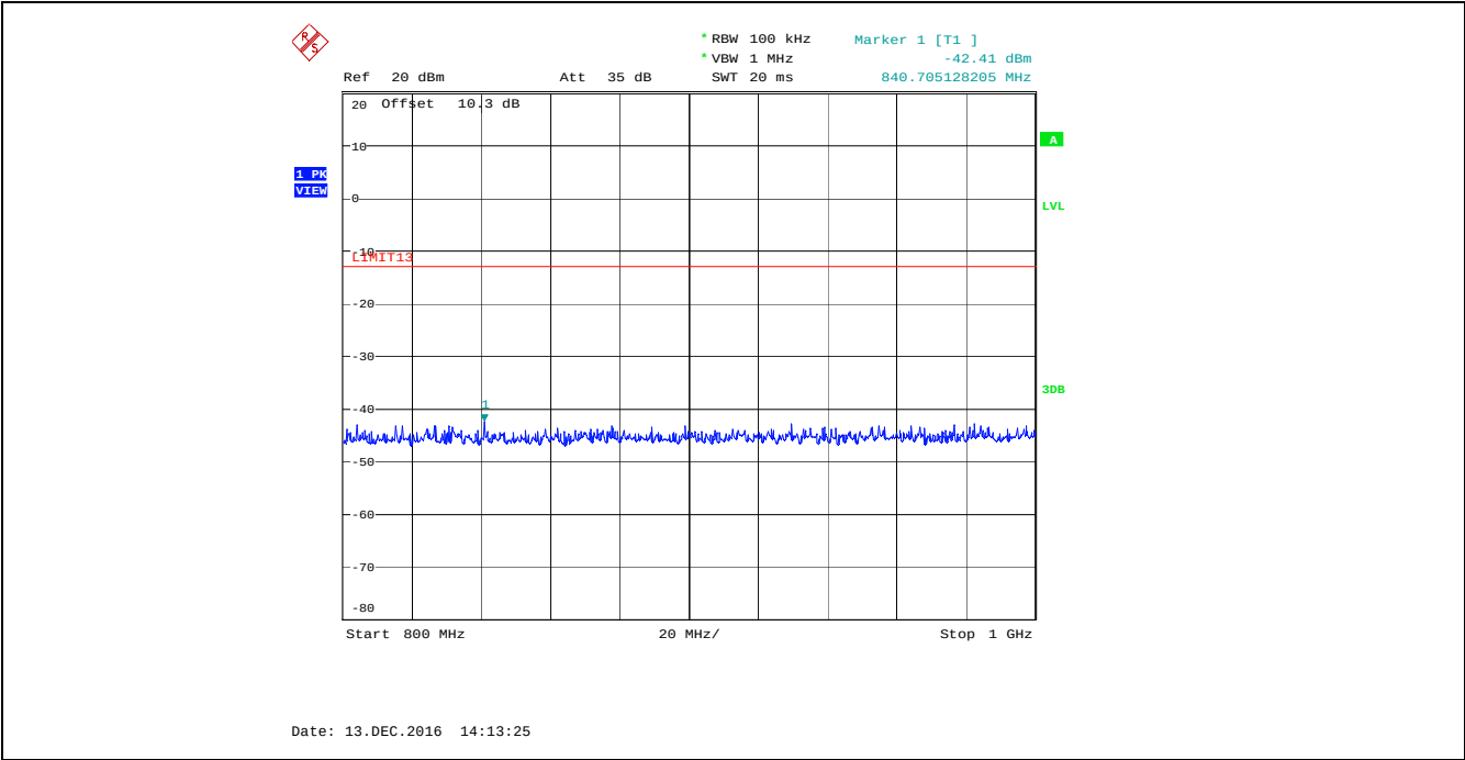
Plot 5.5.4.11. Spurious Emissions at Antenna Terminal, 563.0 MHz, Low Power, Audio Input 15 kHz 1 Vrms 800 MHz - 1 GHz
