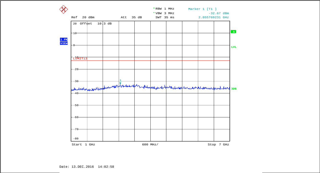
Plot 5.5.4.3. Spurious Emissions at Antenna Terminal, 525.0 MHz, High Power, Audio Input 15 kHz 1 Vrms 1 GHz - 7 GHz
