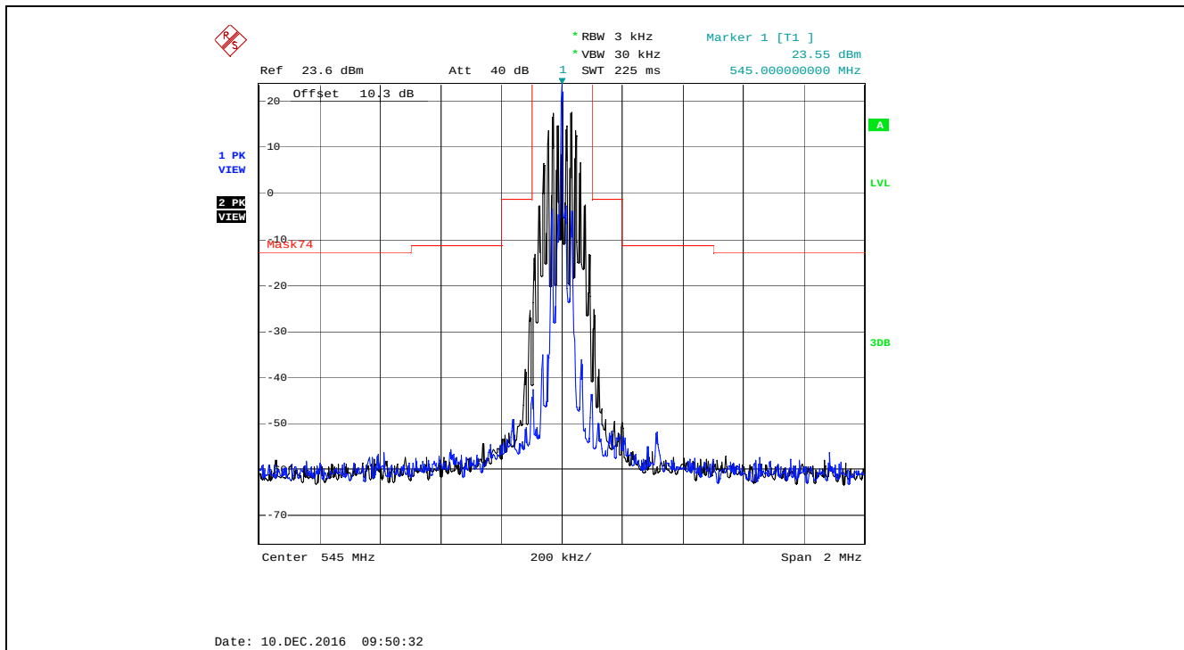
Plot 5.4.4.2.6. Emission Mask of §74.861(e)(6), 545.000 MHz, Low Power, Audio input 15 kHz 1 Vrms
