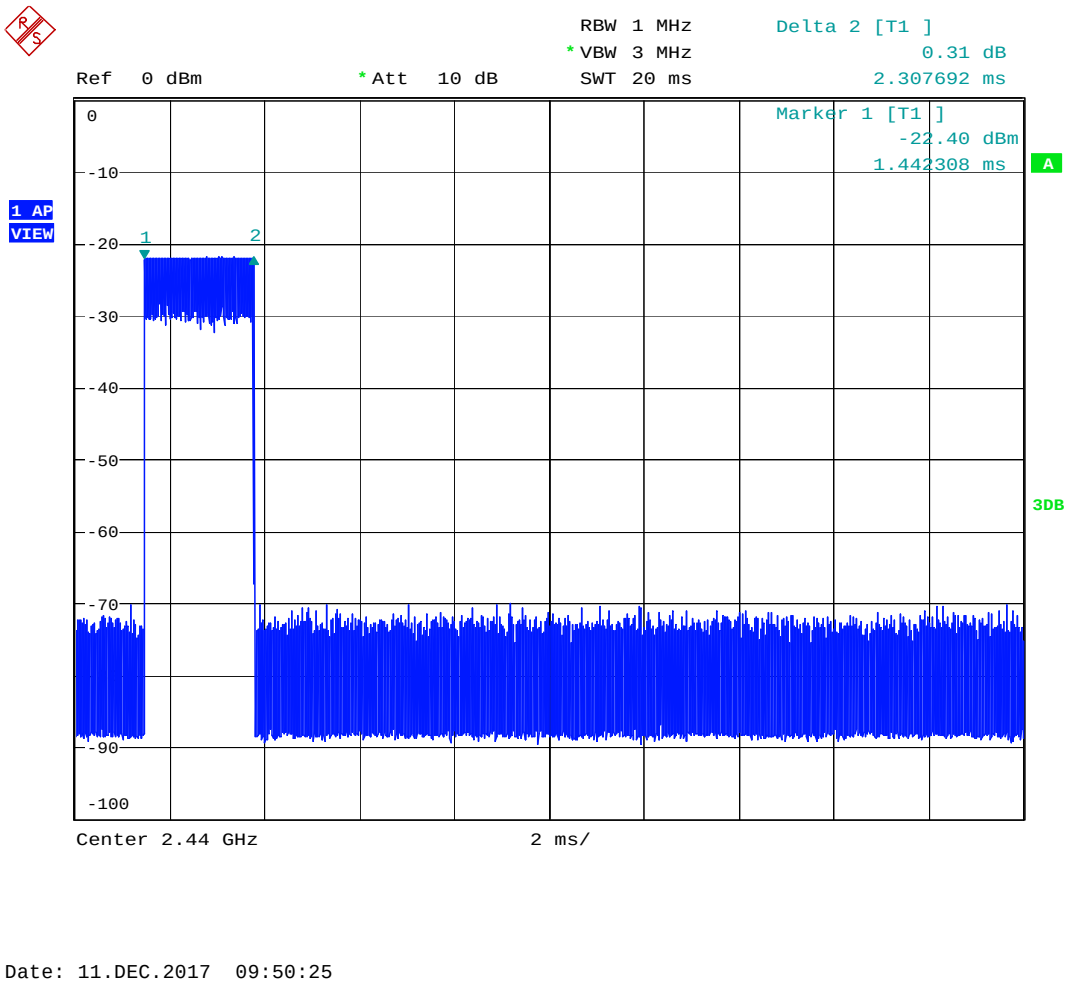
Plot 3 Duty Cycle, Pulse
