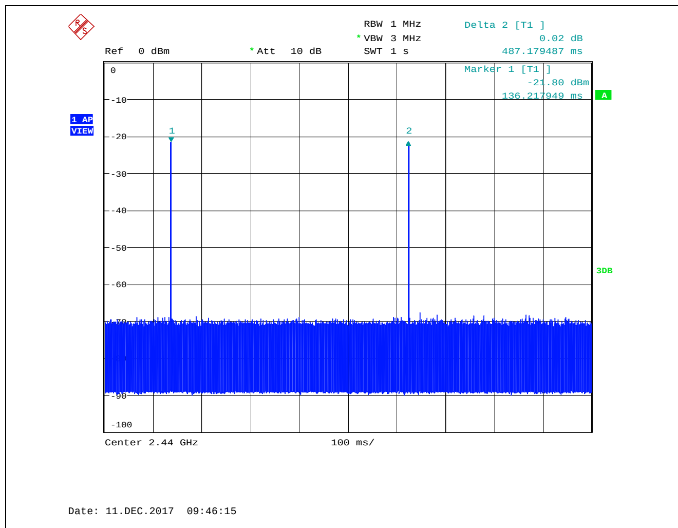
Plot 1 Duty Cycle, Pulse Train
