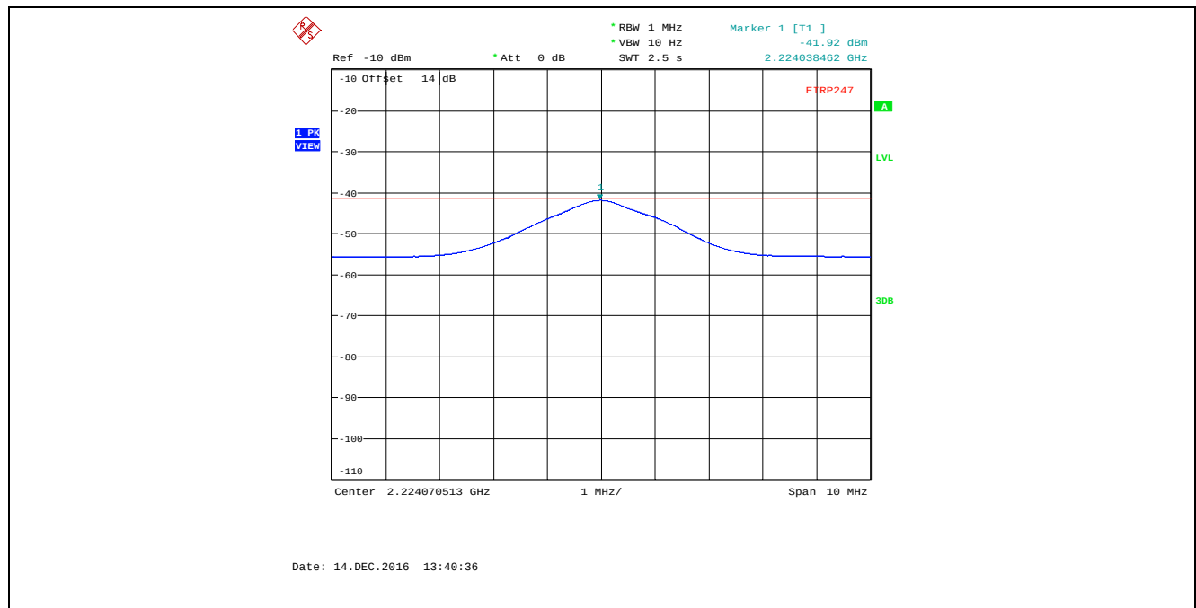
Plot 5.4.4.3.21. Conducted Spurious Emissions in Restricted Frequency Bands Channel 16, 2480 MHz, MSK Modulation, Power Setting 12, 2.2191 - 2.2291 GHz, Average Detector
