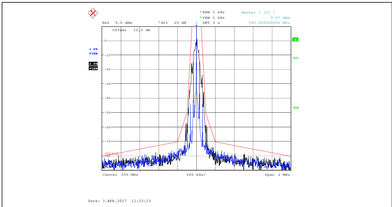
Plot 5.4.4.3.6. Emission Mask of §74.861(e)(7), 550.000 MHz, Low Power Audio input maximum 1 Vrms, Noise source input level 1V band limit to 15 kHz
