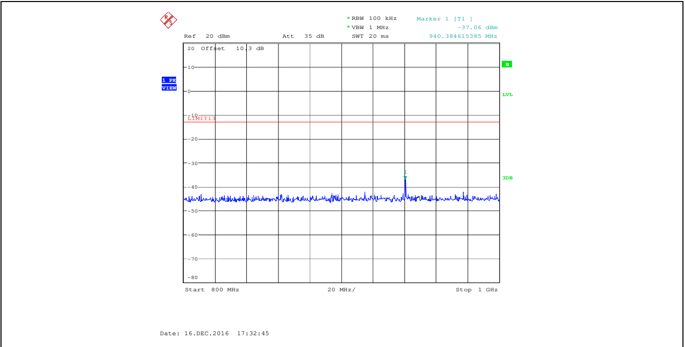
Plot 5.5.4.2. Spurious Emissions at Antenna Terminal, 470.250 MHz, High Power, Audio Input 15 kHz 1 Vrms 800 MHz - 1 GHz
