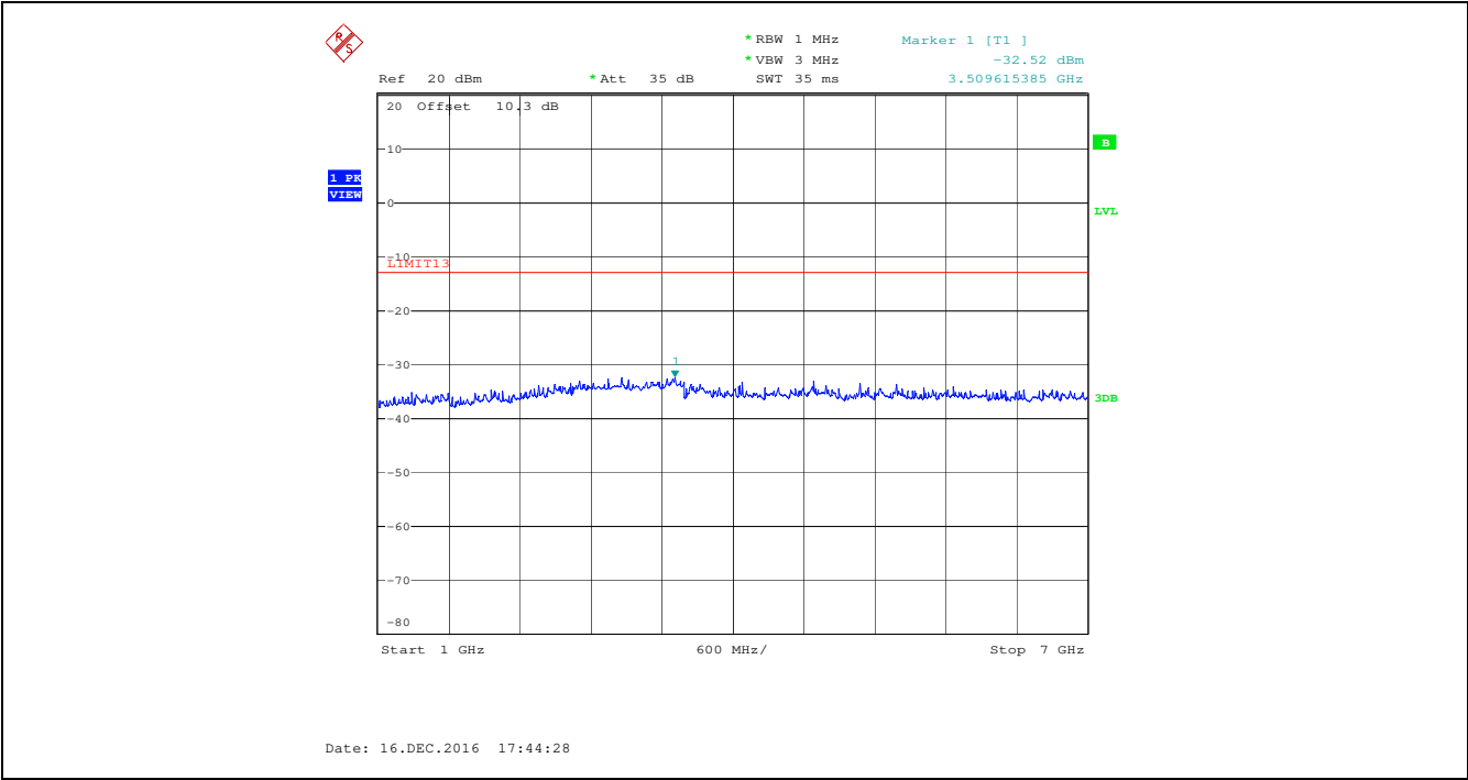
Plot 5.5.4.15. Spurious Emissions at Antenna Terminal, 550.000 MHz, High Power, Audio Input 15 kHz 1 Vrms 1 GHz - 7 GHz
