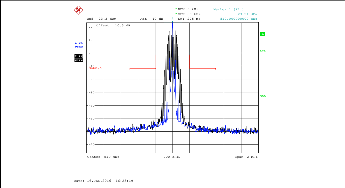
Plot 5.4.4.2.3. Emission Mask of §74.861(e)(6), 510.000 MHz, High Power, Audio input 15 kHz 1 Vrms
