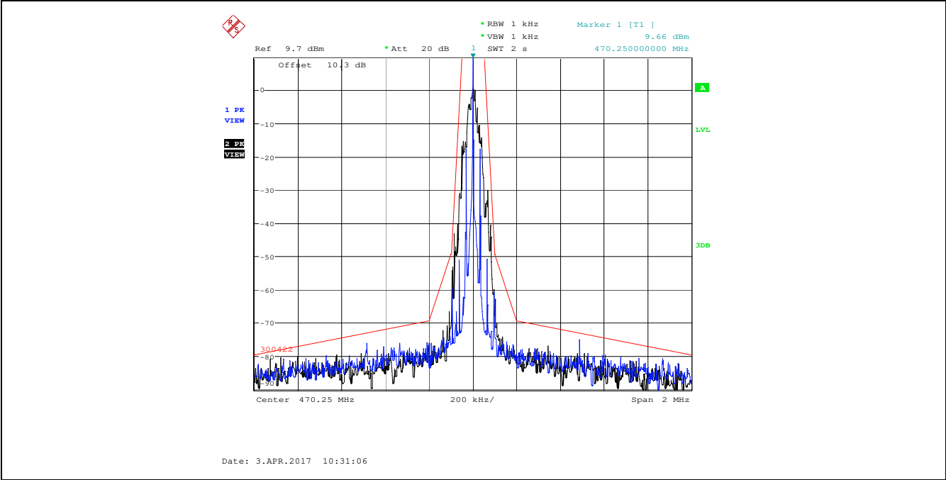
Plot 5.4.4.3.2. Emission Mask of §74.861(e)(7), 470.250 MHz, Low Power Audio input maximum 1 Vrms, Noise source input level 1V band limit to 15 kHz
