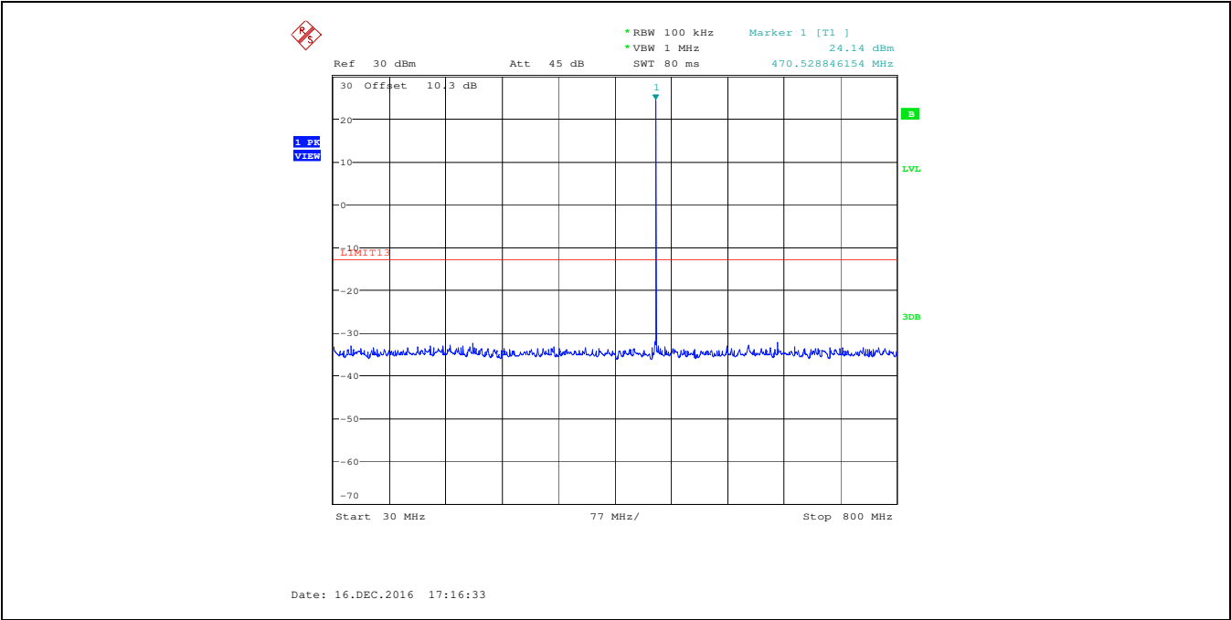
Plot 5.5.4.1. Spurious Emissions at Antenna Terminal, 470.250 MHz, High Power, Audio Input 15 kHz 1 Vrms 30 MHz - 800 MHz
