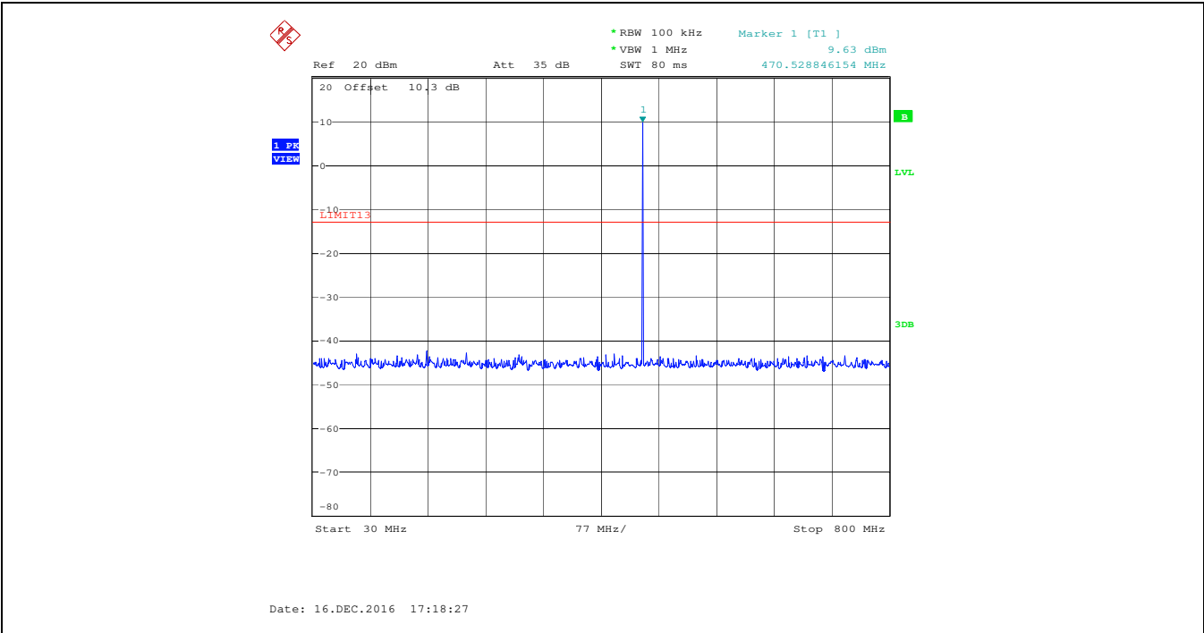
Plot 5.5.4.4. Spurious Emissions at Antenna Terminal, 470.250 MHz, Low Power, Audio Input 15 kHz 1 Vrms 30 MHz - 800 MHz
