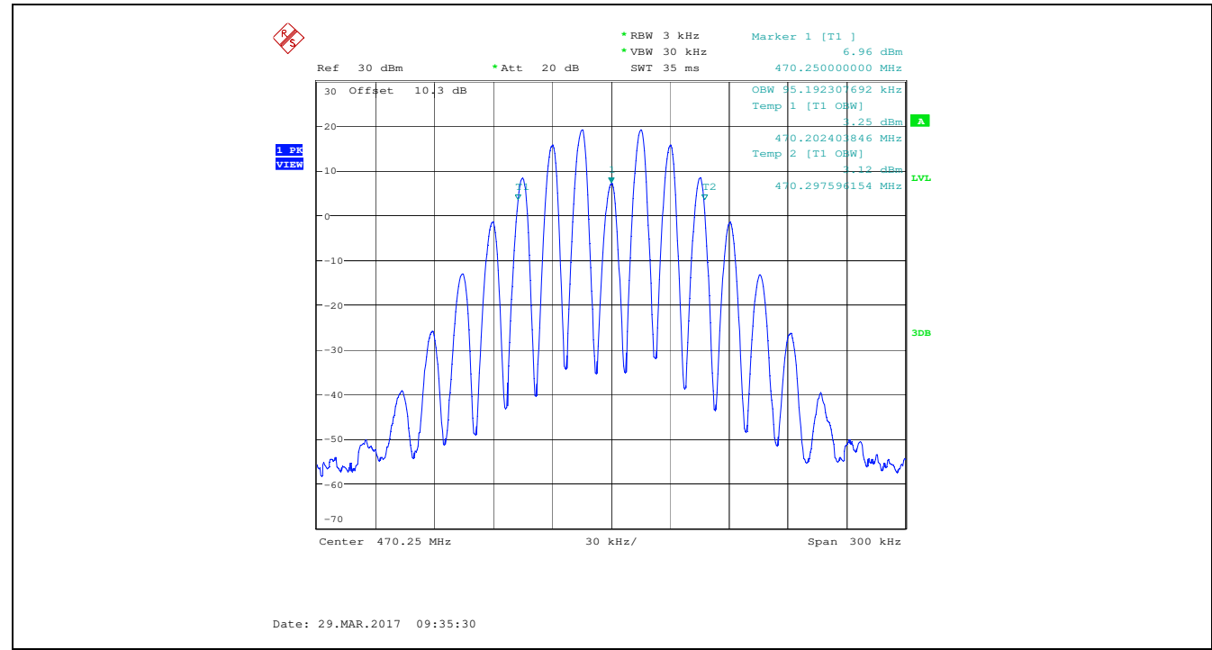
Plot 5.4.4.1.1. Occupied Bandwidth, 470.250 MHz, Audio input 15 kHz 1 Vrms, High Power
