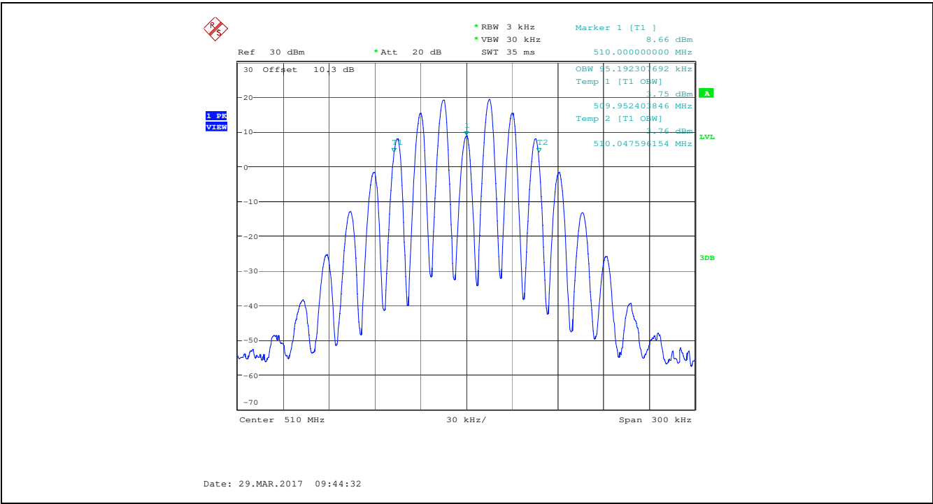
Plot 5.4.4.1.2. Occupied Bandwidth, 510.000 MHz, Audio input 15 kHz 1 Vrms, High Power
