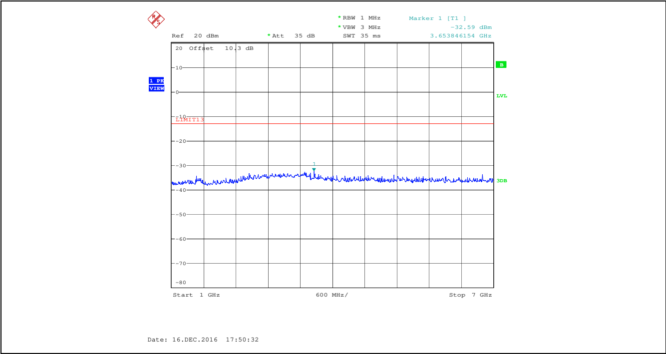
Plot 5.5.4.3. Spurious Emissions at Antenna Terminal, 470.250 MHz, High Power, Audio Input 15 kHz 1 Vrms 1 GHz - 7 GHz
