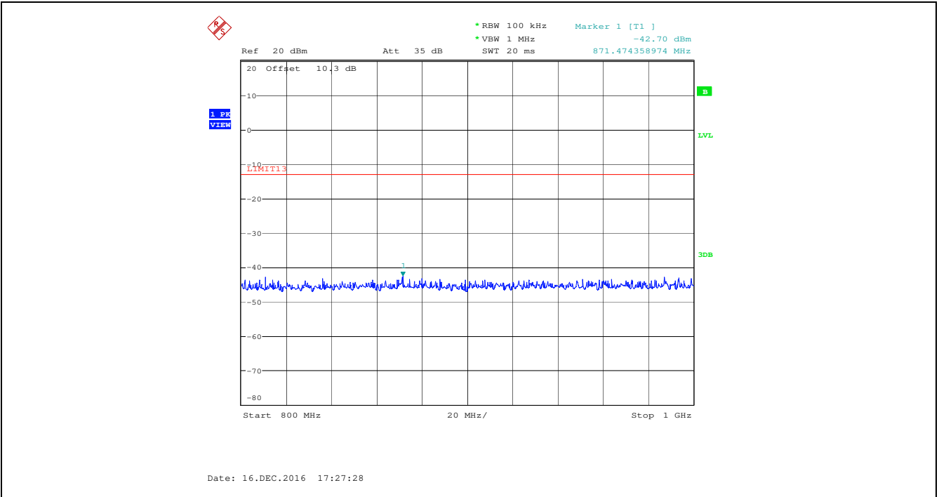
Plot 5.5.4.8. Spurious Emissions at Antenna Terminal, 510.000 MHz, High Power, Audio Input 15 kHz 1 Vrms 800 MHz - 1 GHz
