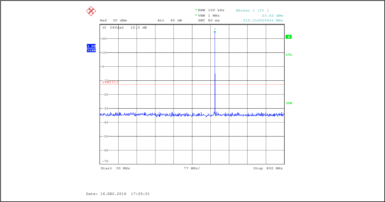
Plot 5.5.4.7. Spurious Emissions at Antenna Terminal, 510.000 MHz, High Power, Audio Input 15 kHz 1 Vrms 30 MHz - 800 MHz
