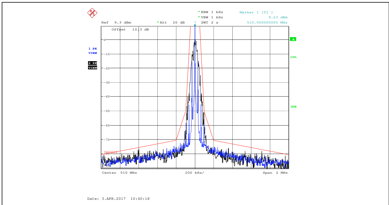
Plot 5.4.4.3.4. Emission Mask of §74.861(e)(7), 510.000 MHz, Low Power Audio input maximum 1 Vrms, Noise source input level 1V band limit to 15 kHz
