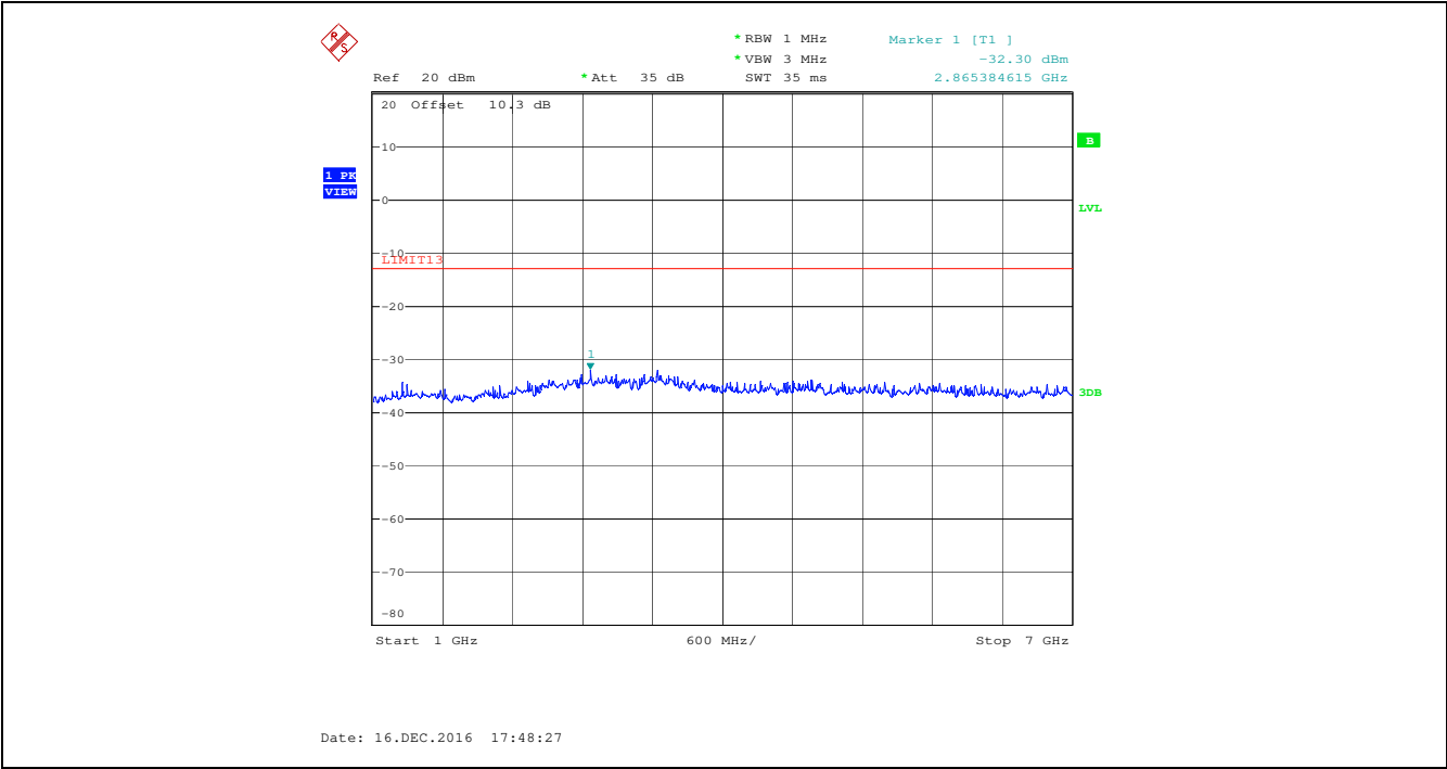
Plot 5.5.4.9. Spurious Emissions at Antenna Terminal, 510.000 MHz, High Power, Audio Input 15 kHz 1 Vrms 1 GHz - 7 GHz
