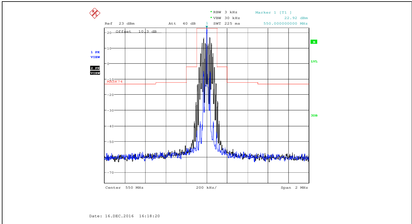
Plot 5.4.4.2.5. Emission Mask of §74.861(e)(6), 550.000 MHz, High Power, Audio input 15 kHz 1 Vrms
