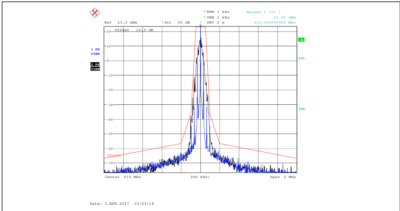
Plot 5.4.4.3.3. Emission Mask of §74.861(e)(7), 510.000 MHz, High Power Audio input maximum 1 Vrms, Noise source input level 1V band limit to 15 kHz
