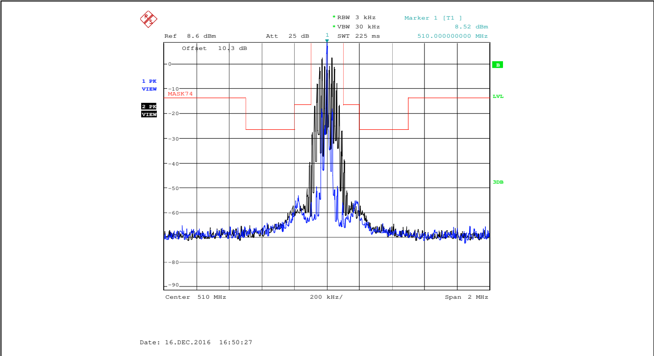
Plot 5.4.4.2.4. Emission Mask of §74.861(e)(6), 510.000 MHz, Low Power, Audio input 15 kHz 1 Vrms
