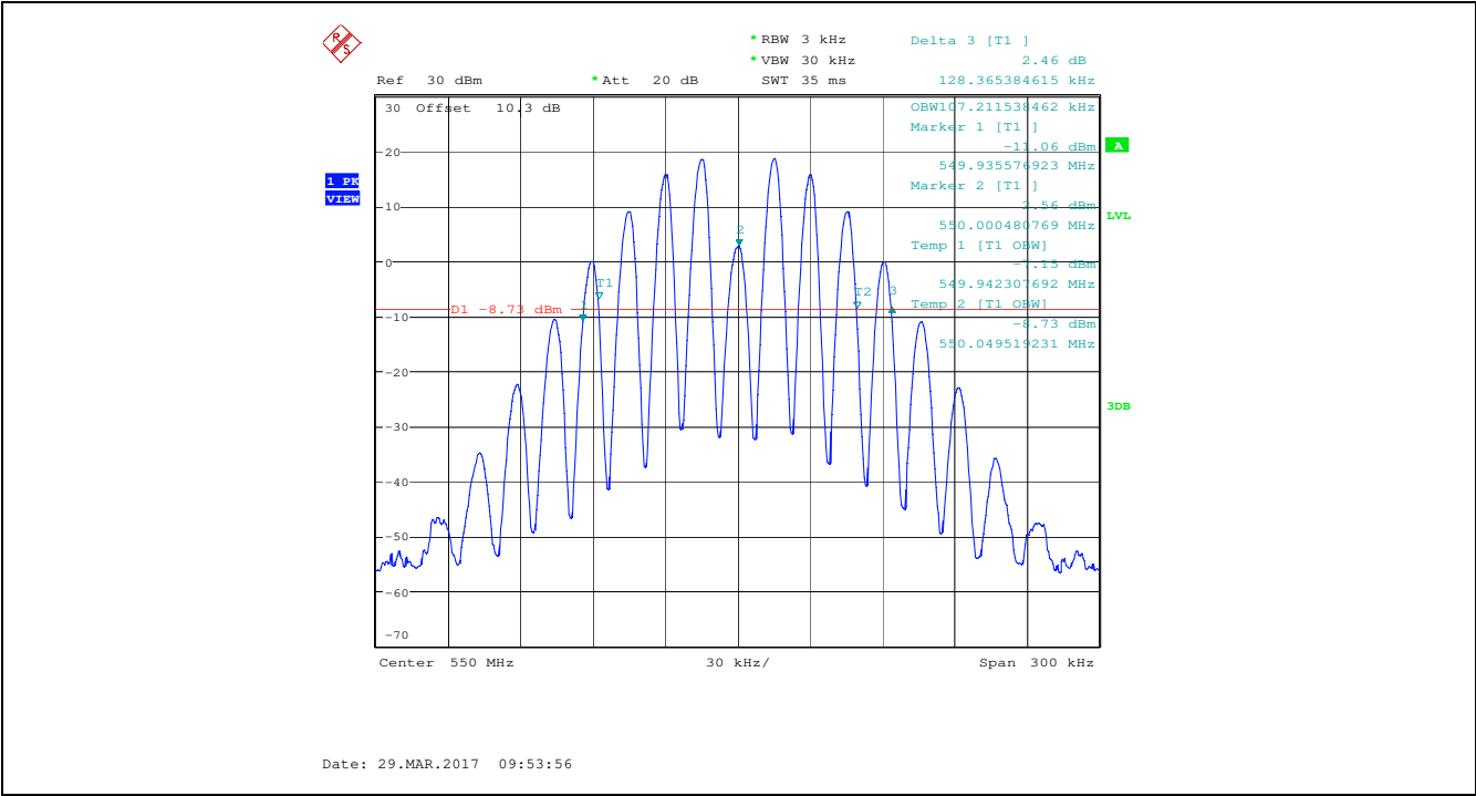
Plot 5.4.4.1.3. Occupied Bandwidth, 550.000 MHz, Audio input 15 kHz 1 Vrms, High Power
