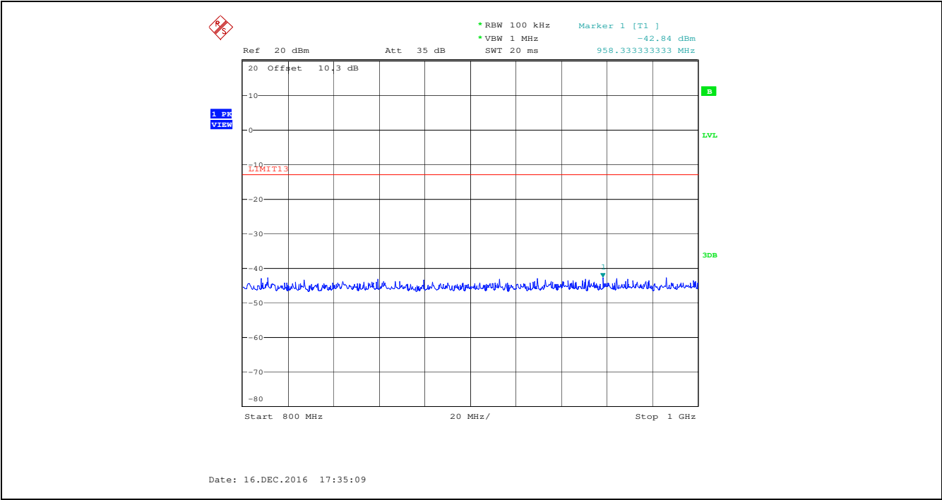
Plot 5.5.4.5. Spurious Emissions at Antenna Terminal, 470.250 MHz, Low Power, Audio Input 15 kHz 1 Vrms 800 MHz - 1 GHz
