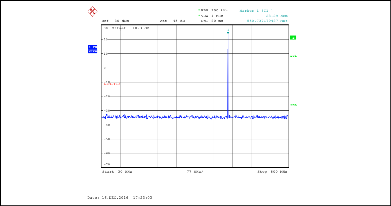
Plot 5.5.4.13. Spurious Emissions at Antenna Terminal, 550.000 MHz, High Power, Audio Input 15 kHz 1 Vrms 30 MHz - 800 MHz
