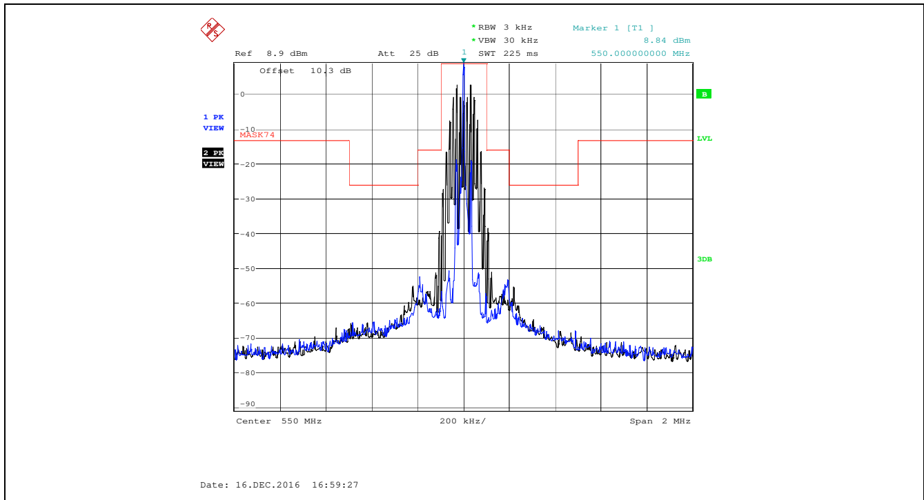
Plot 5.4.4.2.6. Emission Mask of §74.861(e)(6), 550.000 MHz, Low Power, Audio input 15 kHz 1 Vrms
