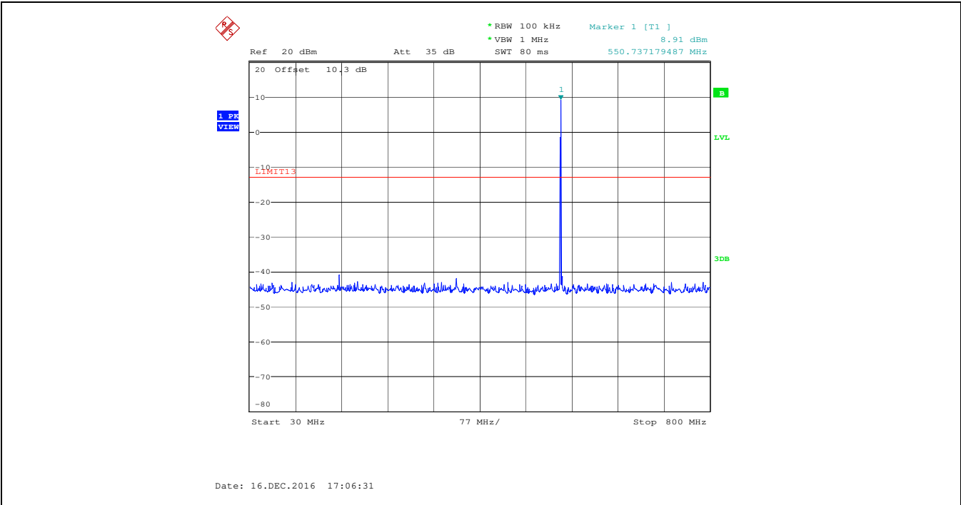
Plot 5.5.4.16. Spurious Emissions at Antenna Terminal, 550.000 MHz, Low Power, Audio Input 15 kHz 1 Vrms 30 MHz - 800 MHz
