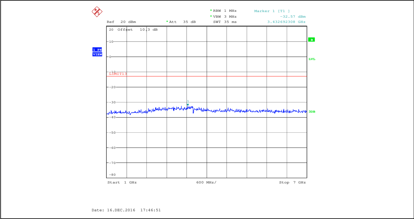
Plot 5.5.4.12. Spurious Emissions at Antenna Terminal, 510.000 MHz, Low Power, Audio Input 15 kHz 1 Vrms 1 GHz - 7 GHz
