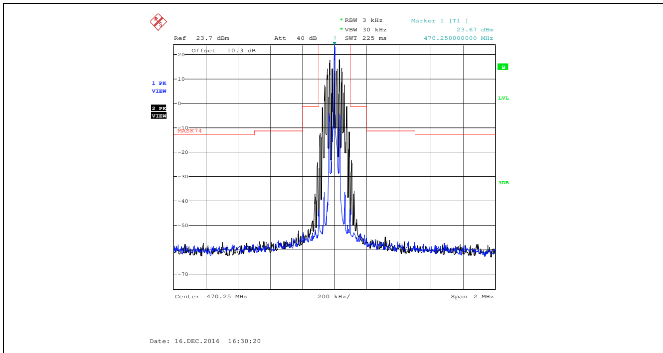
Plot 5.4.4.2.1. Emission Mask of §74.861(e)(6), 470.250 MHz, High Power, Audio input 15 kHz 1 Vrms
