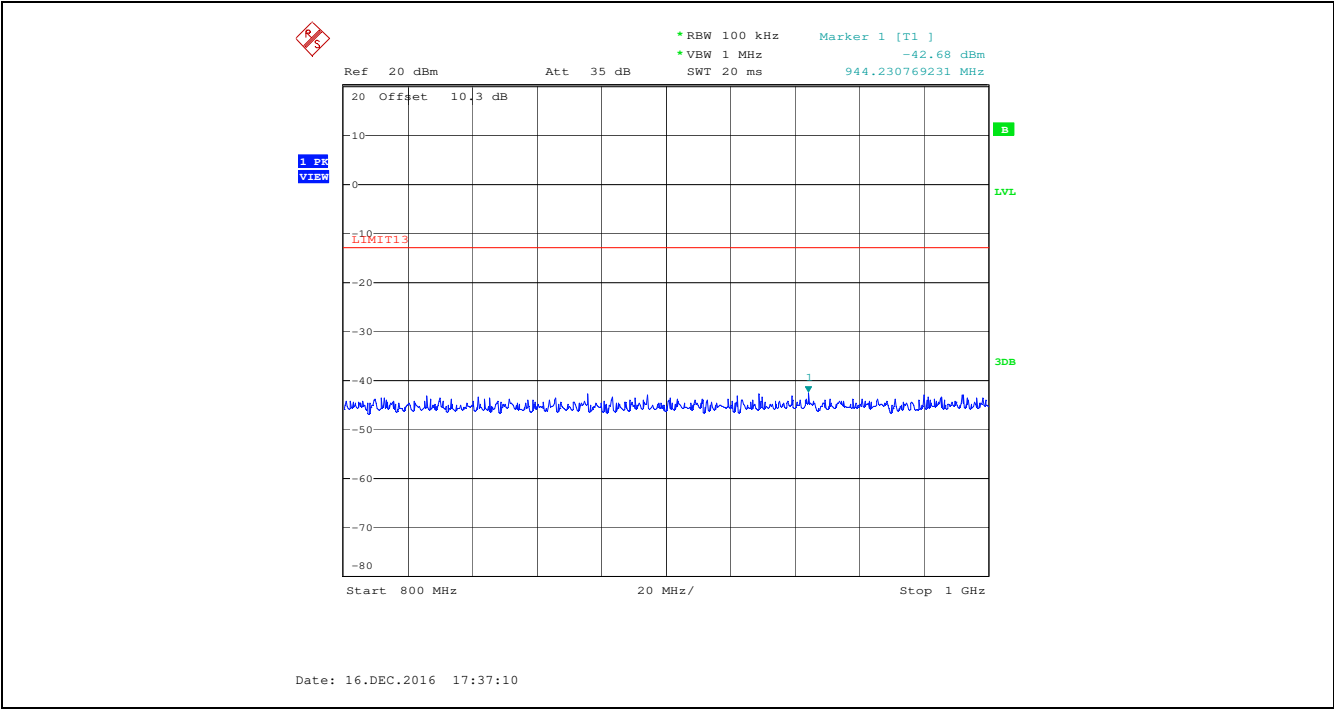
Plot 5.5.4.11. Spurious Emissions at Antenna Terminal, 510.000 MHz, Low Power, Audio Input 15 kHz 1 Vrms 800 MHz - 1 GHz
