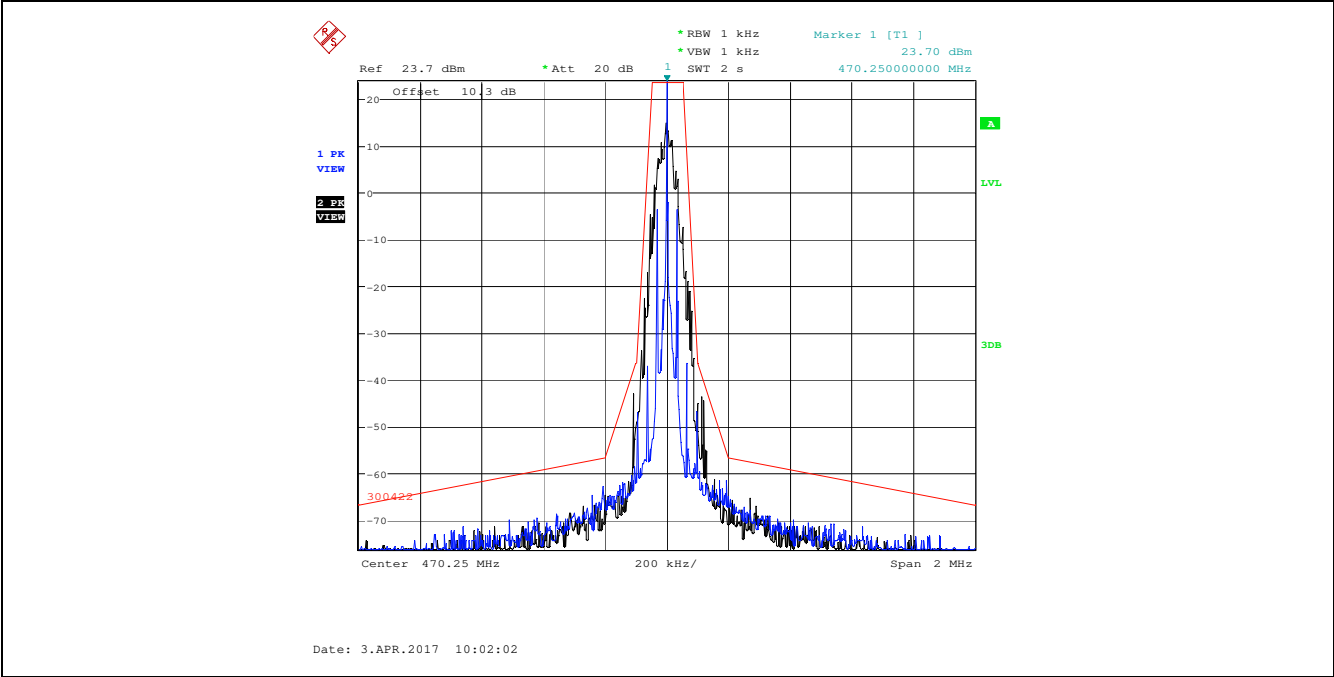
Plot 5.4.4.3.1. Emission Mask of §74.861(e)(7), 470.250 MHz, High Power Audio input maximum 1 Vrms, Noise source input level 1V band limit to 15 kHz
