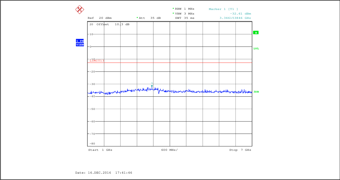
Plot 5.5.4.18. Spurious Emissions at Antenna Terminal, 550.000 MHz, Low Power, Audio Input 15 kHz 1 Vrms 1 GHz - 7 GHz
