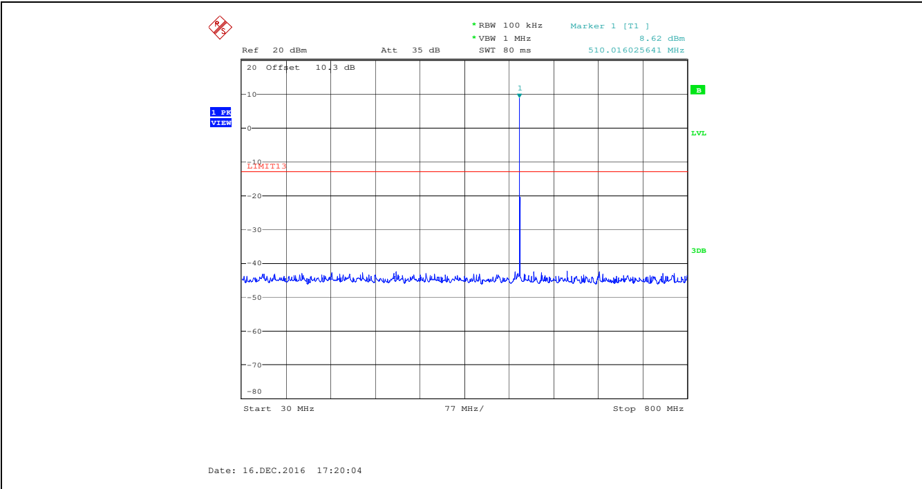
Plot 5.5.4.10. Spurious Emissions at Antenna Terminal, 510.000 MHz, Low Power, Audio Input 15 kHz 1 Vrms 30 MHz - 800 MHz
