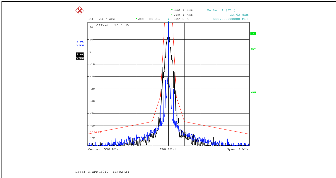
Plot 5.4.4.3.5. Emission Mask of §74.861(e)(7), 550.000 MHz, High Power Audio input maximum 1 Vrms, Noise source input level 1V band limit to 15 kHz
